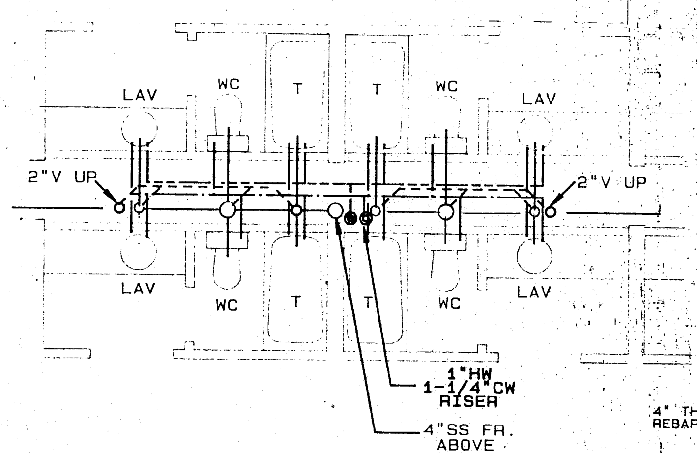
TYPICAL 1st FLR. KING & DOUBLE BACK-BACK SUITES
