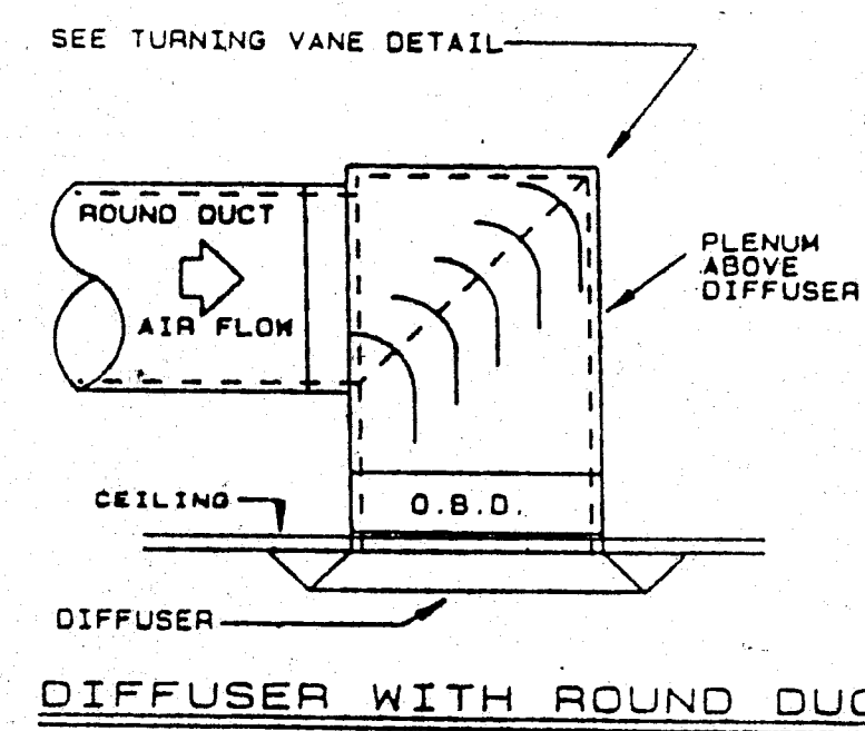
DIFFUSER WITH ROUND DUCT
