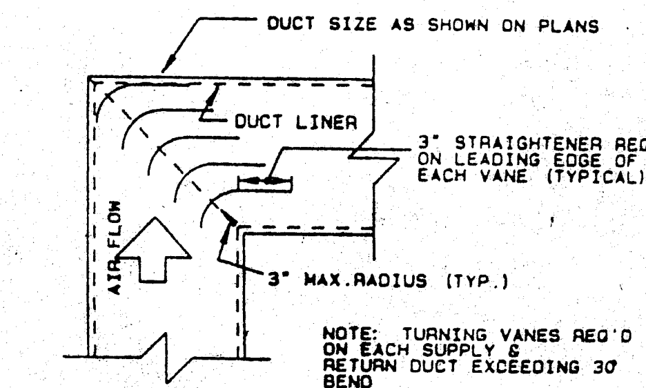
TURNING VANE DETAIL
