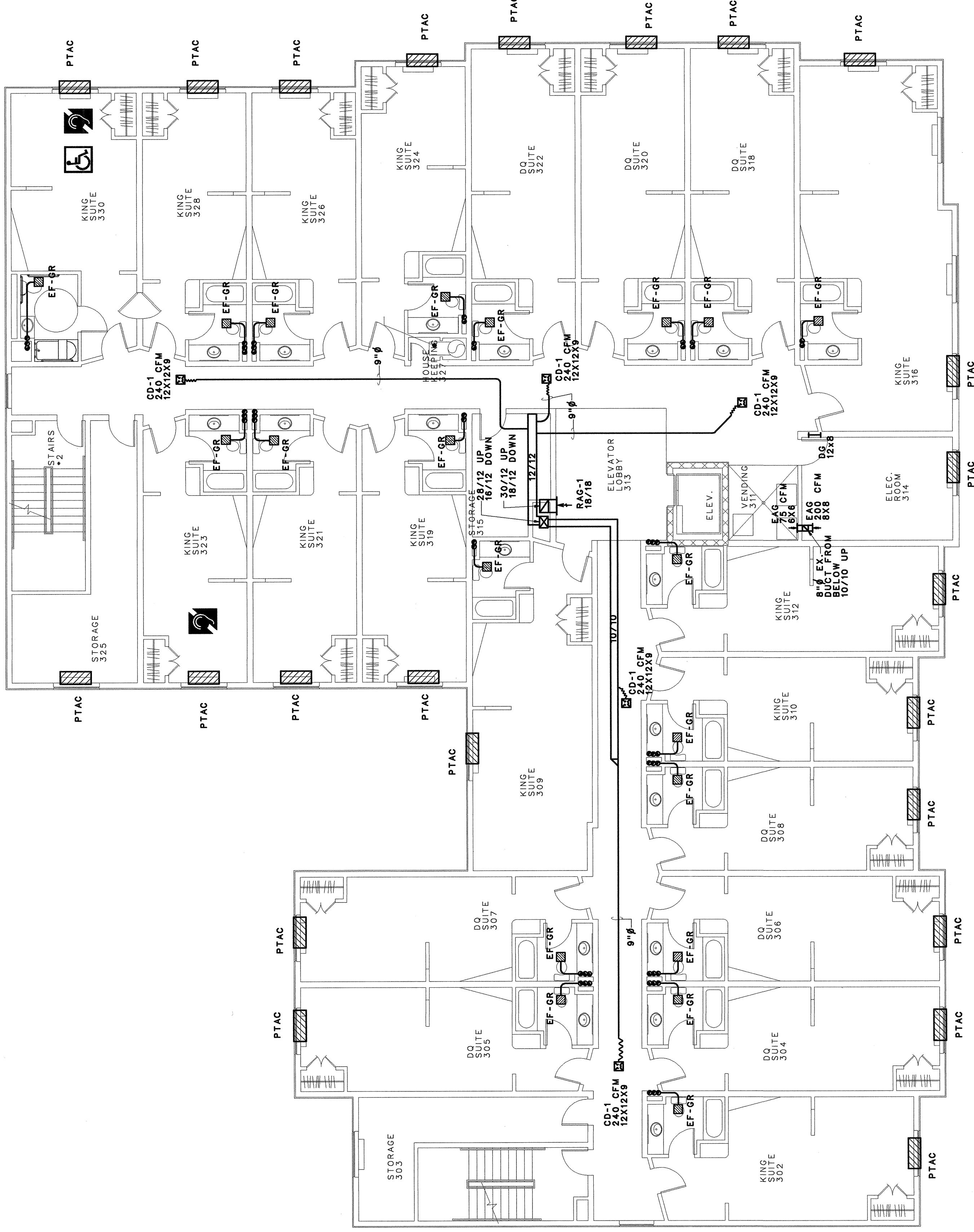
HVAC PLAN - THIRD FLOOR
