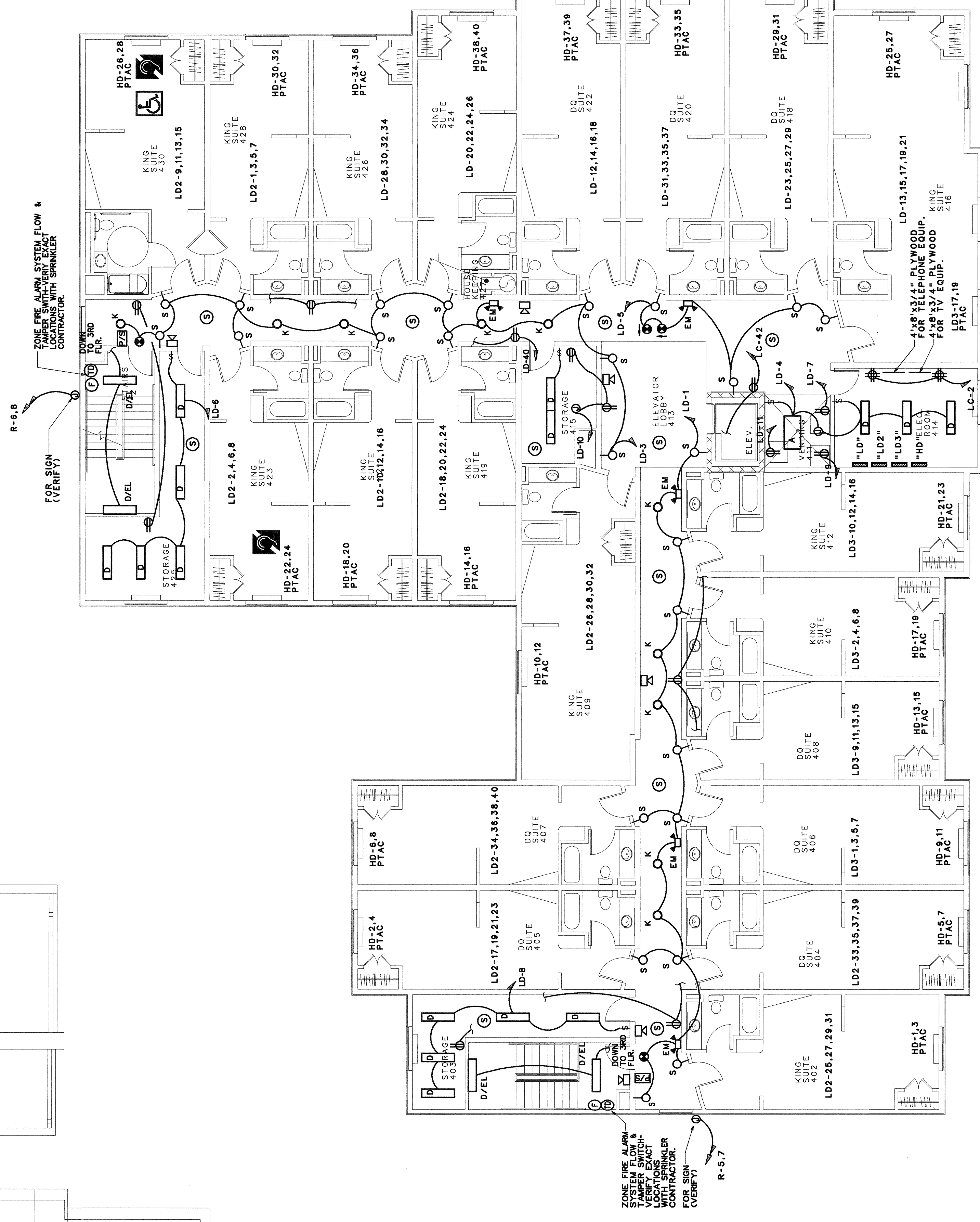
ELECTRICAL PLAN - FOURTH FLOOR
