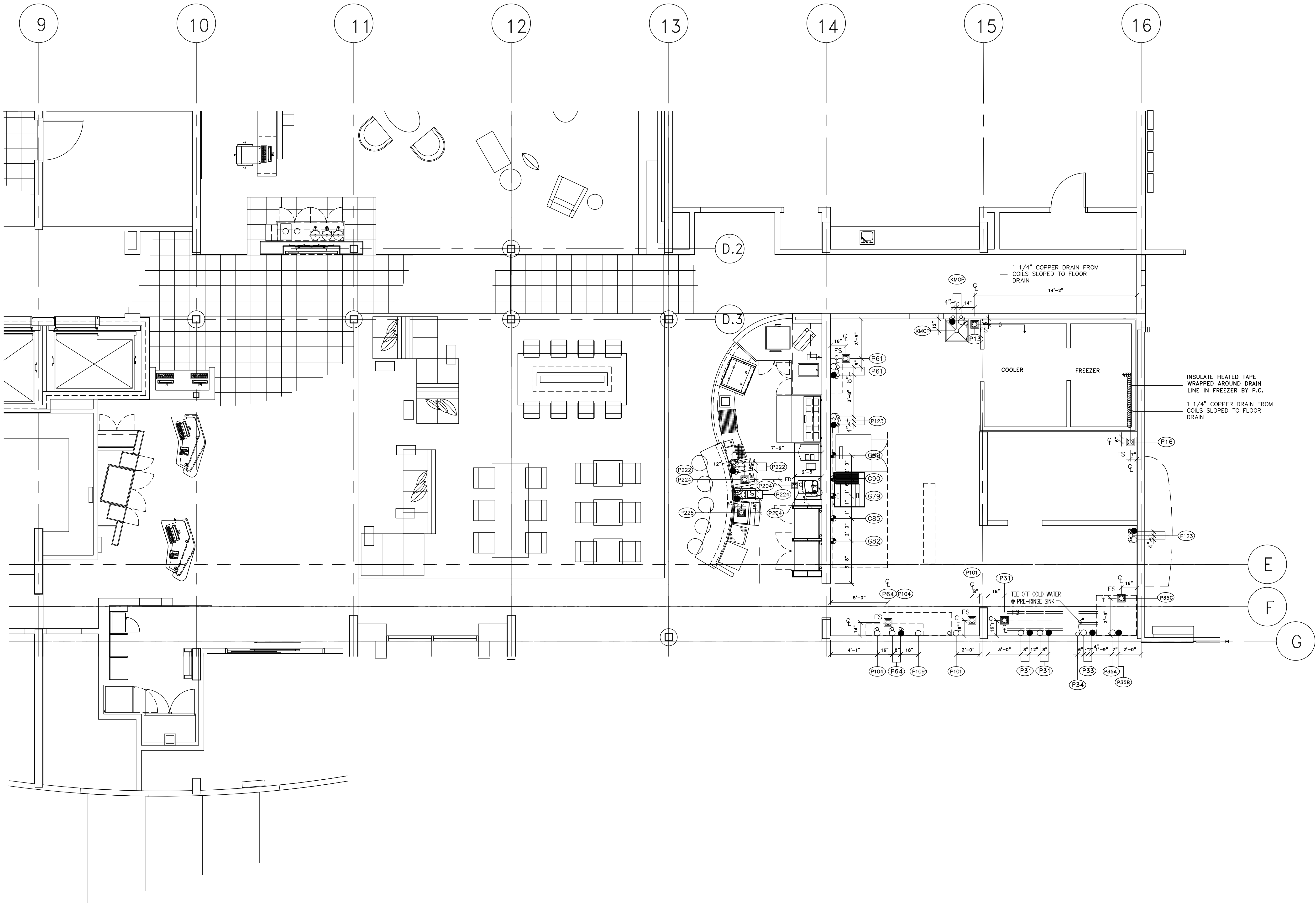
PLUMBING ROUGH-IN PLAN SCALE: 1/4"=1'-0"
