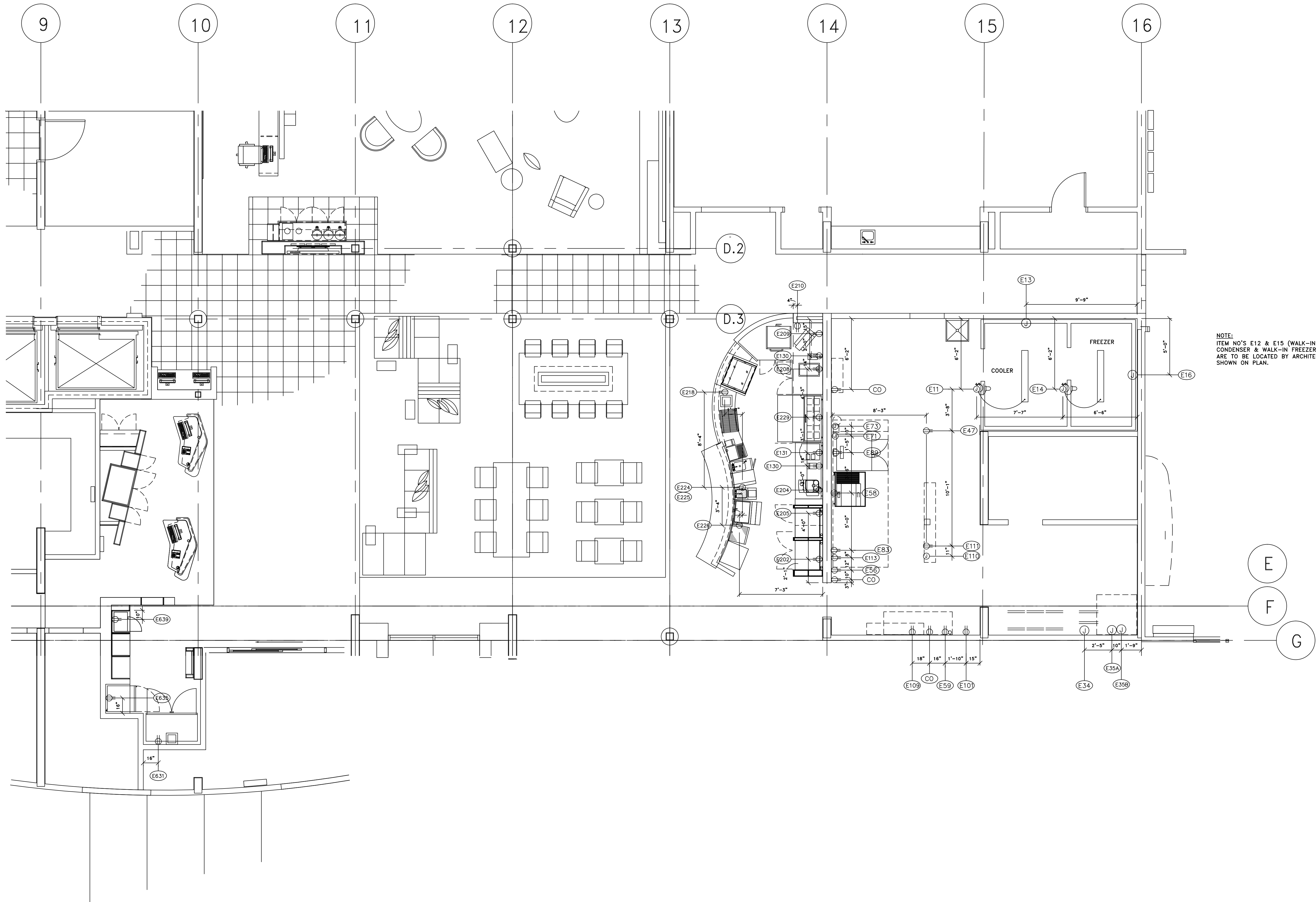
ELECTRICAL ROUGH-IN PLAN SCALE: 1/4"=1'-0"
