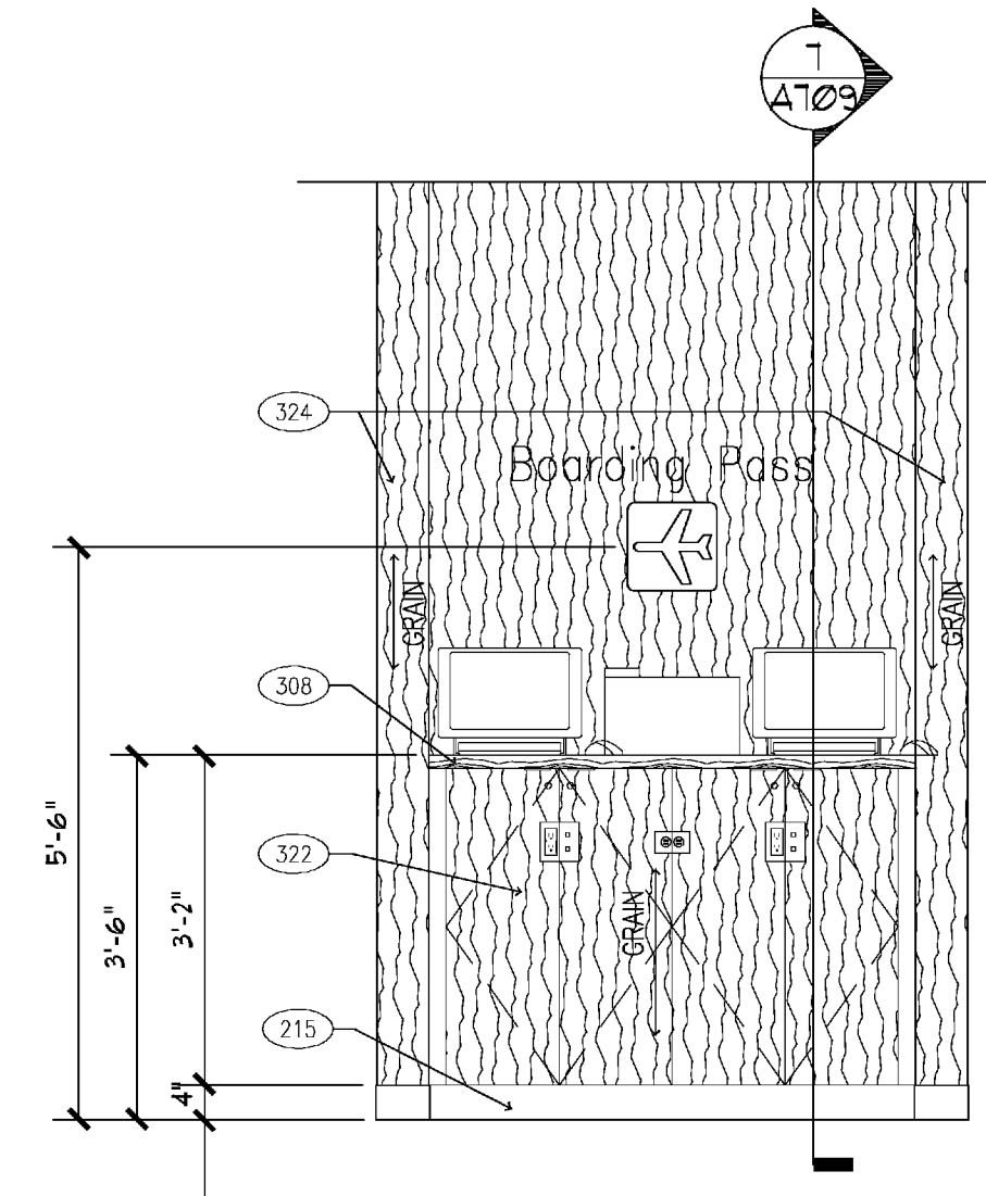
3 ELEVATION-QUICK PRINT
