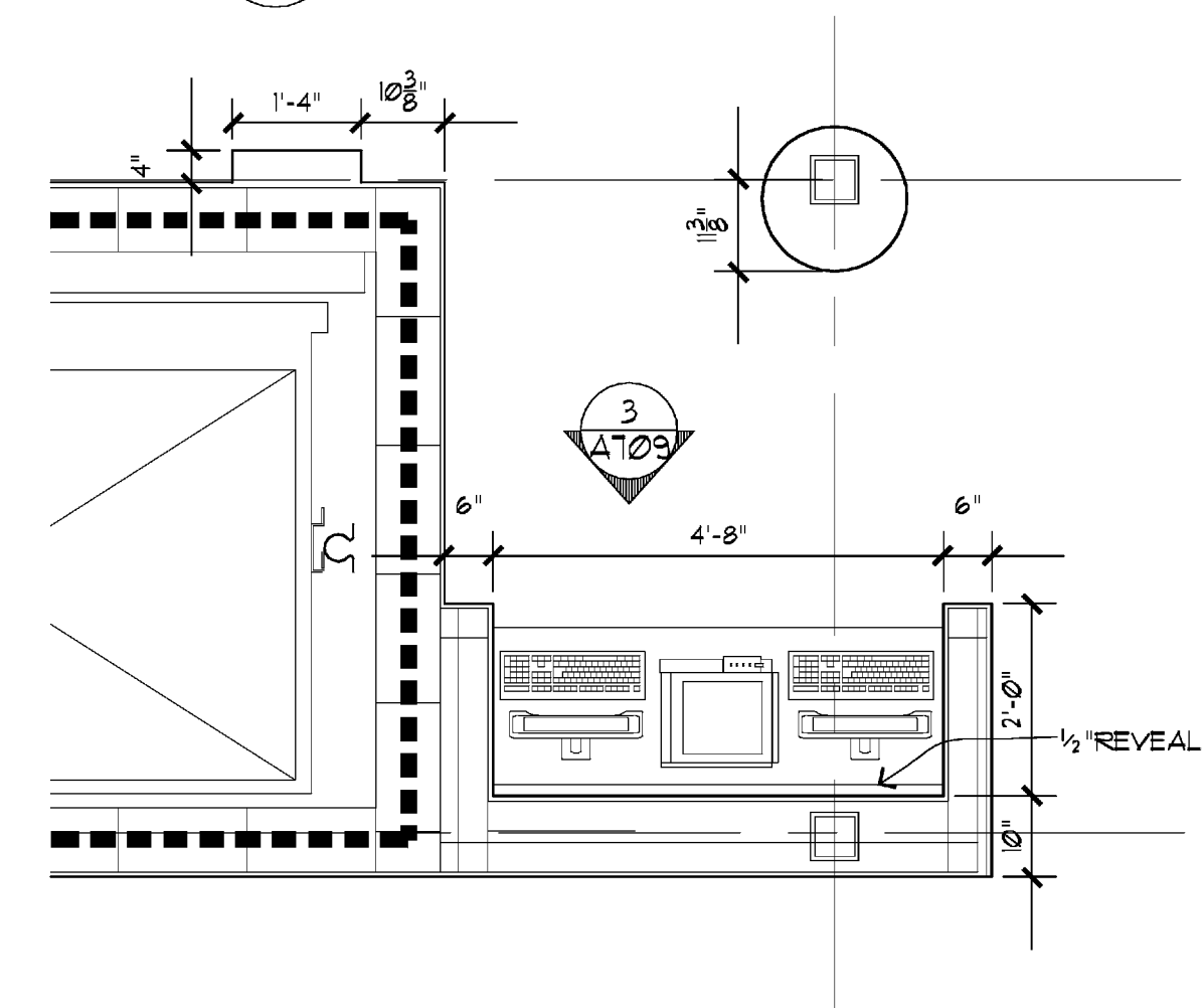
2 PLAN-CONDIMENT CENTER
