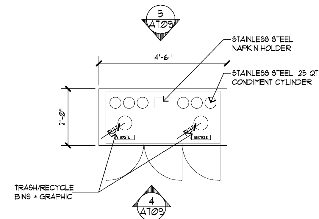
2 PLAN-CONDIMENT CENTER
