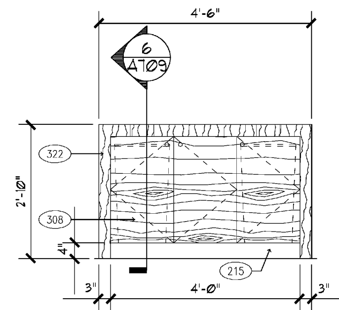
4 ELEVATION-CONDIMENT CENTER
