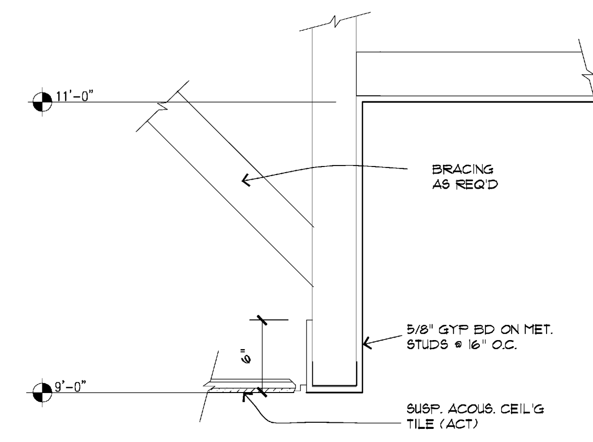
6 CEILING DETAIL
