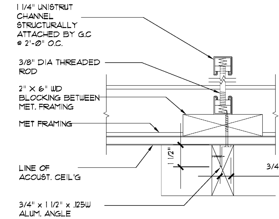
1 CEILING DETAIL
