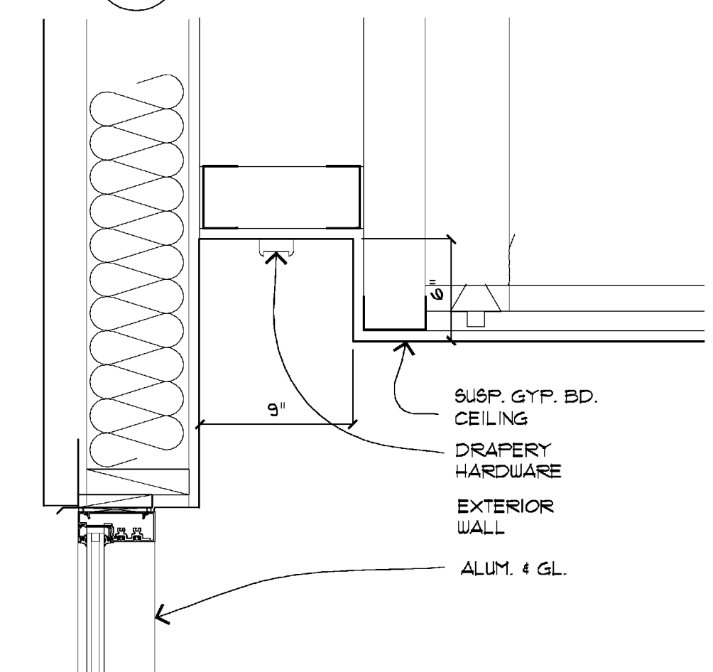
10 CEILING DETAIL
