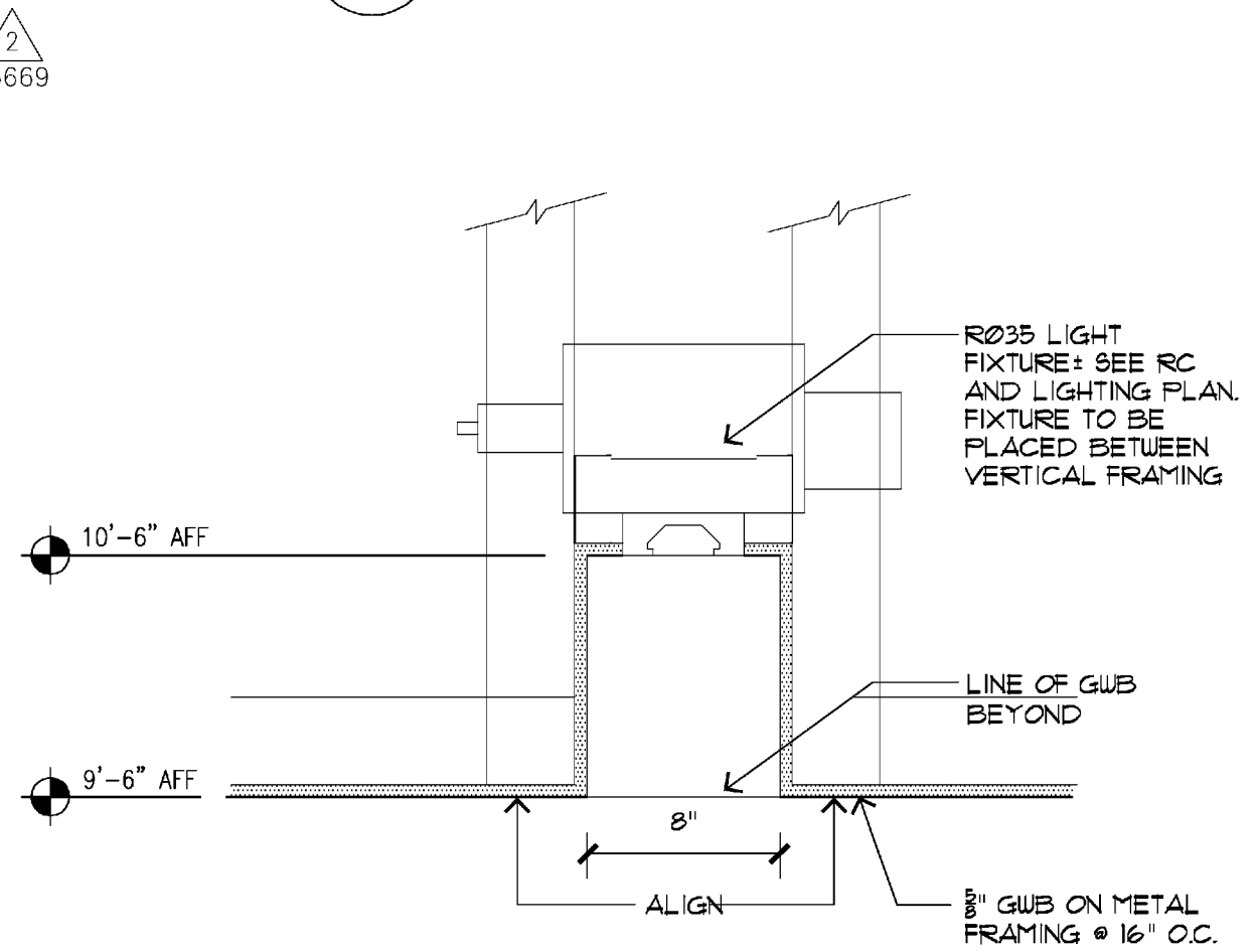
14 CEILING DETAIL
