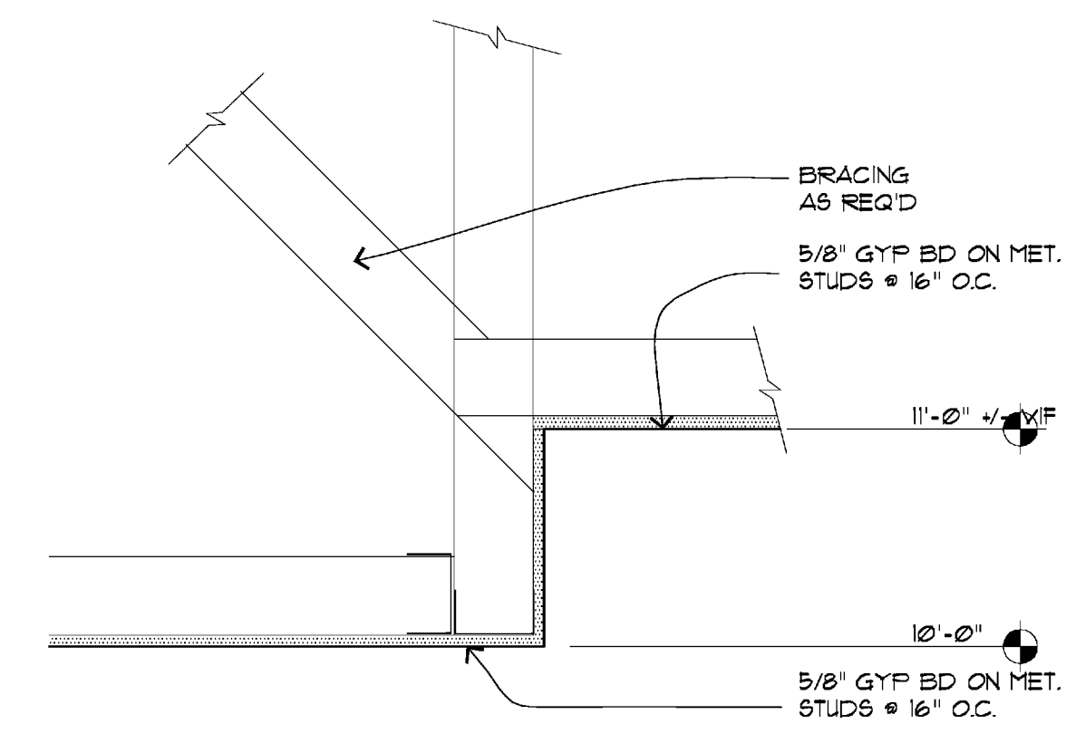
2 CEILING DETAIL
