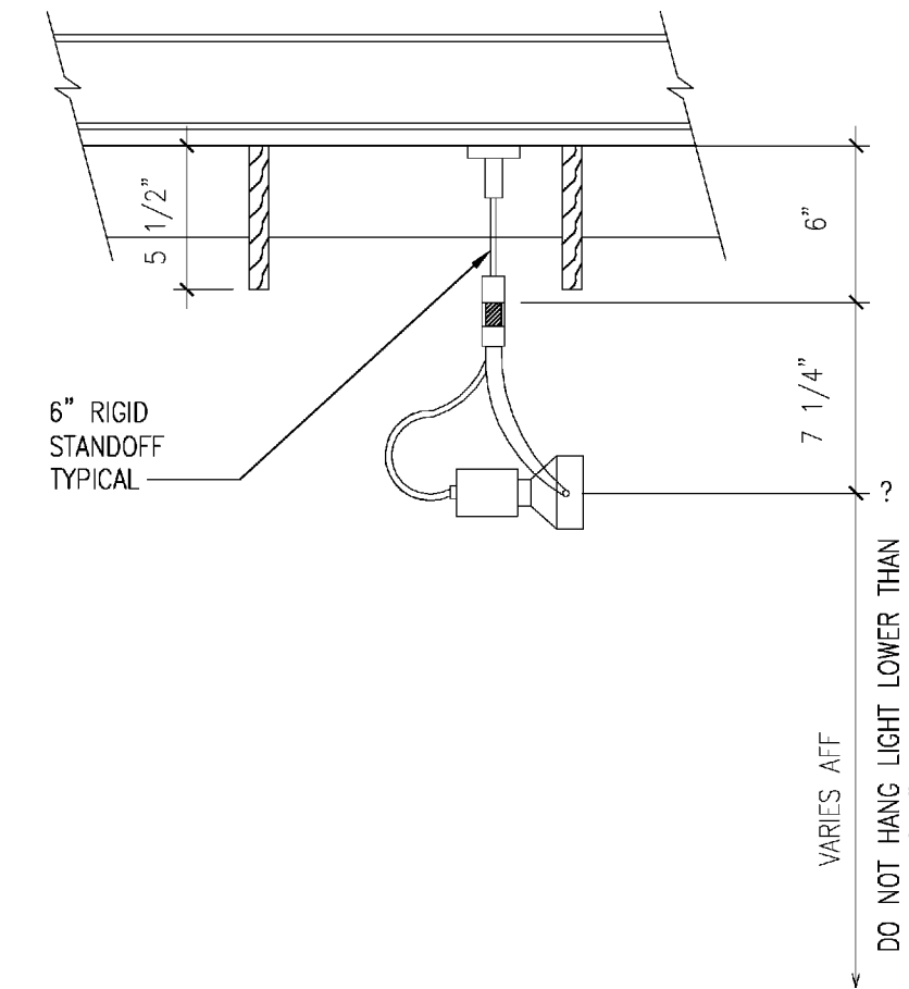
12 LIGHT DETAIL
