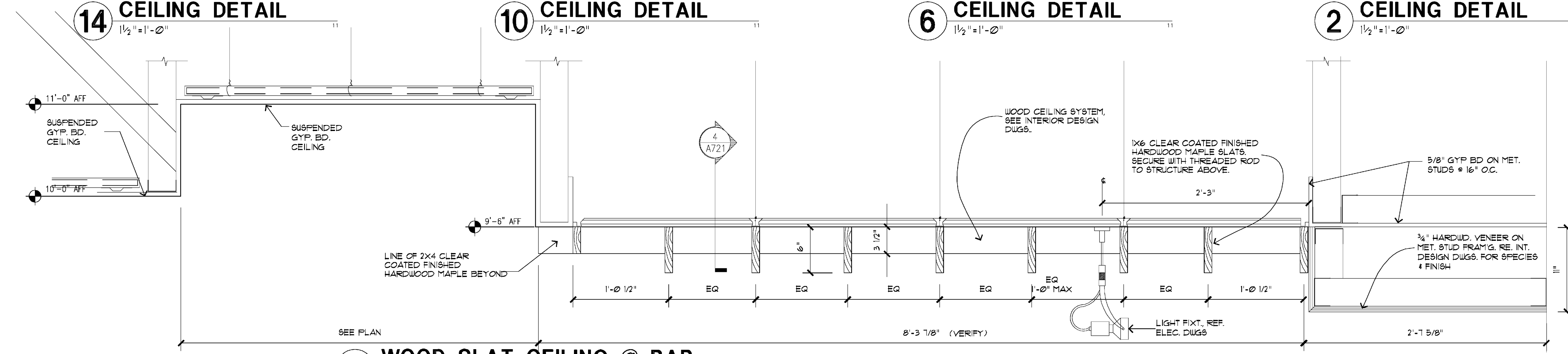
1 WOOD SLAT CEILING @ BAR
