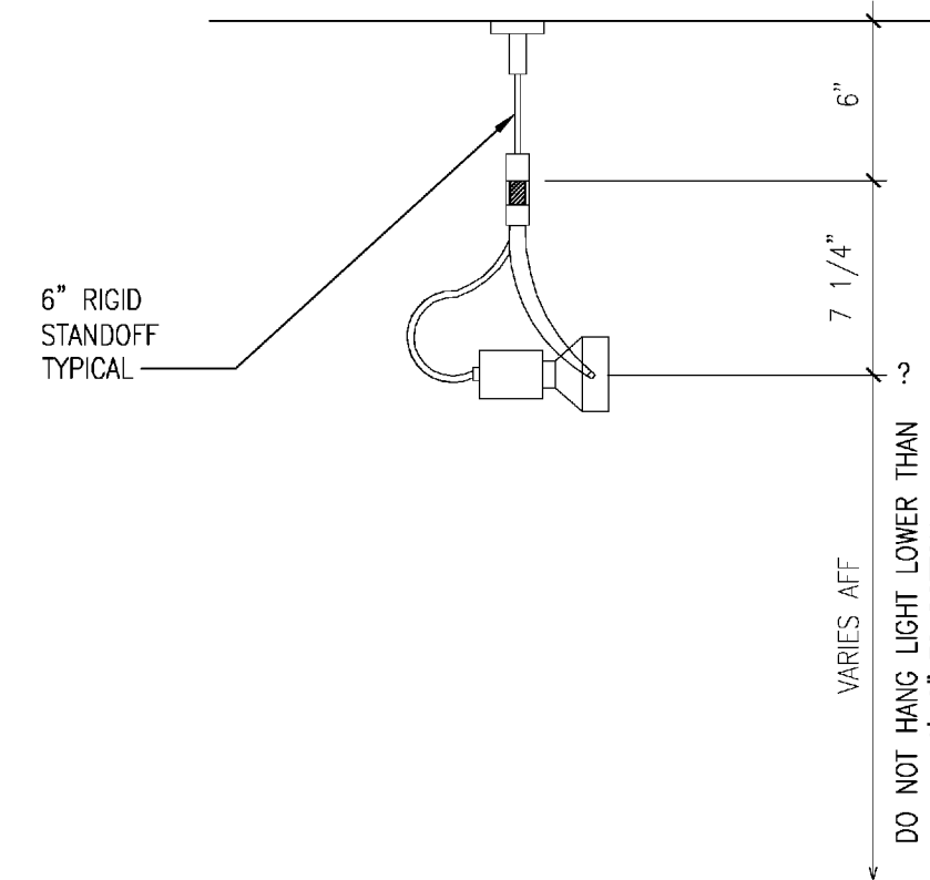
8 LIGHT DETAIL
