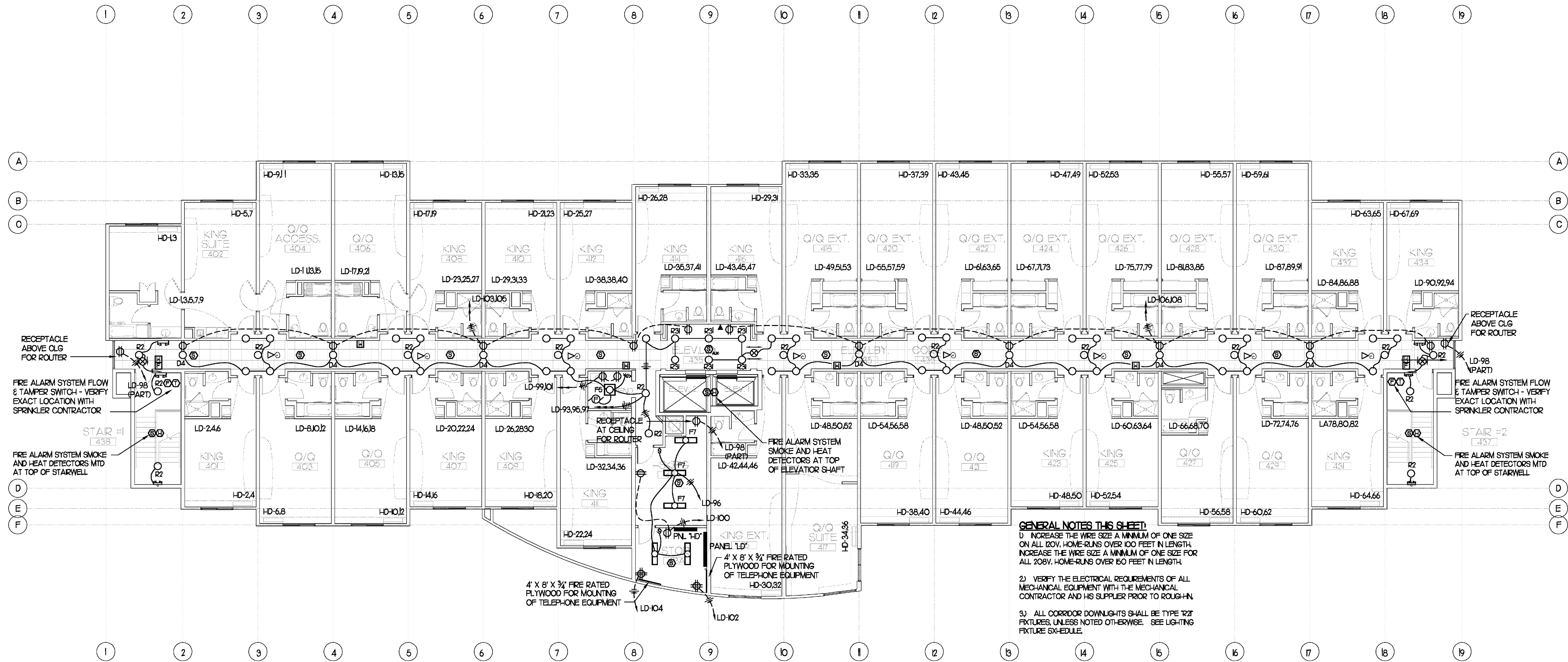
FOURTH FLOOR ELECTRICAL PLAN SCALE: 1/8" = 1'-0"
