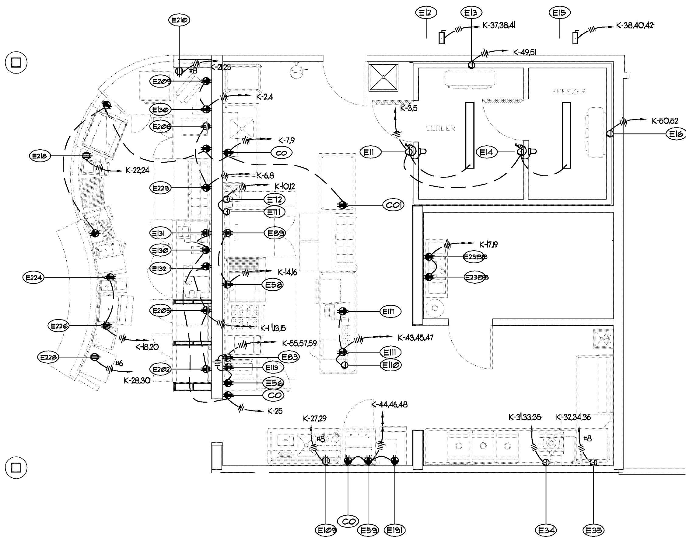
KITCHEN & BAR POWER PLAN SCALE: 1/4" = 1'-0"
