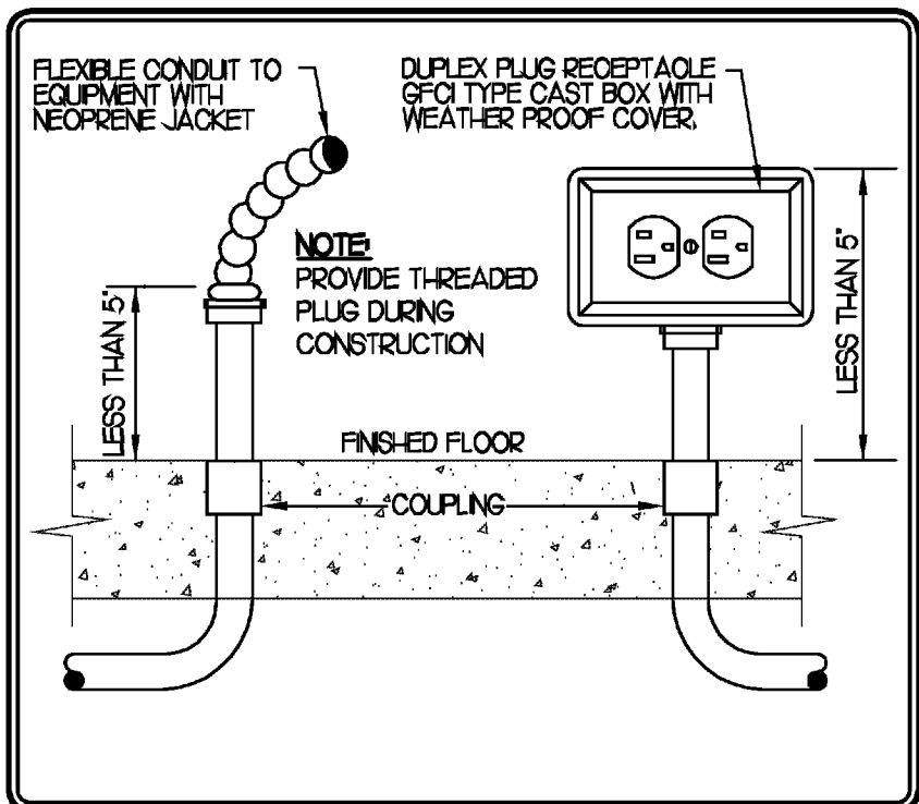
CONDUIT STUB-UP & RECEPTACLE DETAIL NO SCALE
