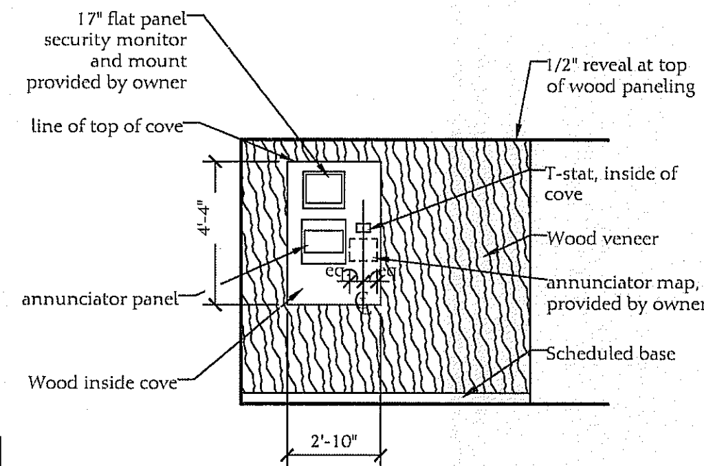
14 Elevation - Annunciator Panel
