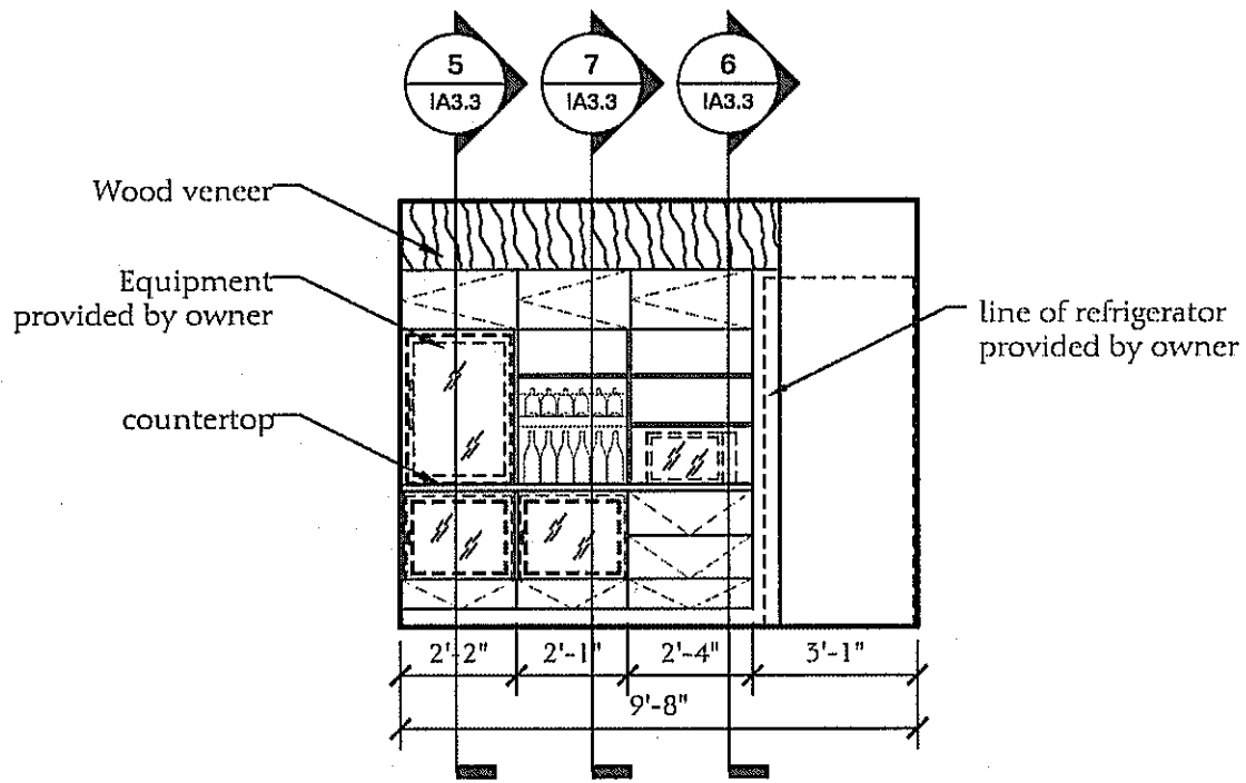
04 Elevation - The Market
