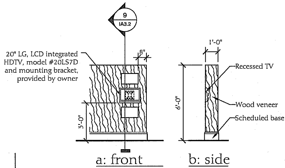
11 Elevation - Cafe Window Lounge TV's
