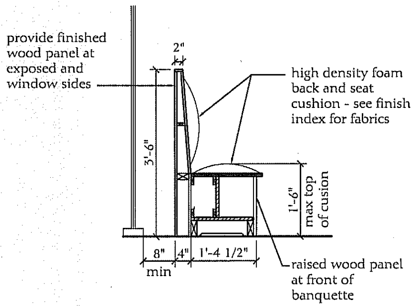
02 Detail - Media Booth Banquette
