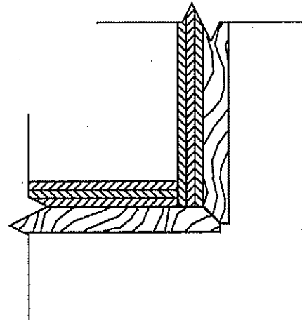
05 Detail - Typical Wall Panel Corner
