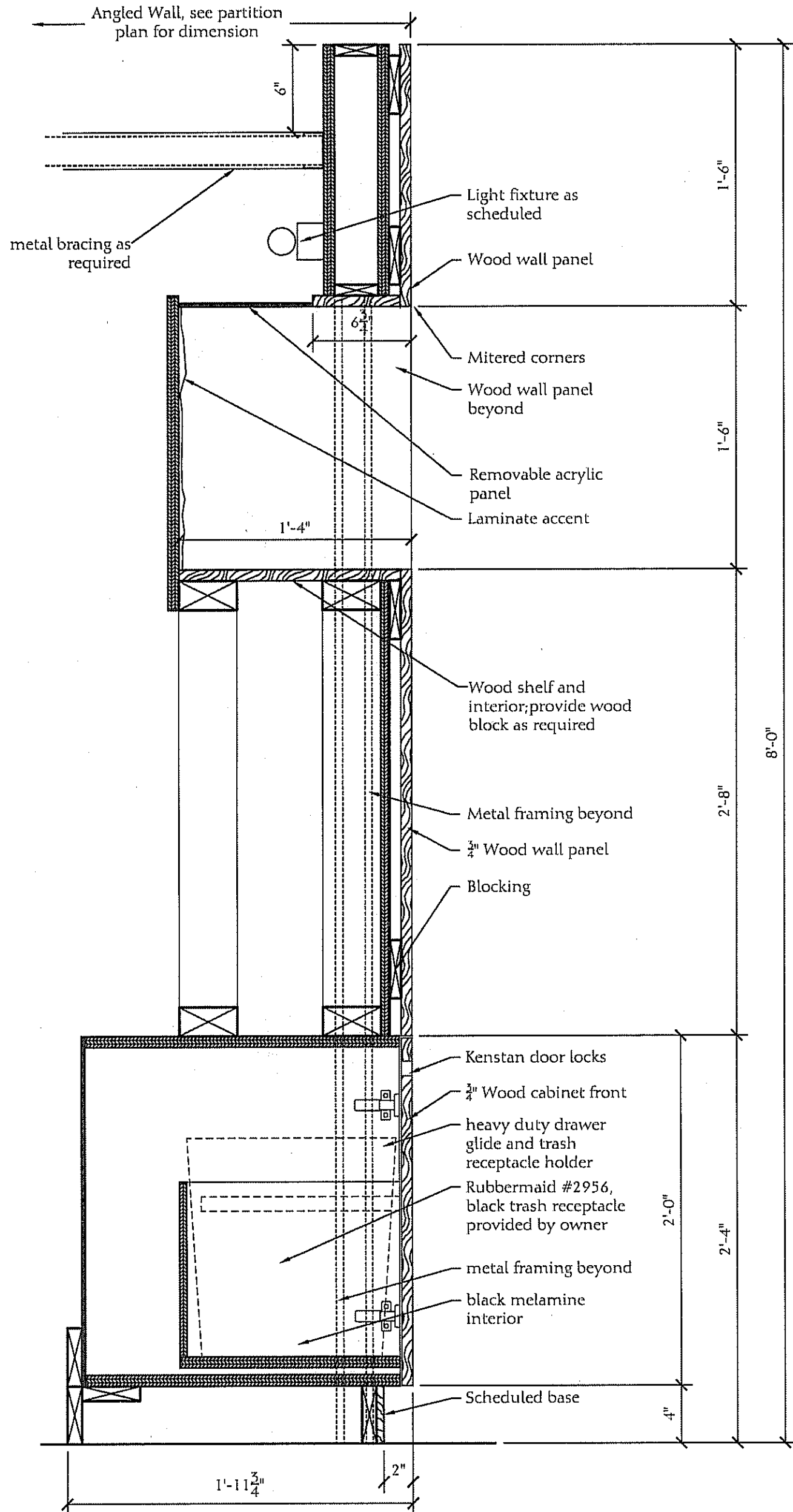
20 Detail - Check-In Wall Trash
