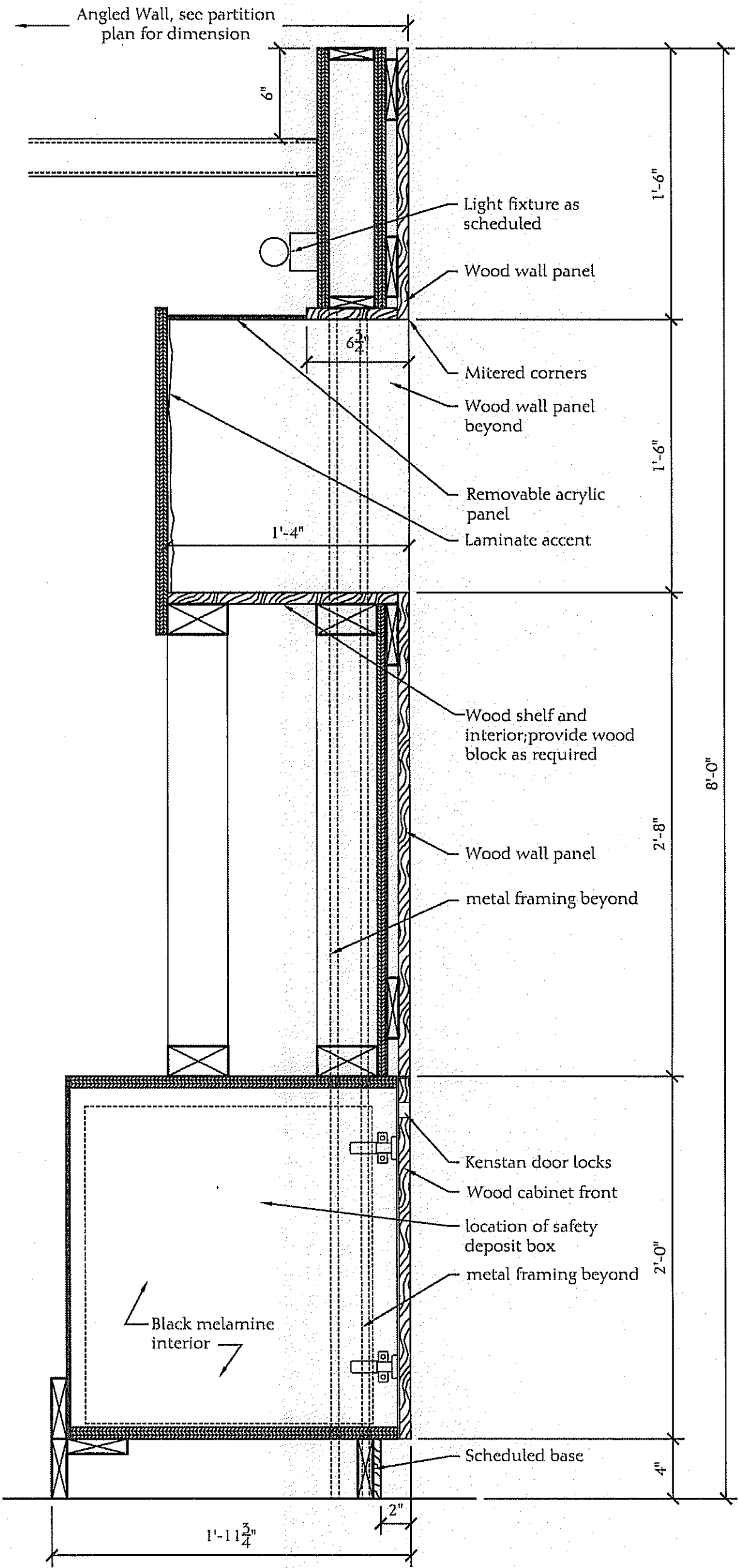
19 Detail - Check-In Wall Cabinet
