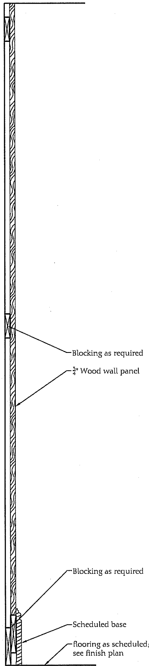
18 Detail - Typical Wood Wall
