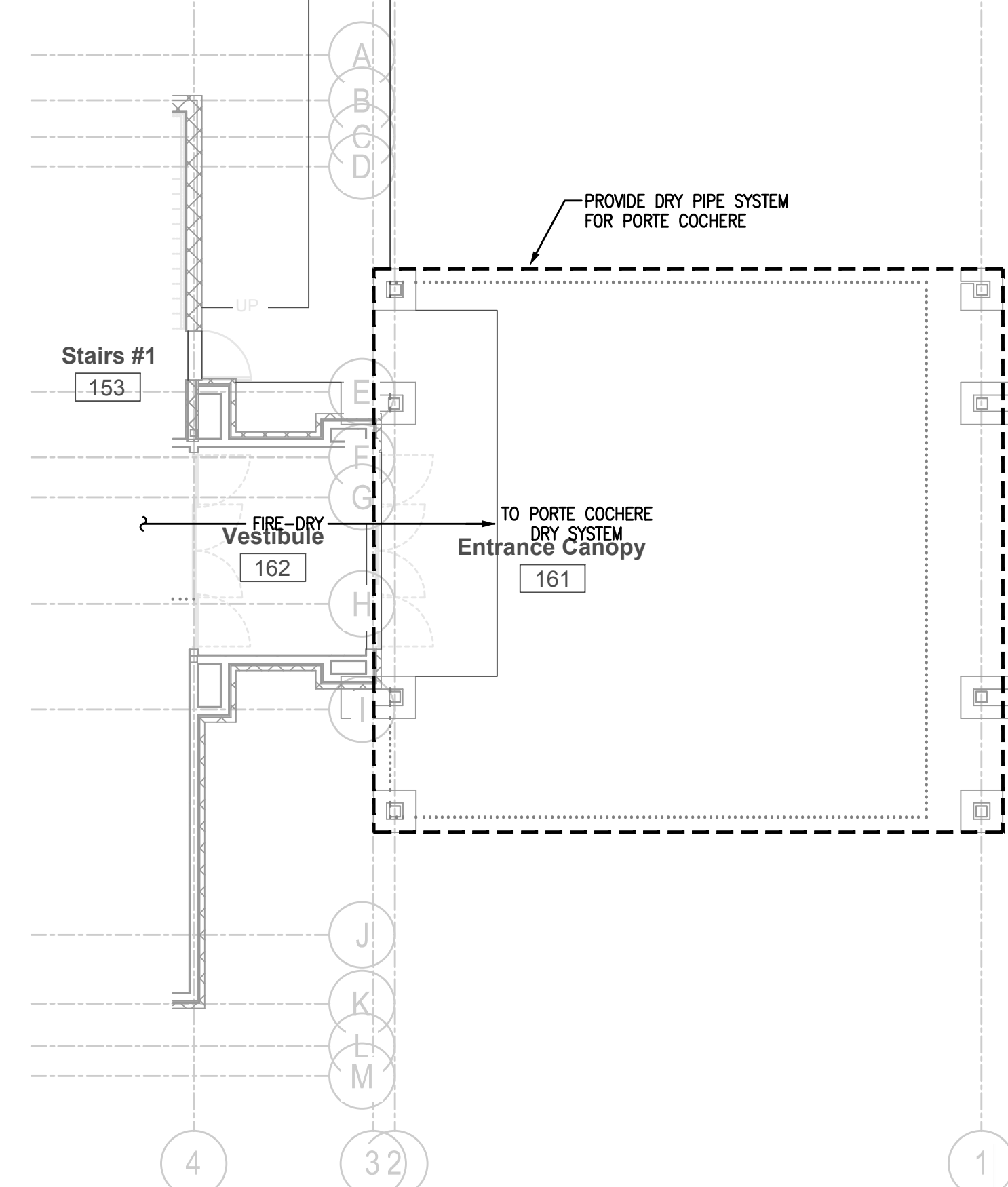
2 PARTIAL FIRST FLOOR PLAN - FIRE PROTECTION FP101 SCALE: 1/8" = 1'-0" 2 1/2" FEMALE CONNECTIONS WITH CAP AND CHAIN(S).
