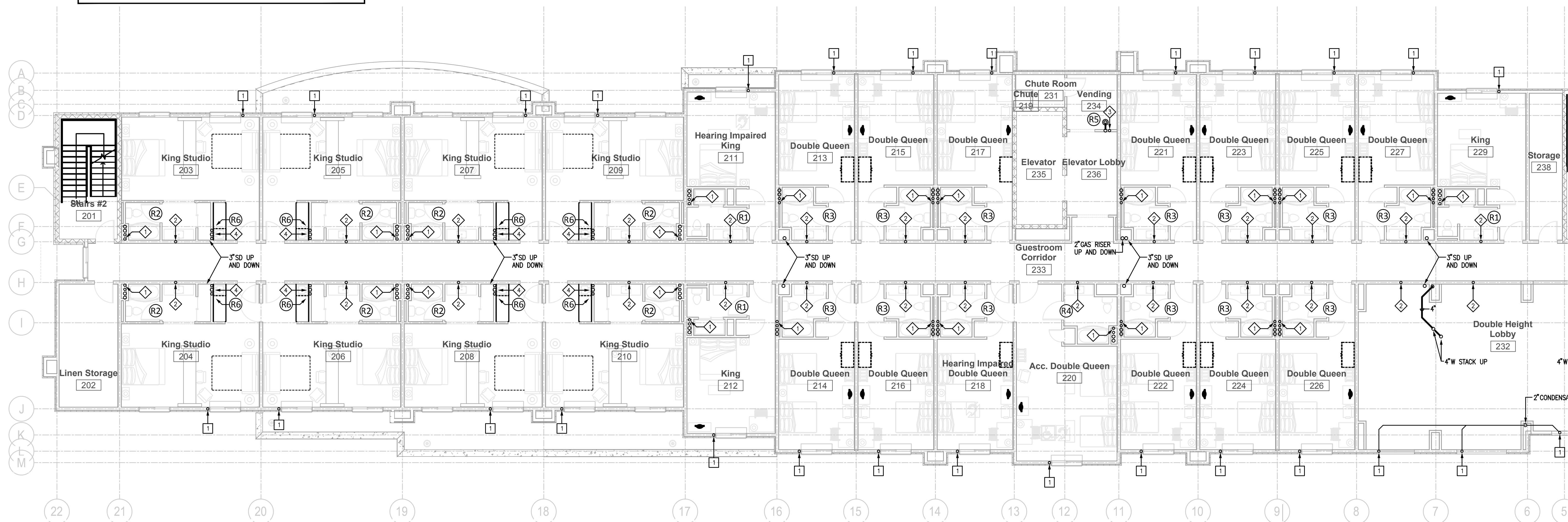
1 SECOND FLOOR PLAN - PLUMBING SCALE: 1/8" = 1'-0"
