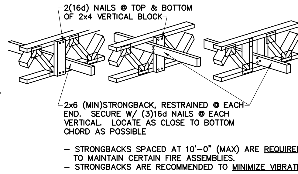
3 STRONGBACK DETAILS S401 NO SCALE
