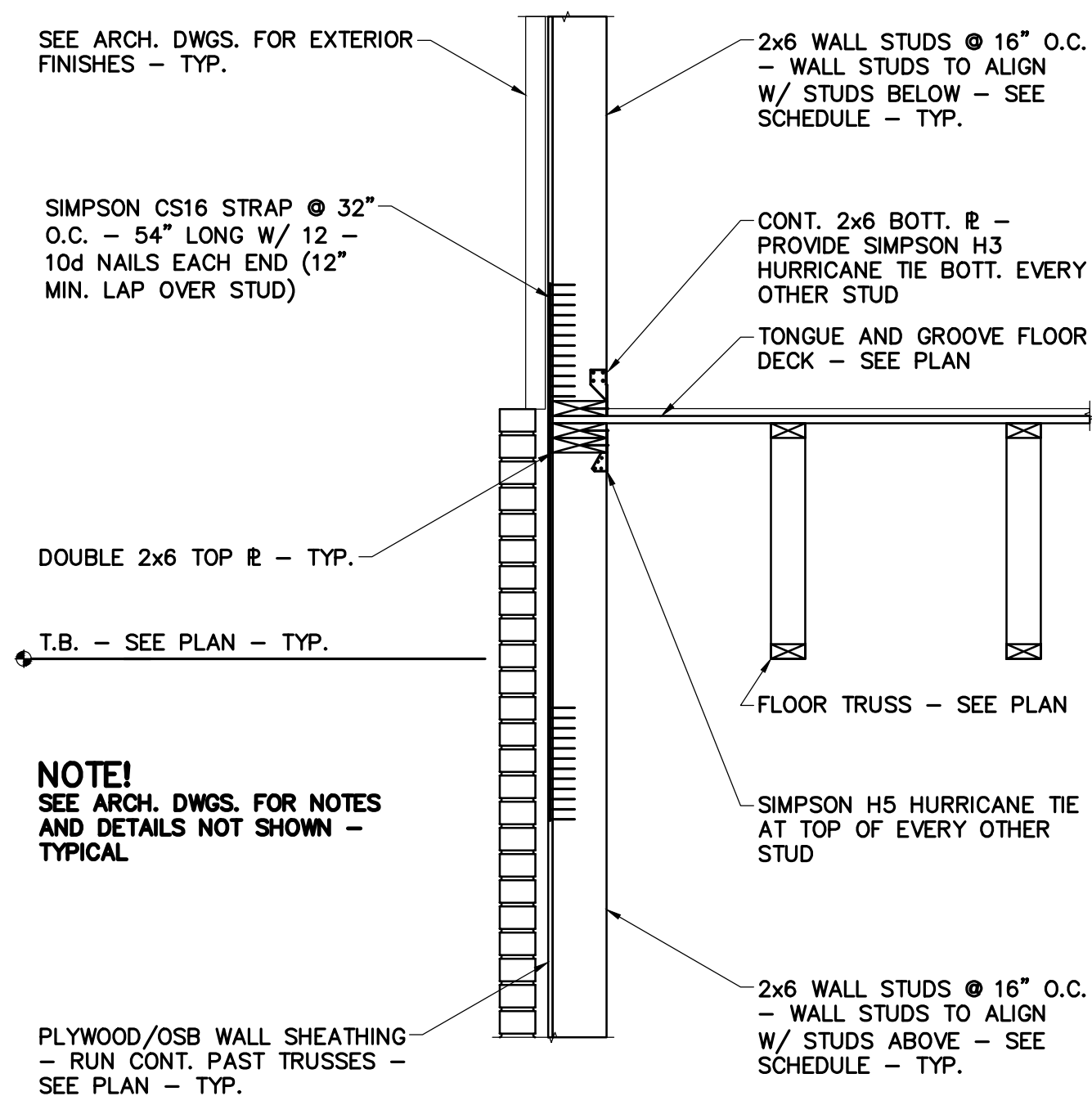
6 SECTION AT FLOOR S401 3/4" = 1'-0"
