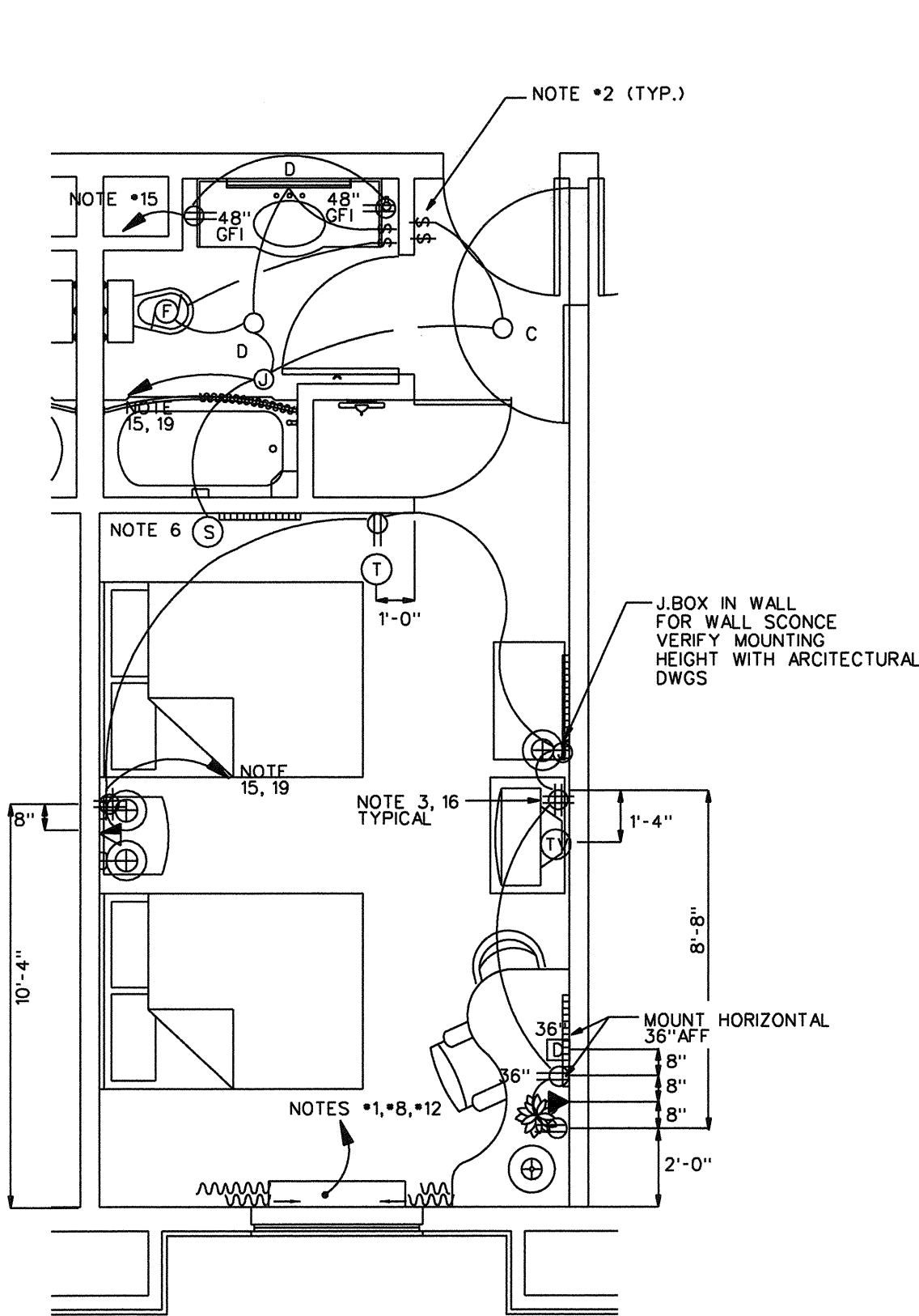
TYP. DOUBLE QUEEN SCALE: 1/4" = 1'-0"
