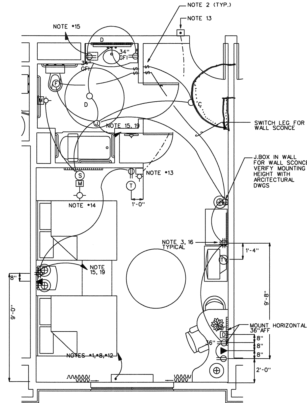
ACCESSIBLE DOUBLE QUEEN SCALE: 1/4" = 1'-0"
