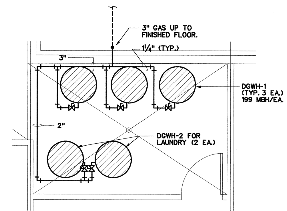
ENLARGED WATER HEATER RM. SCALE: 1/4"=1'-0"
