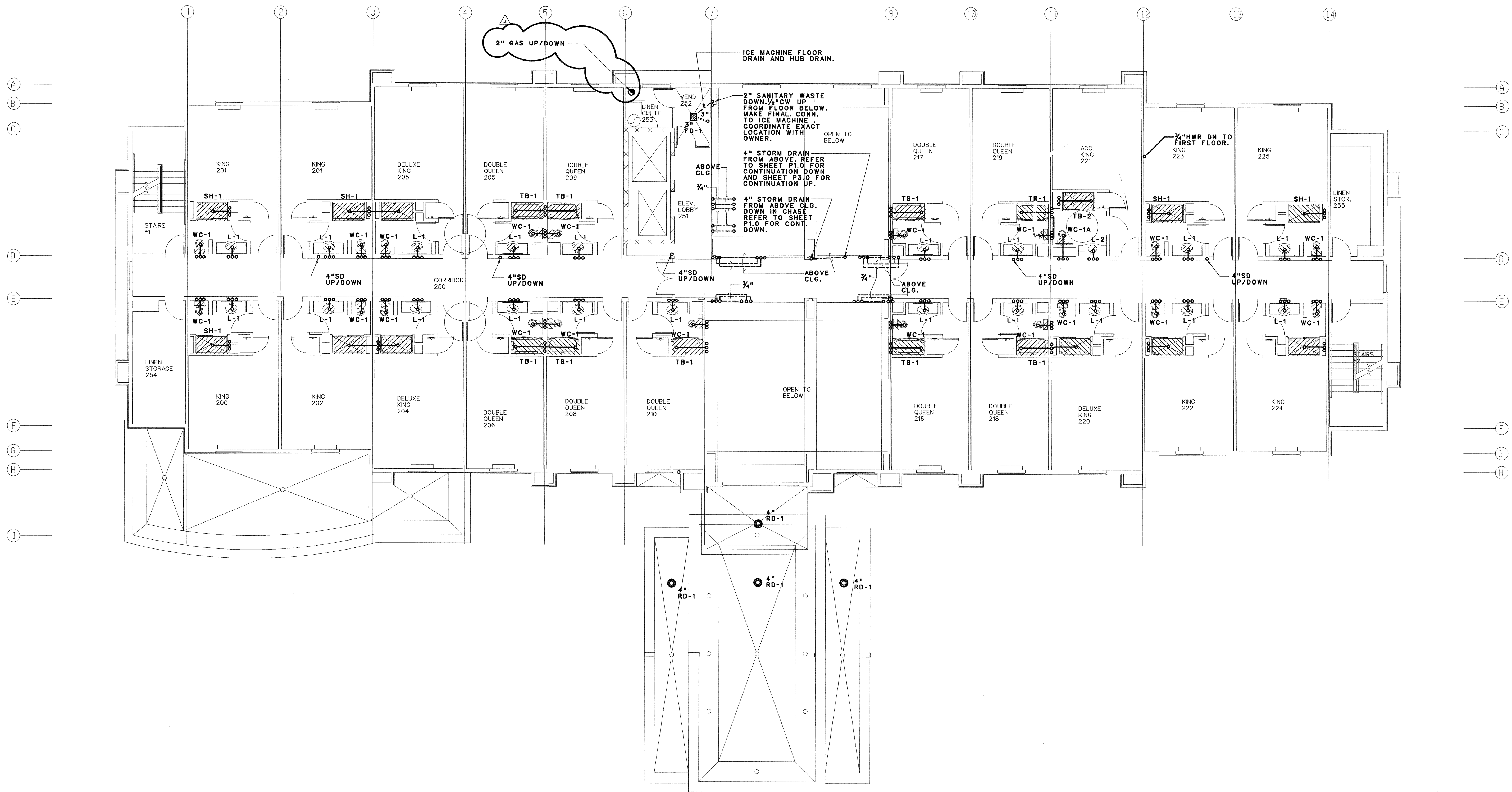
PLUMBING PLAN - SECOND FLOOR SCALE: 1/4" = 1'-0"
