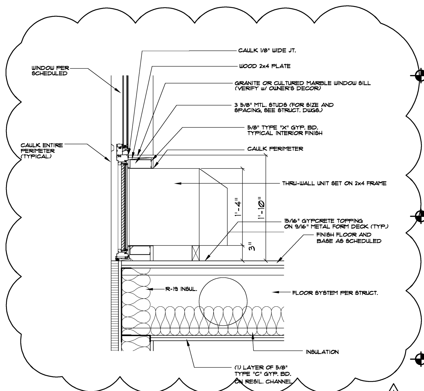
3 WINDOW SILL DETAIL 1" = 1'-0"
