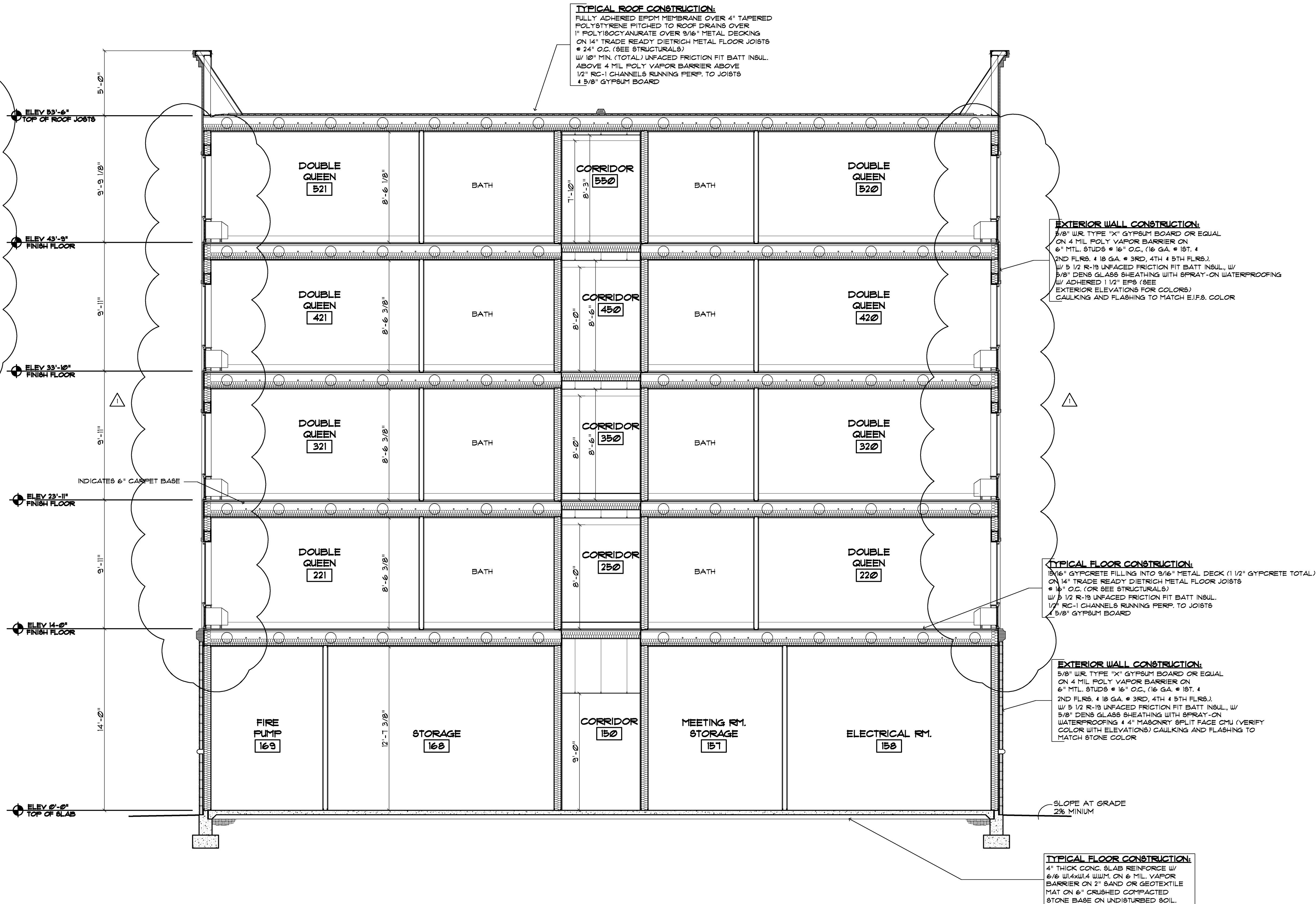
1 TYPICAL TRANSVERSE SECTION 1/4" = 1'-0"
