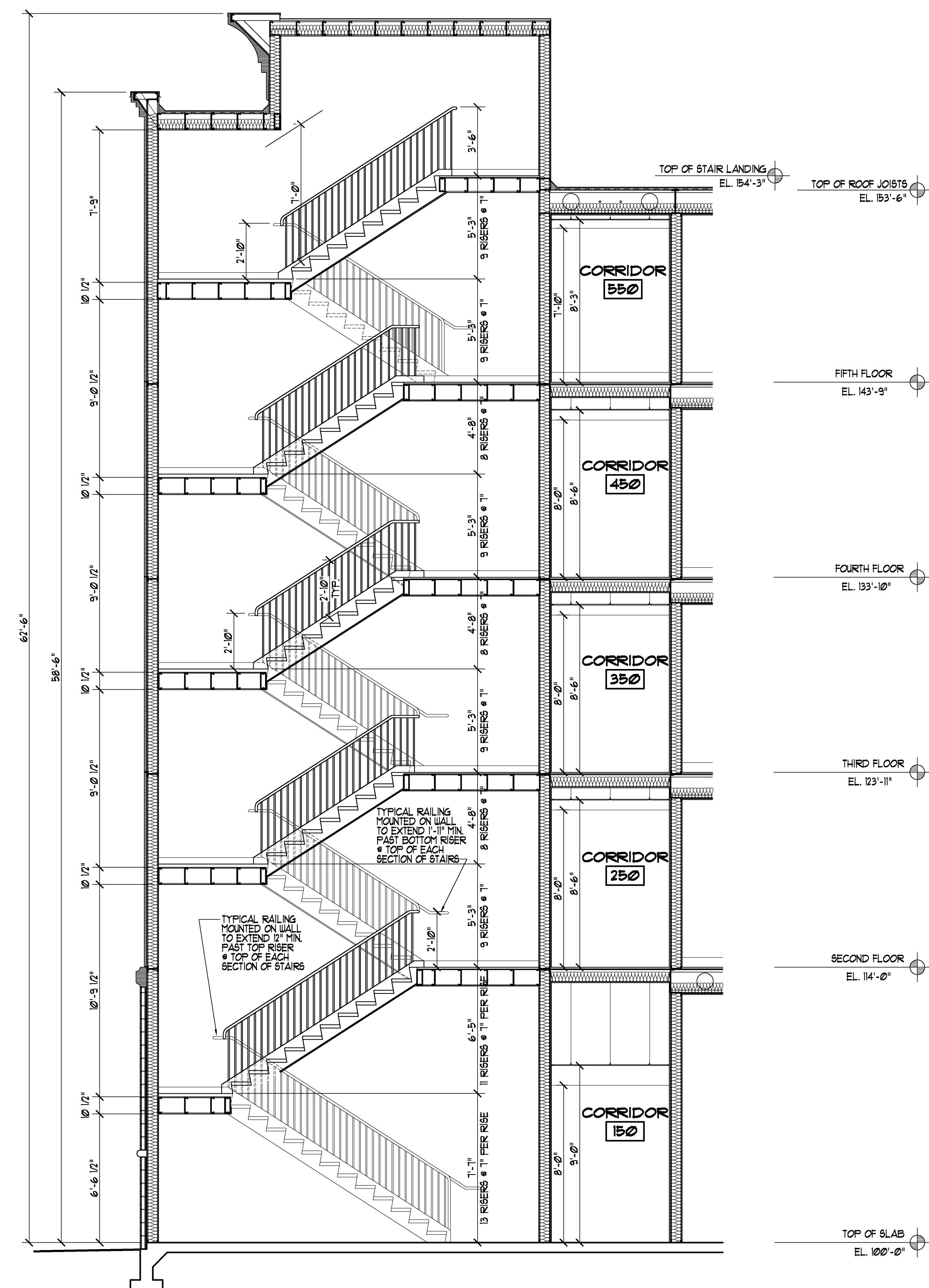
STAIRS SECTION 1/4" = 1'-0"
