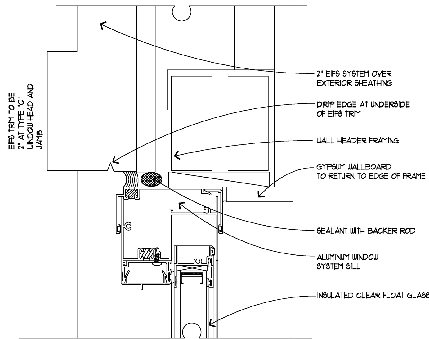
1 WINDOW HEAD (JAMB SIMILAR) A-30 HALF SCALE
