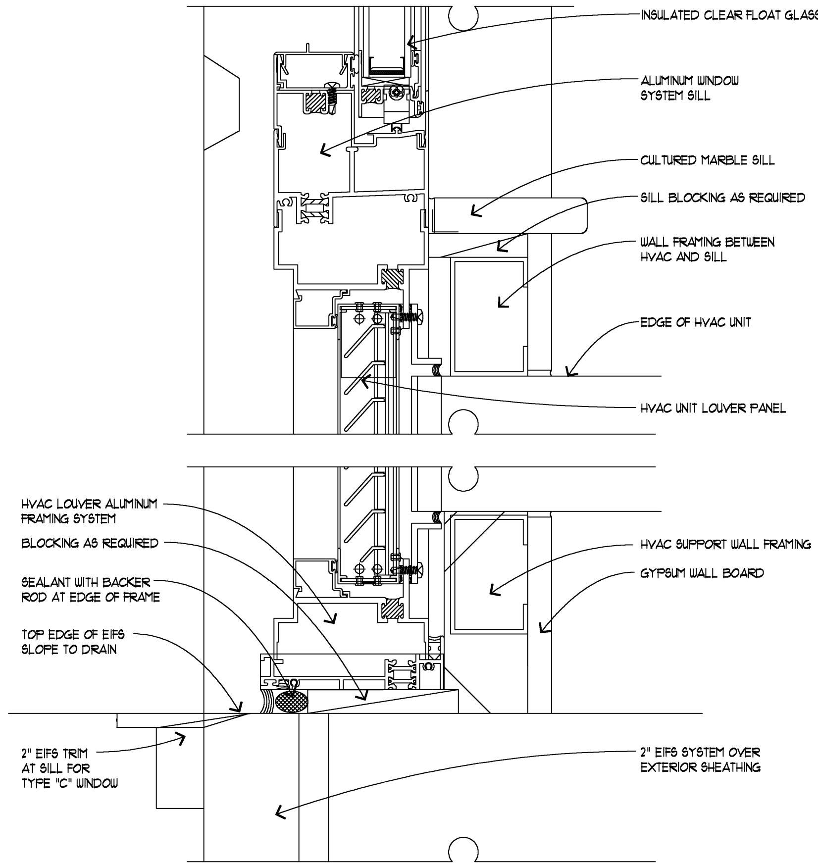
2 WINDOW SILL @ HVAC UNIT A-30 HALF SCALE
