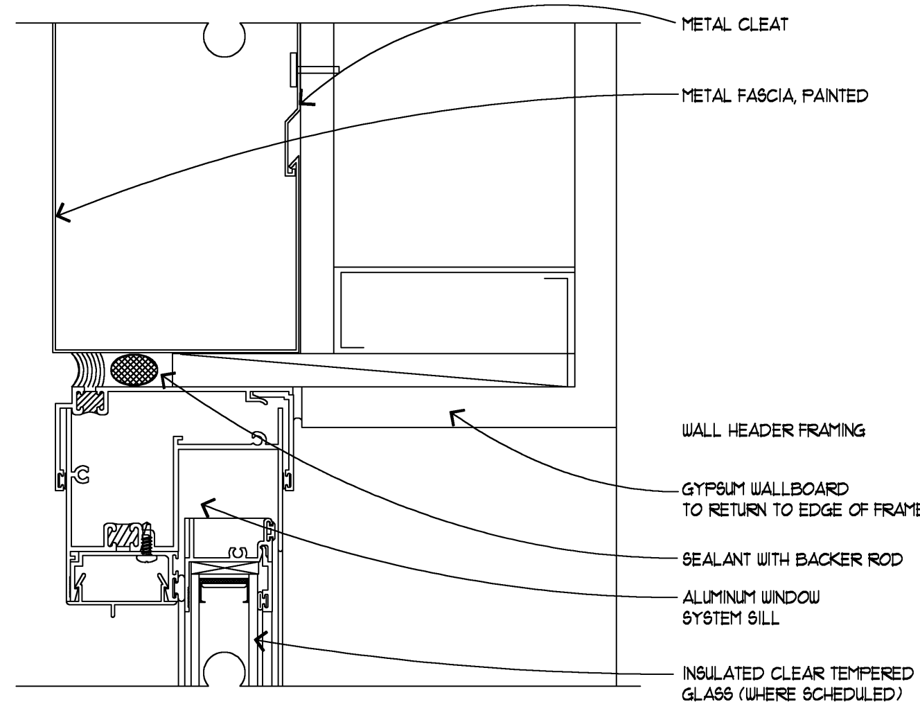
3 HEAD AT VENEER WALL A-30 HALF SCALE
