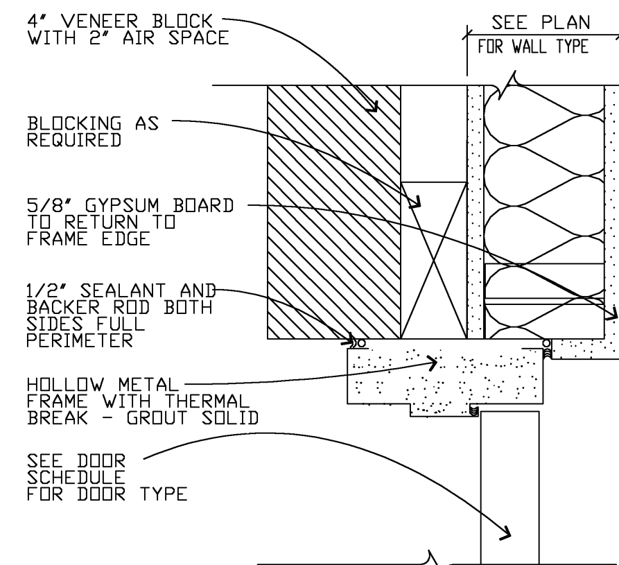
J6 JAMB 3" = 1'-0"
