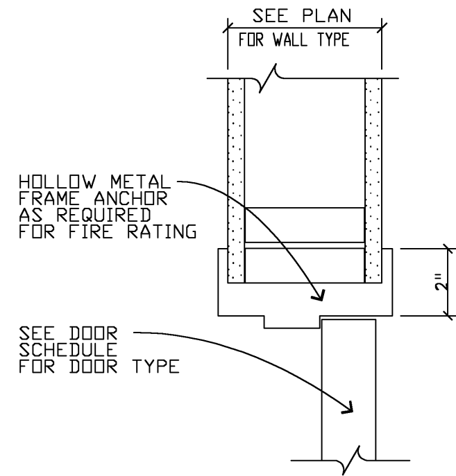
J1 JAMB 3" = 1'-0"
