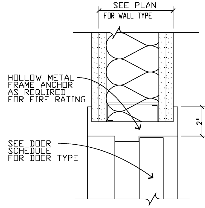
H4 HEAD 3" = 1'-0"
