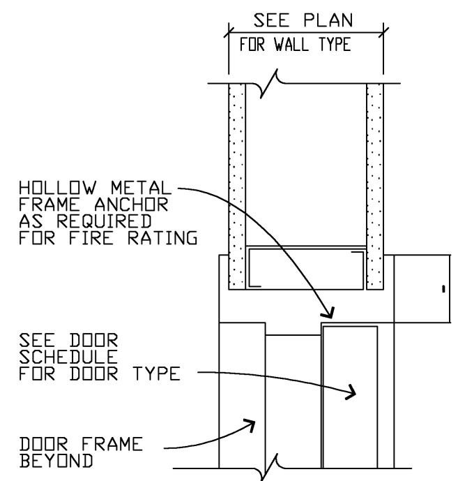
H1 HEAD 3" = 1'-0"
