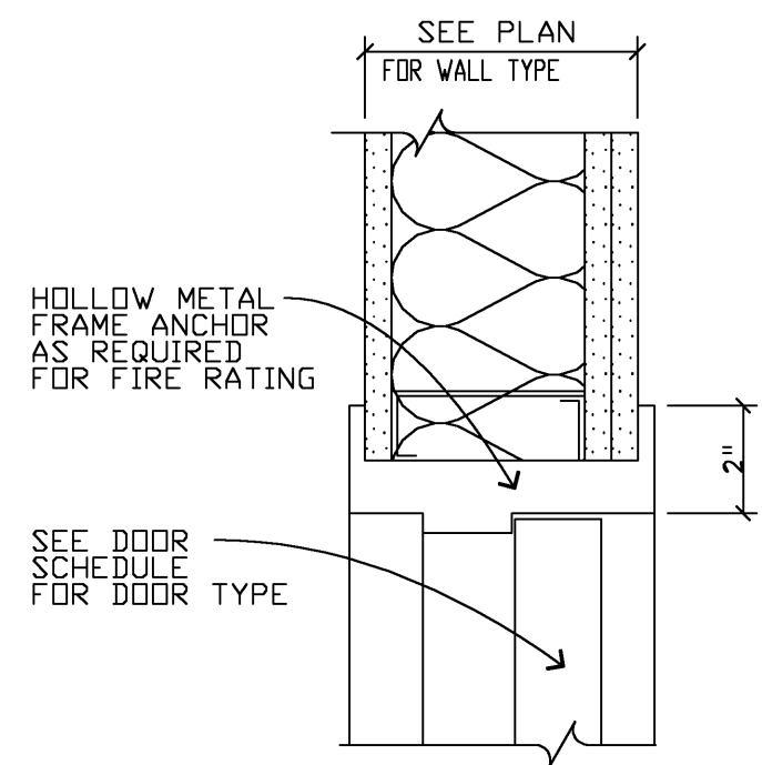
H3 HEAD 3" = 1'-0"
