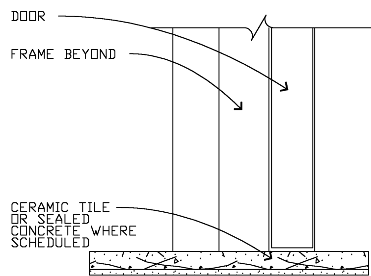
S2 SILL 3" = 1'-0"
