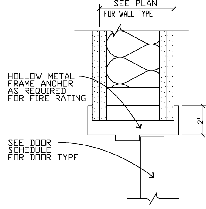
J4 JAMB 3" = 1'-0"
