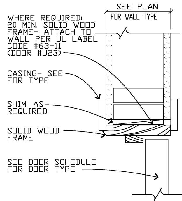
J2 JAMB 3" = 1'-0"
