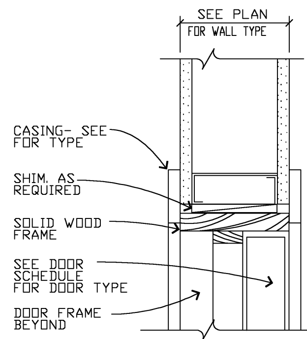
H2 HEAD 3" = 1'-0"
