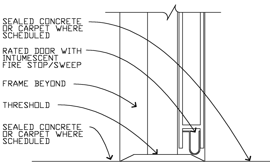
S5 SILL 3" = 1'-0"
