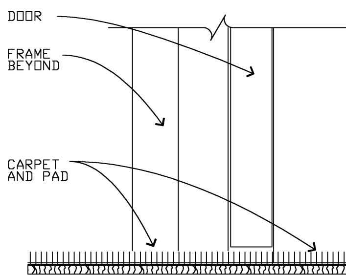
S3 SILL 3" = 1'-0"
