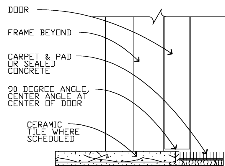
S1 SILL 3" = 1'-0"
