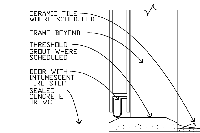
S7 SILL 3" = 1'-0"
