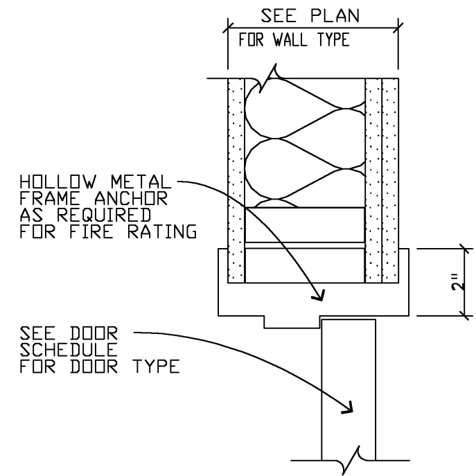
J3 JAMB 3" = 1'-0"
