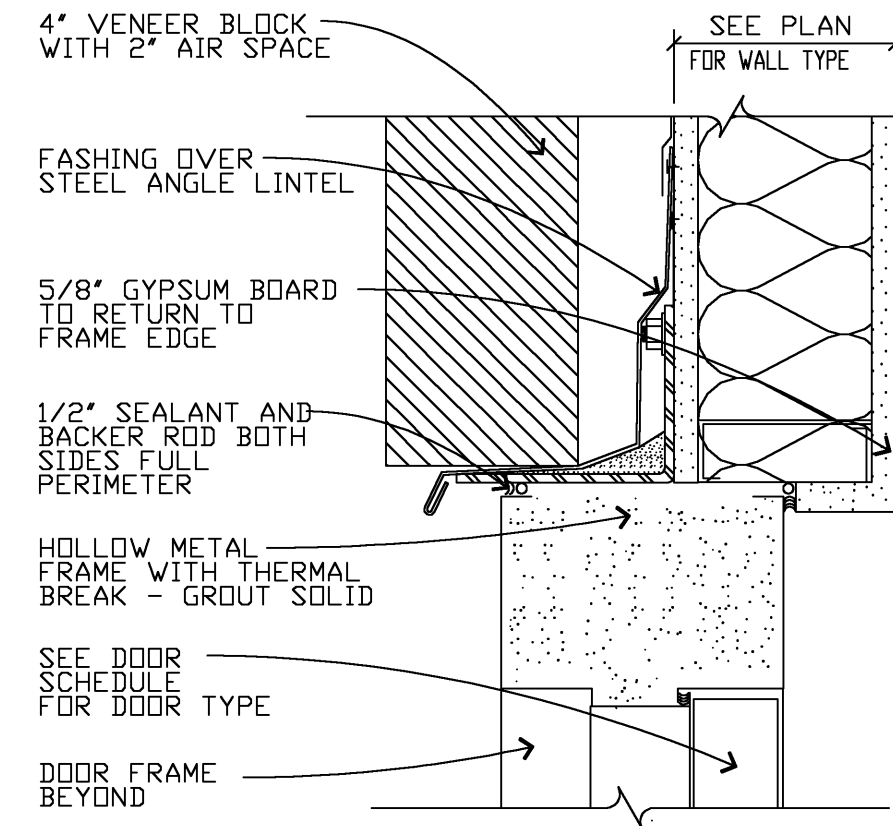
H6 HEAD 3" = 1'-0"
