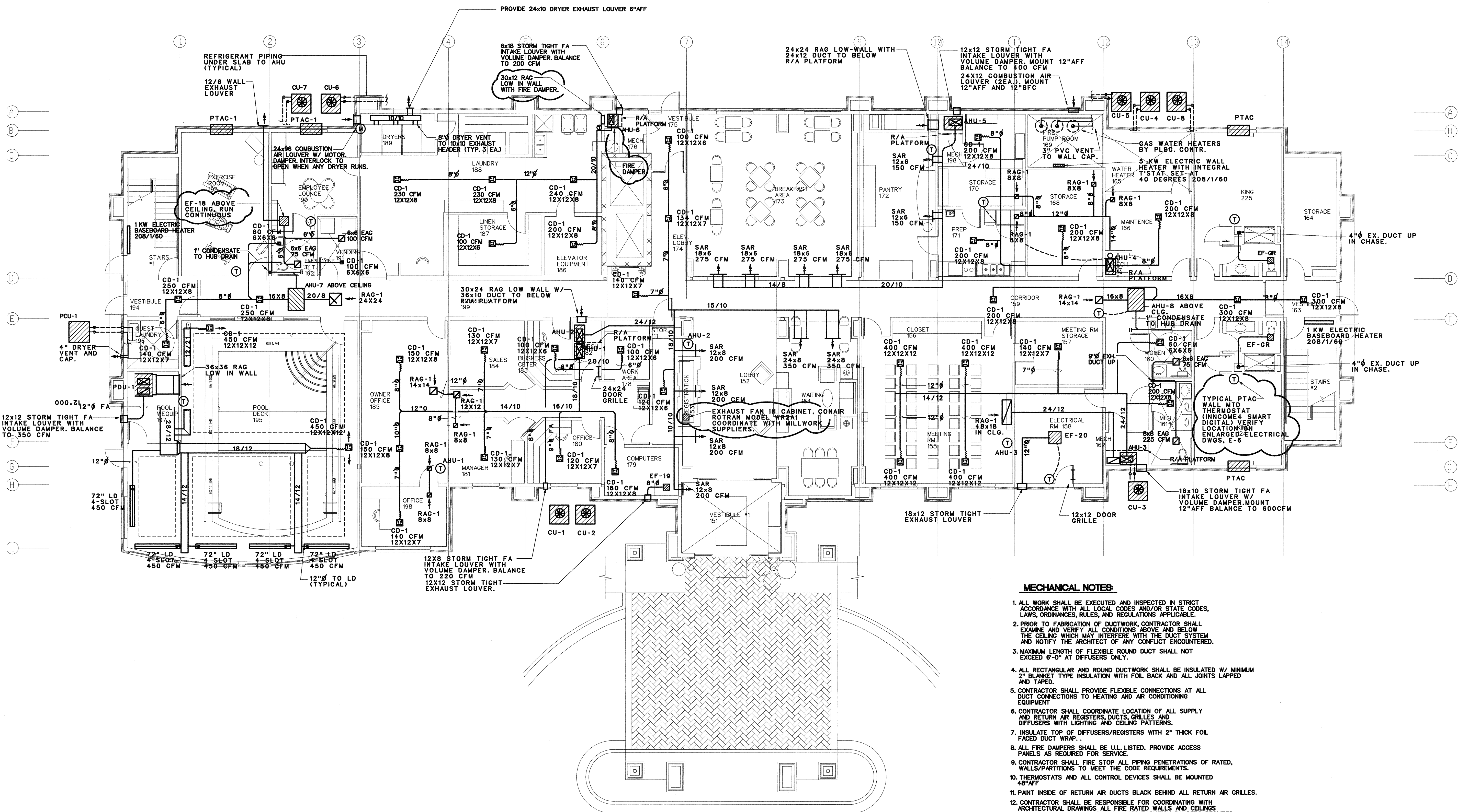
HVAC PLAN - FIRST FLOOR SCALE: 1/4" = 1'-0"
