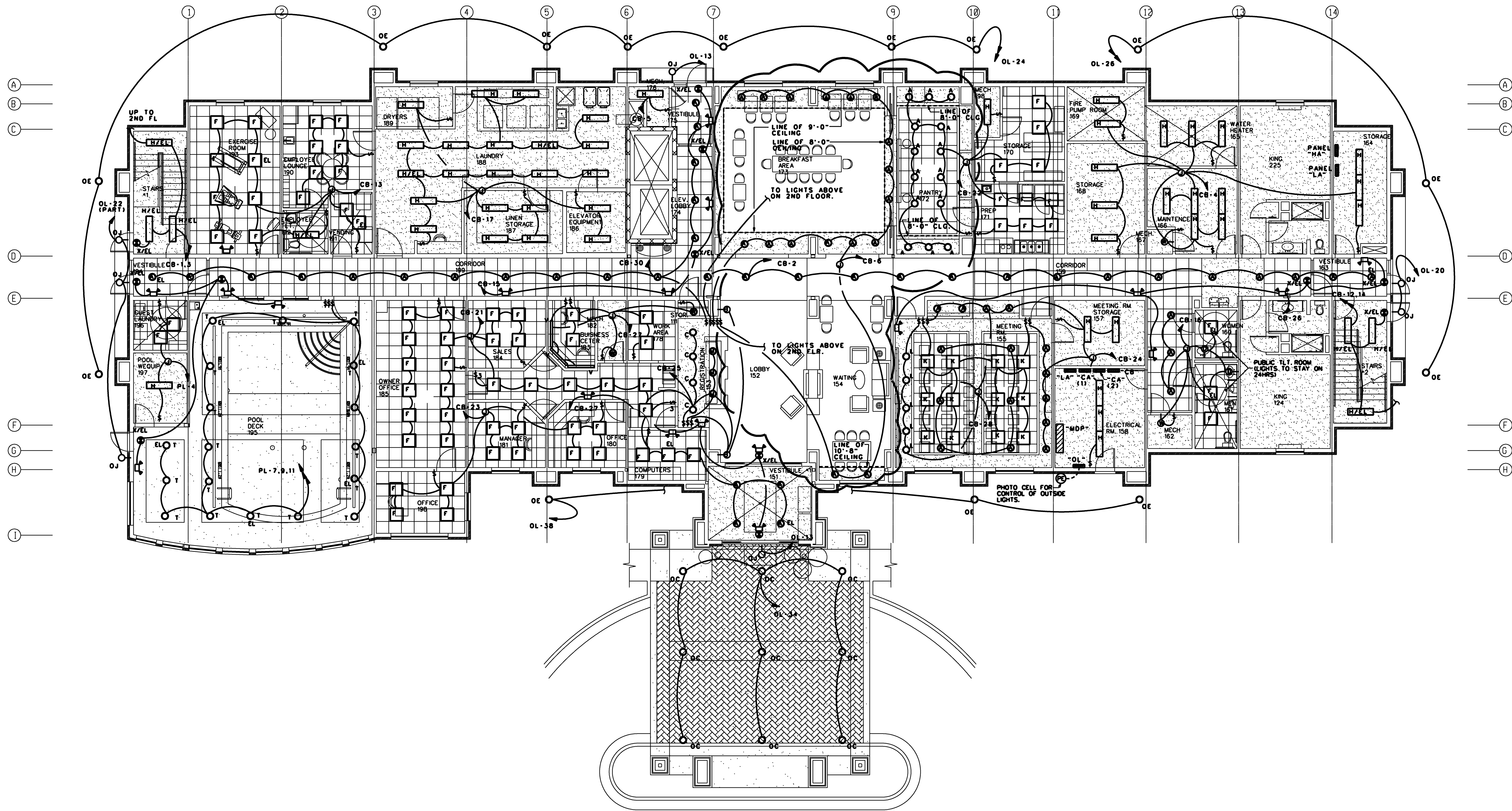
LIGHTING PLAN - FIRST FLOOR SCALE: 1/8" = 1'-0"
