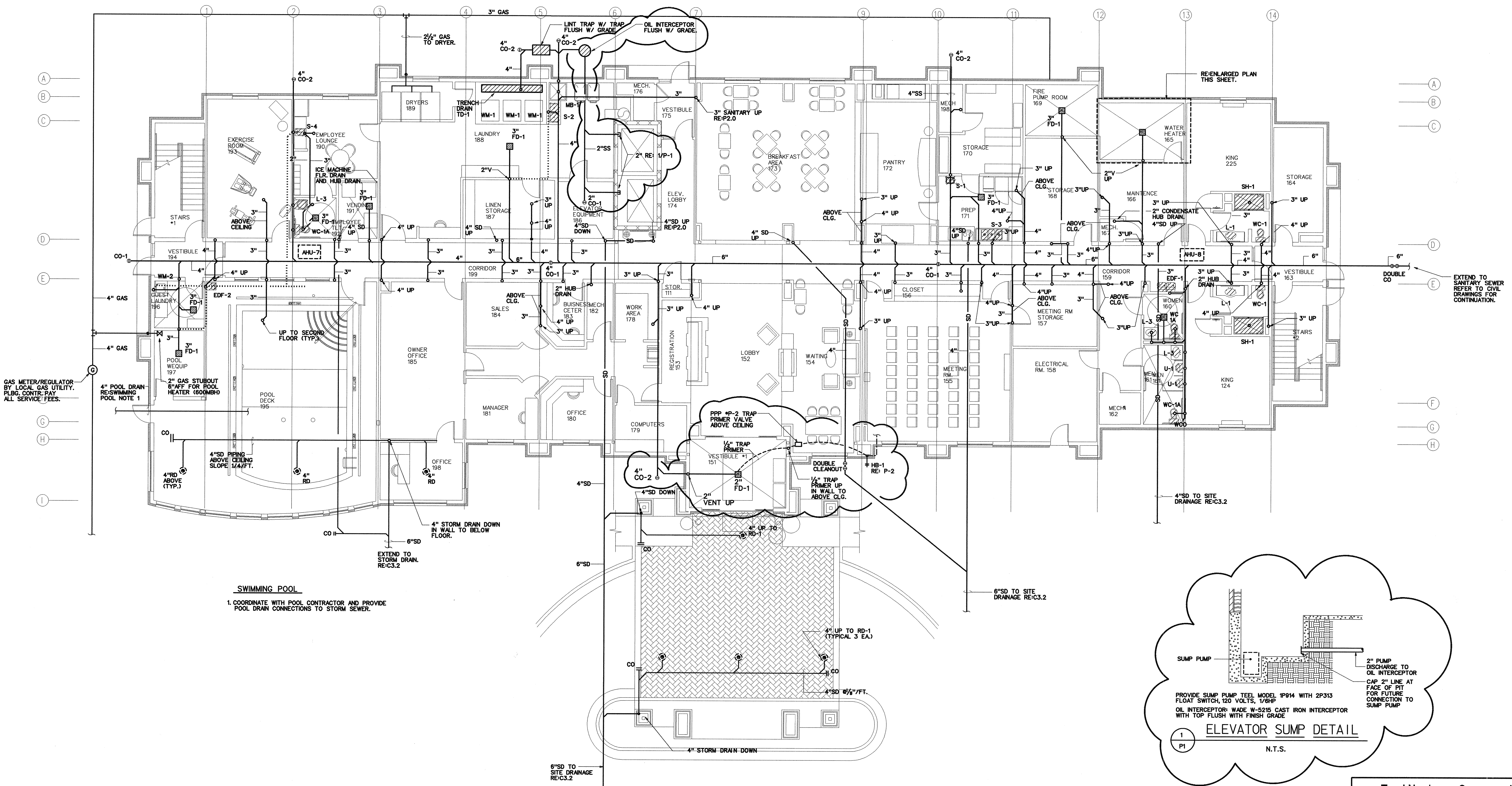
PLUMBING PLAN - FIRST FLOOR SCALE: 1/4" = 1'-0"
