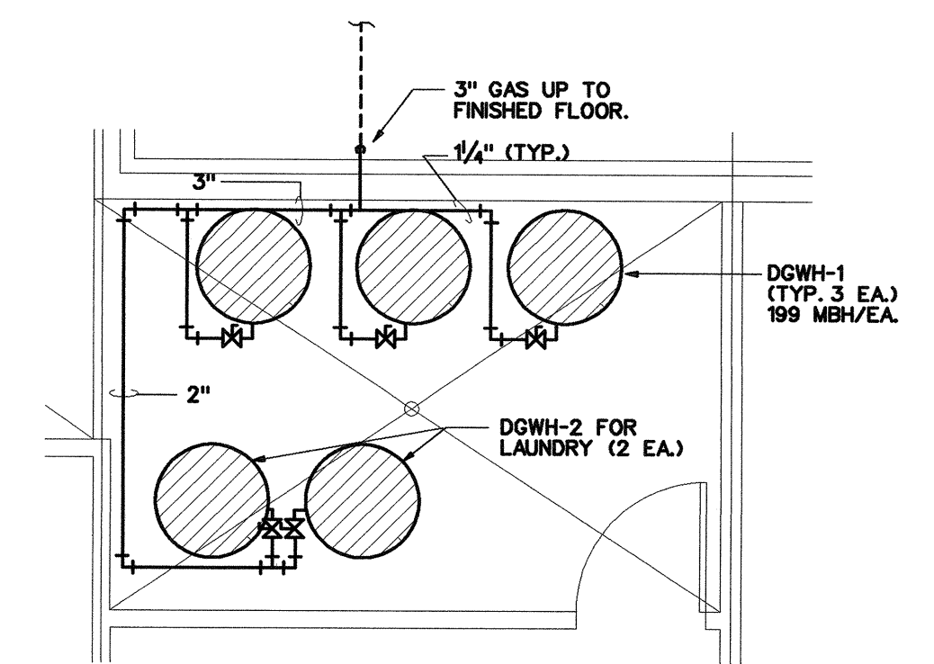
ENLARGED WATER HEATER RM. SCALE: 1/4" = 1'-0"
