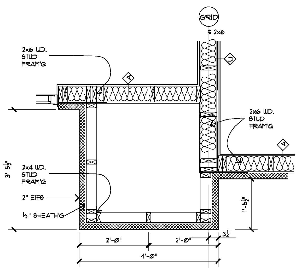
13 PILASTER DETAIL 3/4" = 1' 0"
