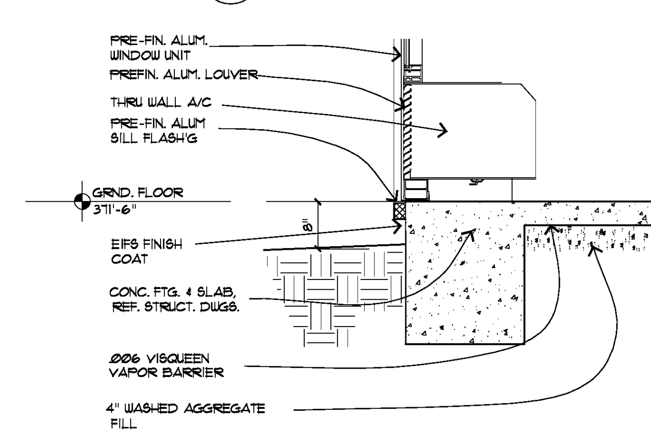
5 FOUNDATION DETAIL 3/4" = 1' 0"
