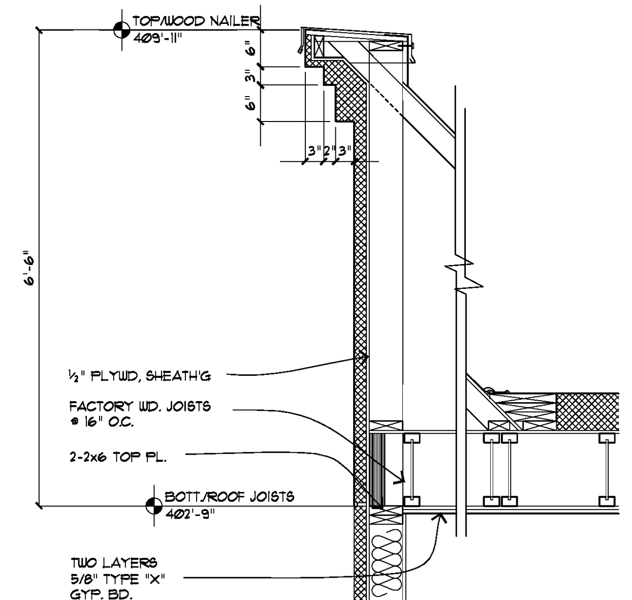
4 CORNICE DETAIL 3/4" = 1' 0"
