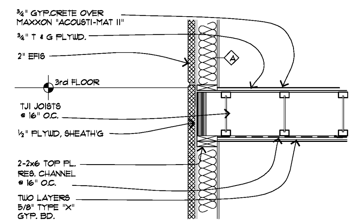
3 WALL DETAIL 3/4" = 1' 0"
