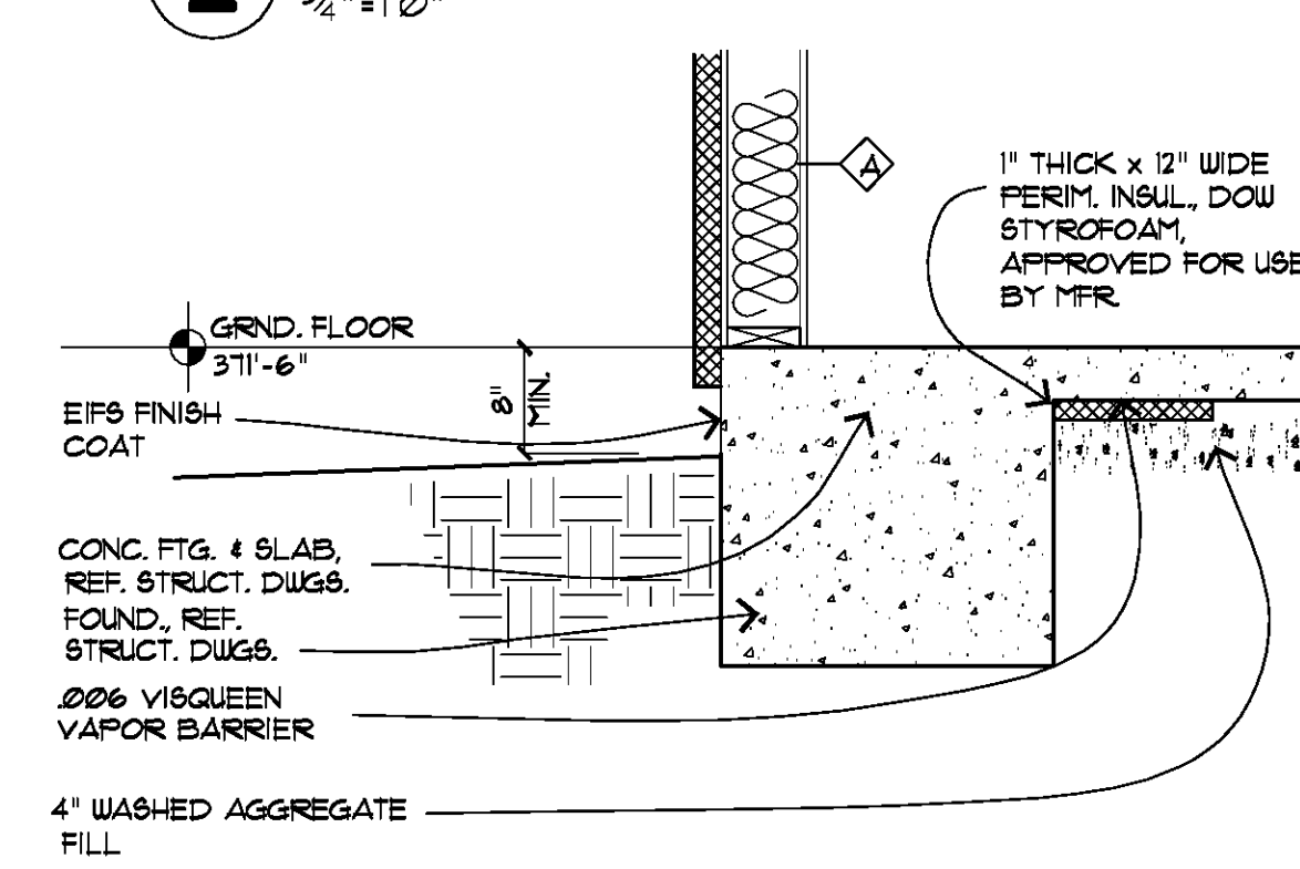
1 FOUNDATION DETAIL 3/4" = 1' 0"
