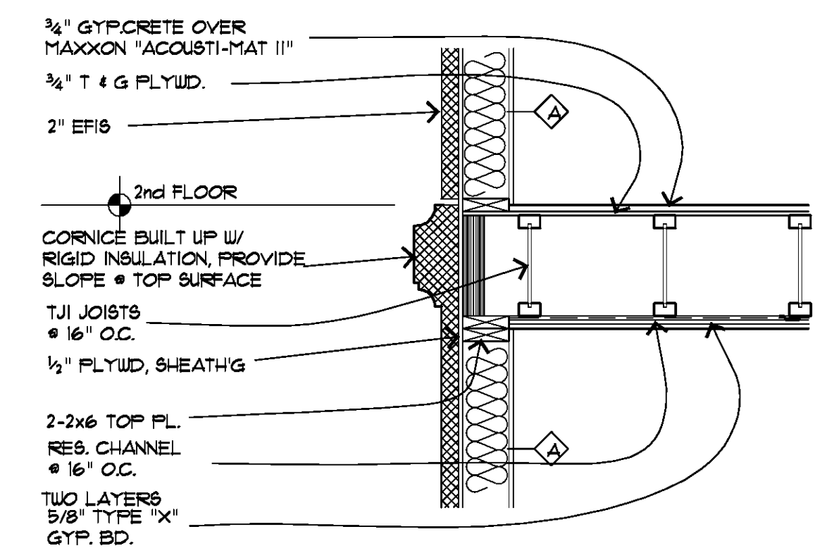
2 WALL DETAIL 3/4" = 1' 0"
