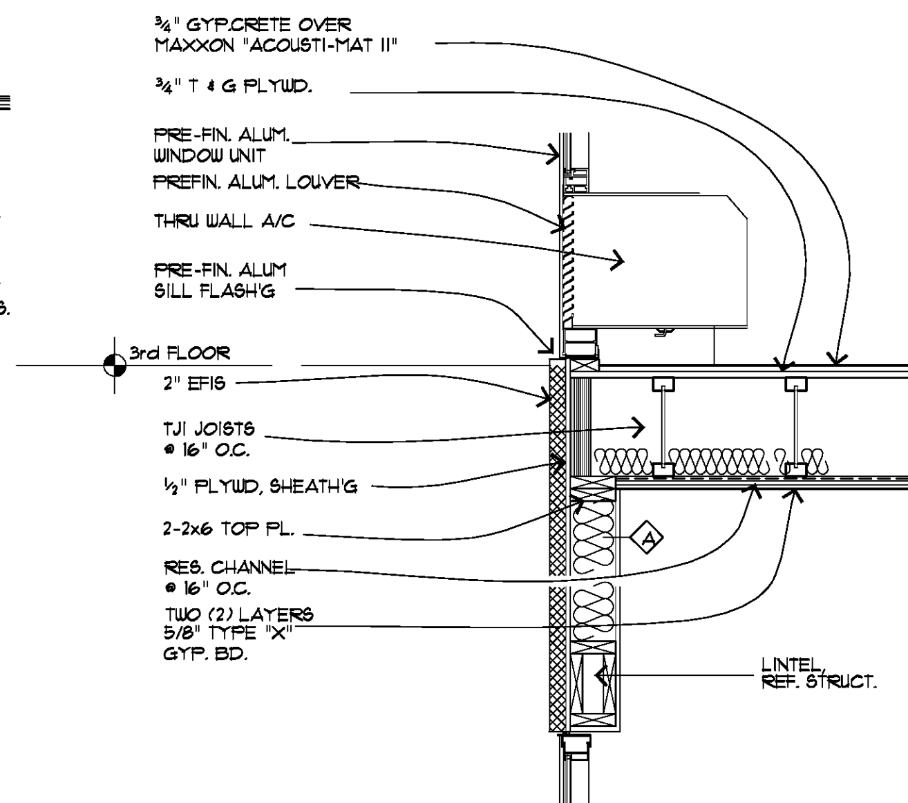
7 WALL DETAIL 3/4" = 1' 0"
