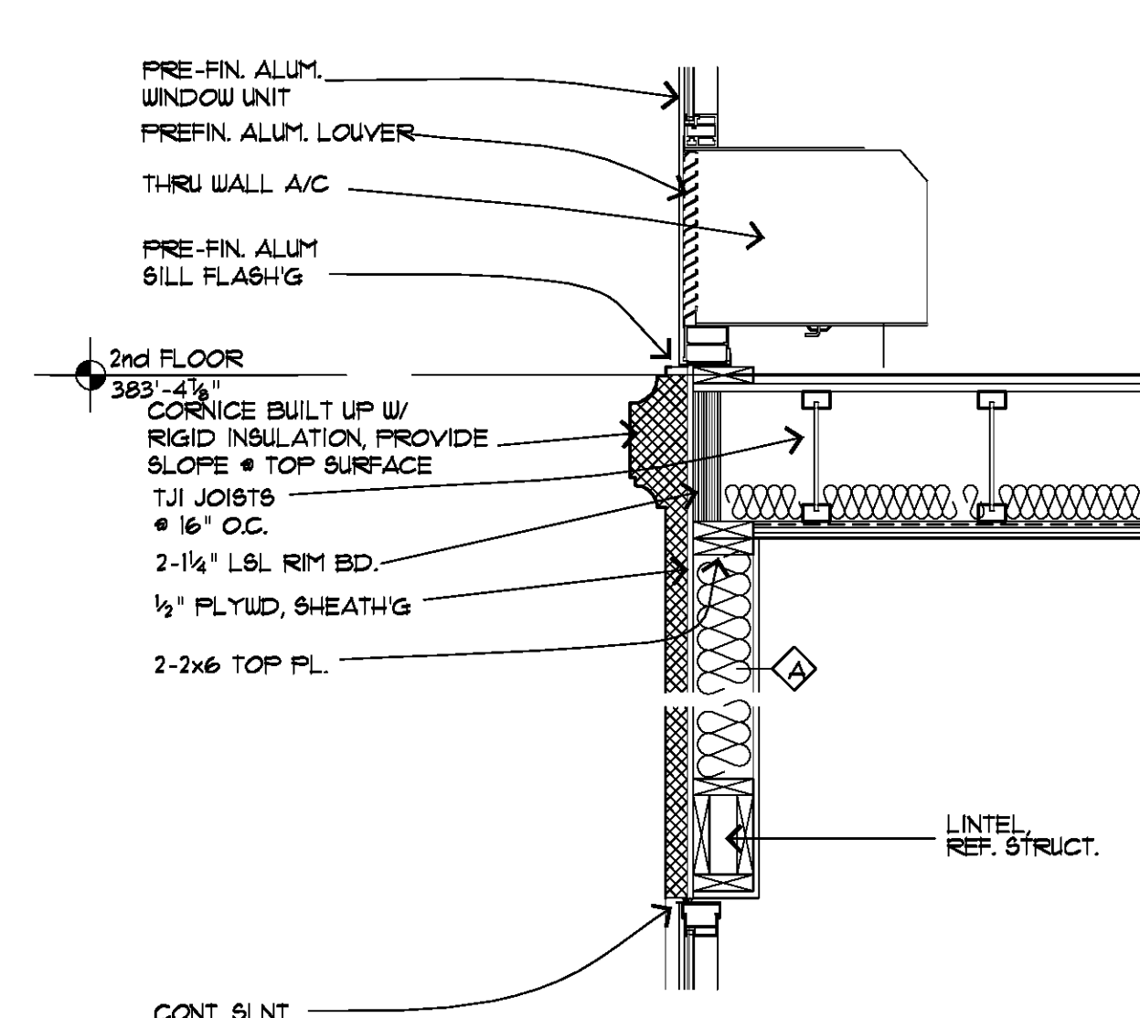
6 WALL DETAIL 3/4" = 1' 0"
