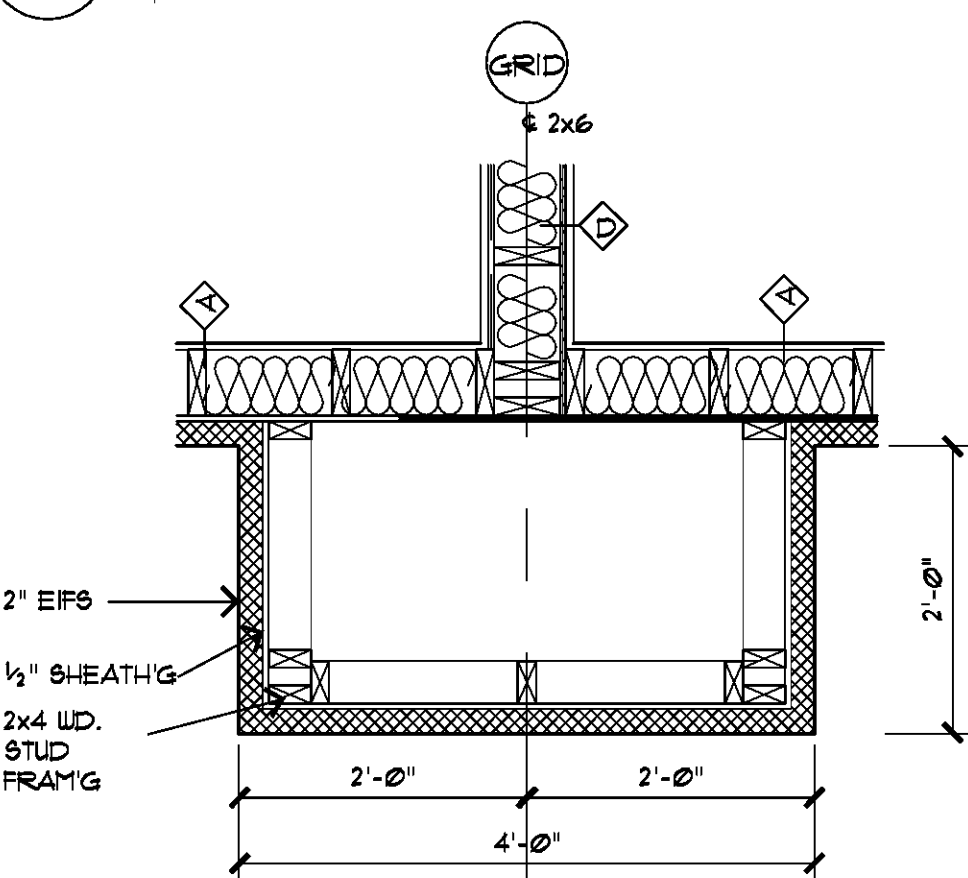
12 PILASTER DETAIL 3/4" = 1' 0"
