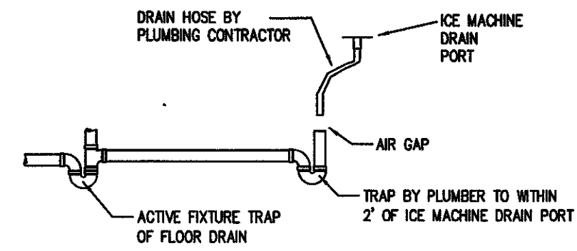
ICE MACHINE HUB DRAIN AT FLOOR DRAIN SCALE: NONE
