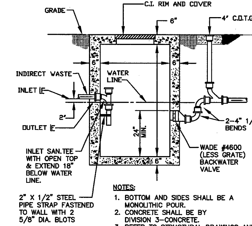
CATCH BASIN NO SCALE
