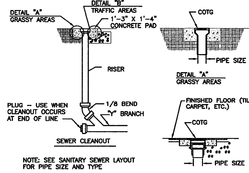
CLEANOUT TO FLOOR OR GRADE SCALE: NONE
