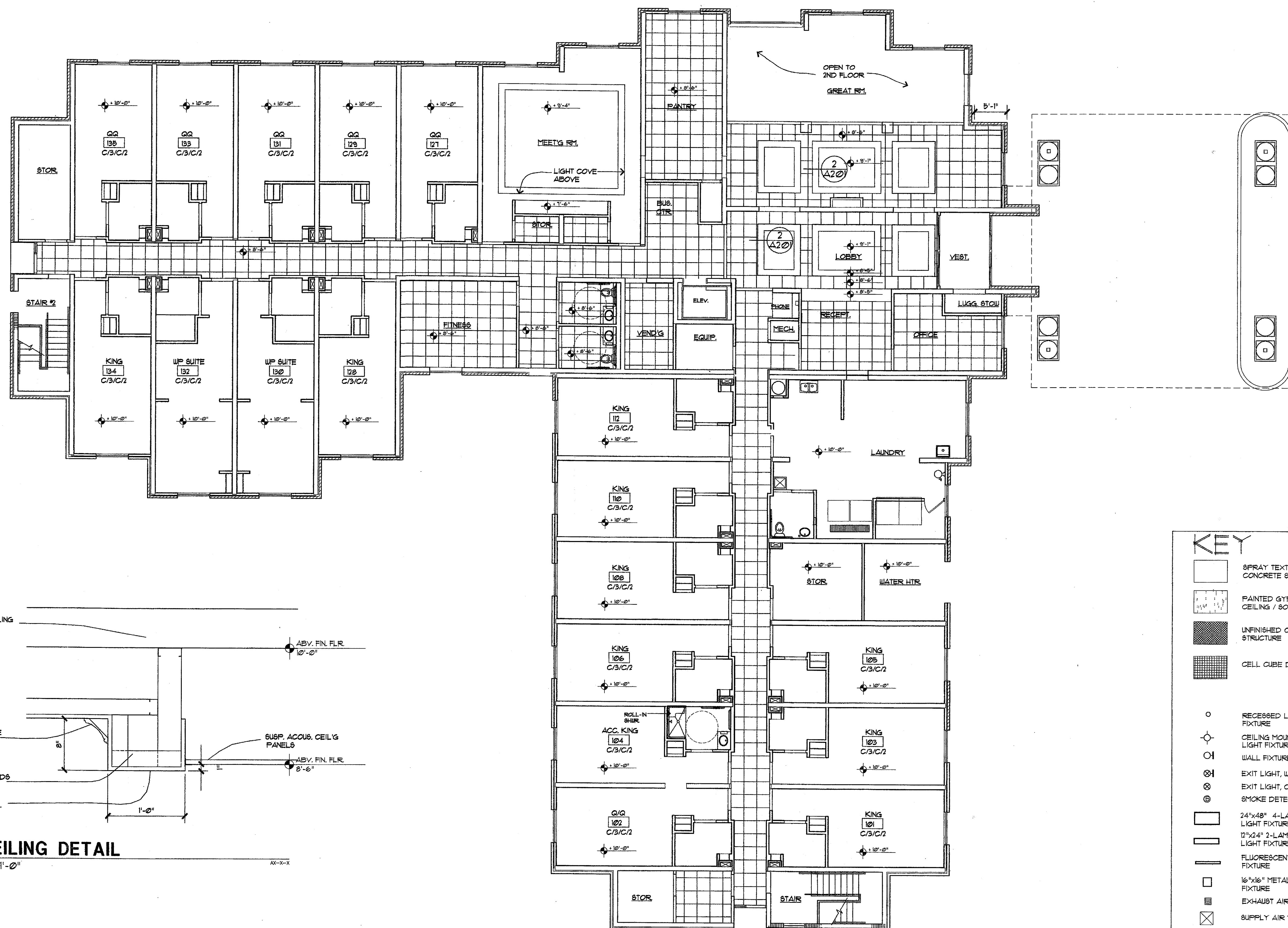
1 GROUND FLOOR CEILING PLAN 1/8" = 1'-0"
