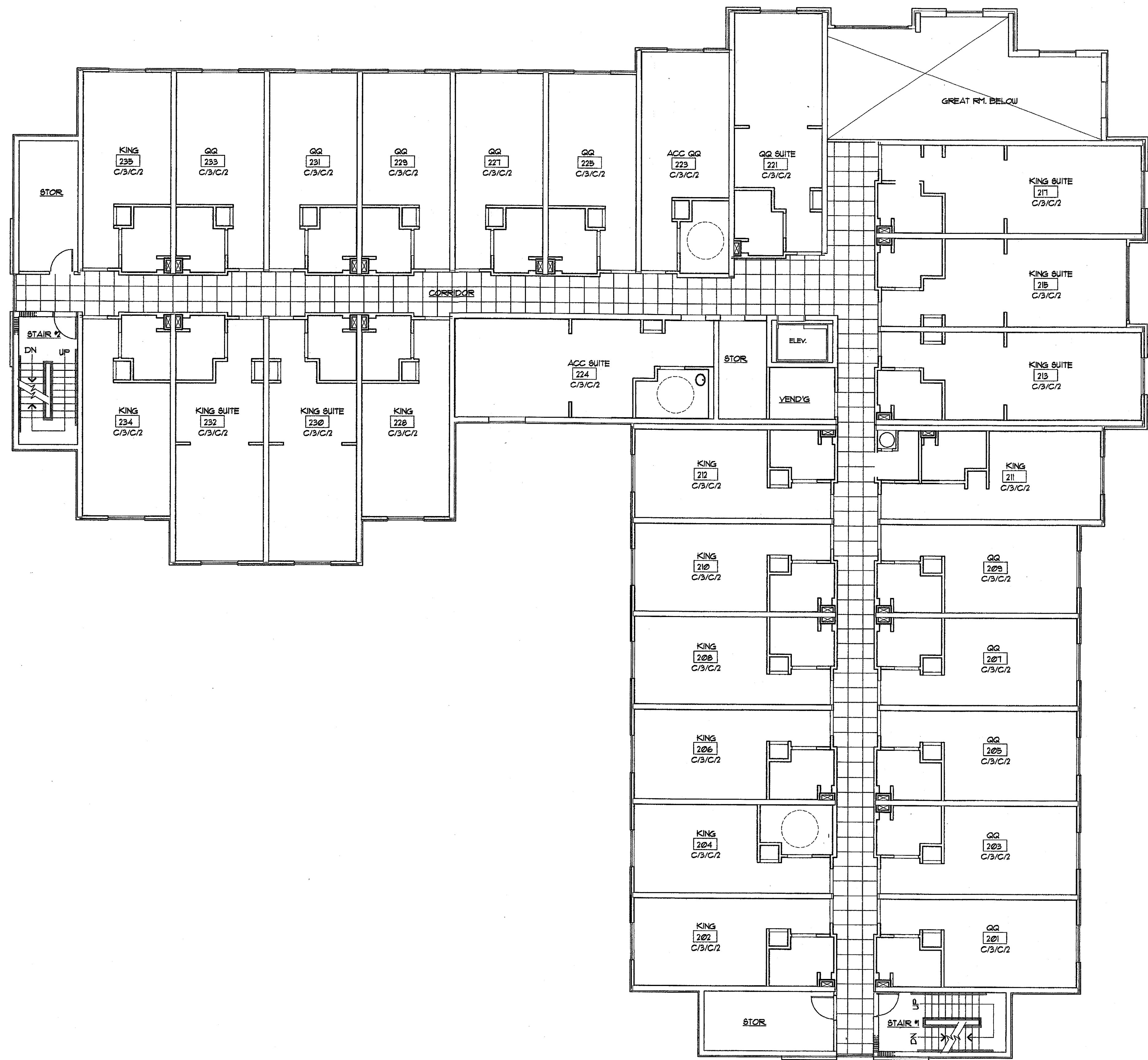
1 2nd FLOOR CEILING PLAN 1/8"=1'-0" AK-X-X KING RMS DBL QUEEN RMS SUITES TOTAL 9 12 1 28
