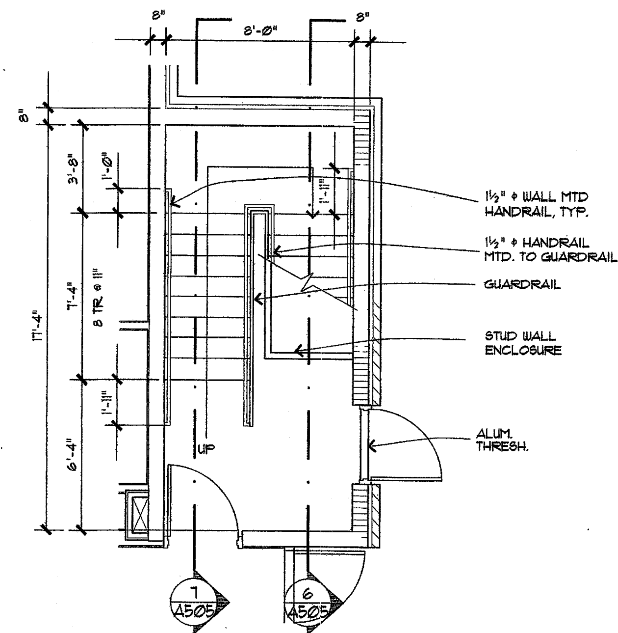
1 STAIR No. 1, GROUND FLOOR 1/4" = 1'-0"
