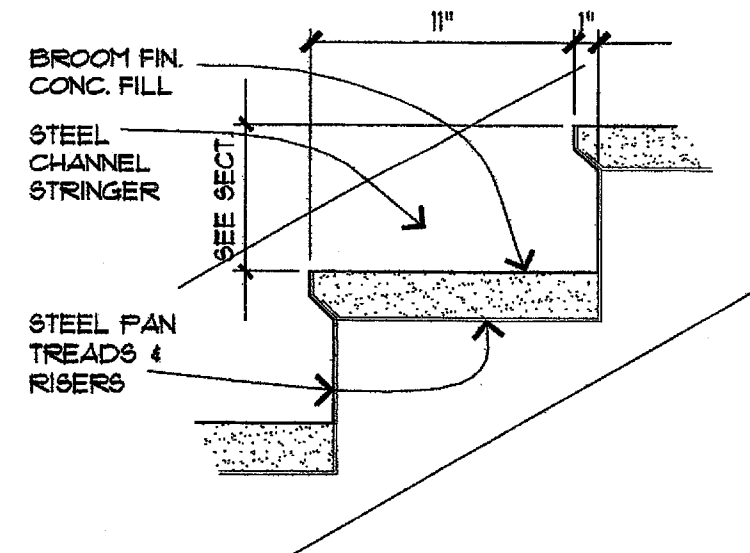
5 STAIR TREAD DET. 1/2" = 1'-0"
