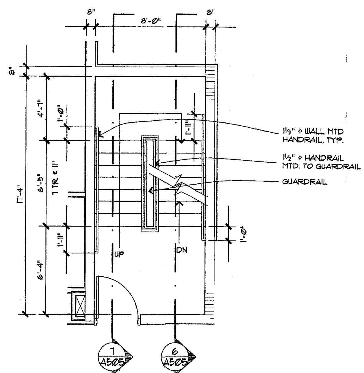
2 STAIR No. 1, 2nd FLOOR 1/4" = 1'-0"
