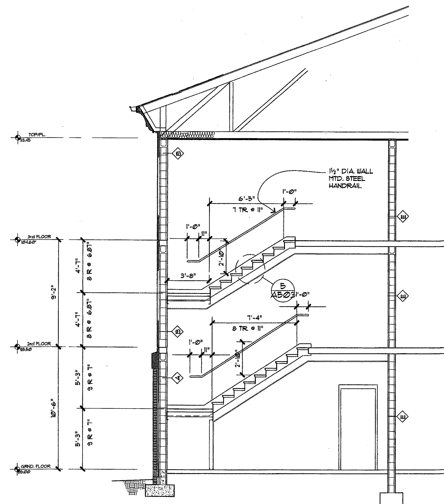
6 STAIR SECTION 1/4" = 1'-0"
