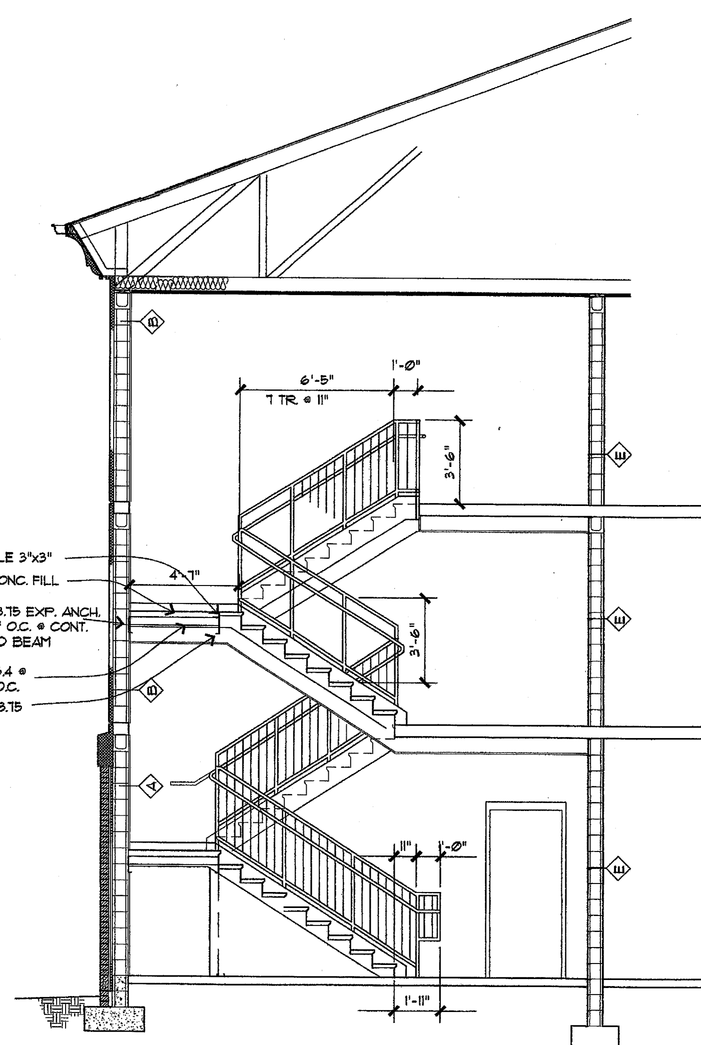
7 STAIR SECTION 1/4" = 1'-0"
