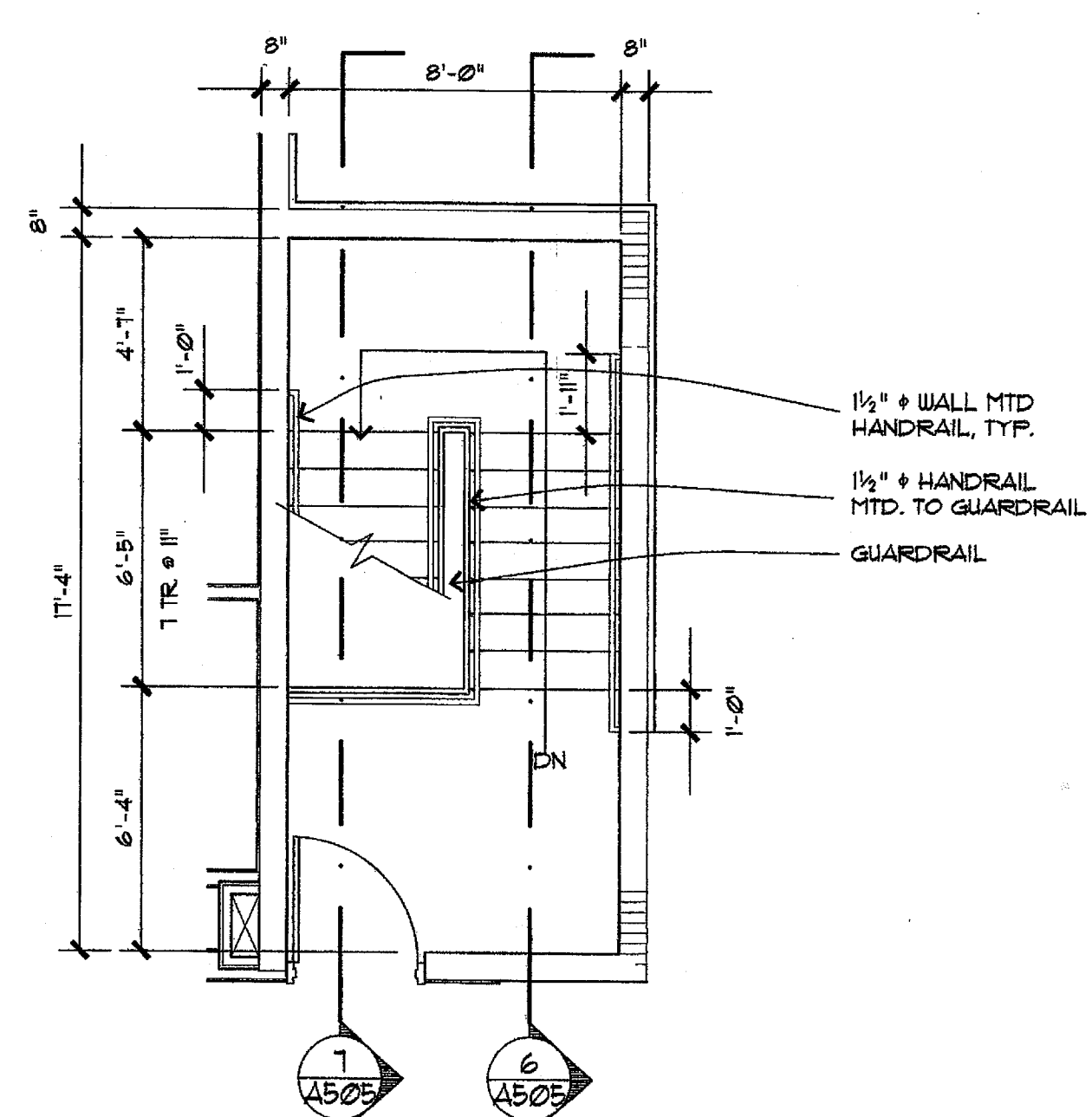
3 STAIR No. 1, 3rd FLR 1/4" = 1'-0"
