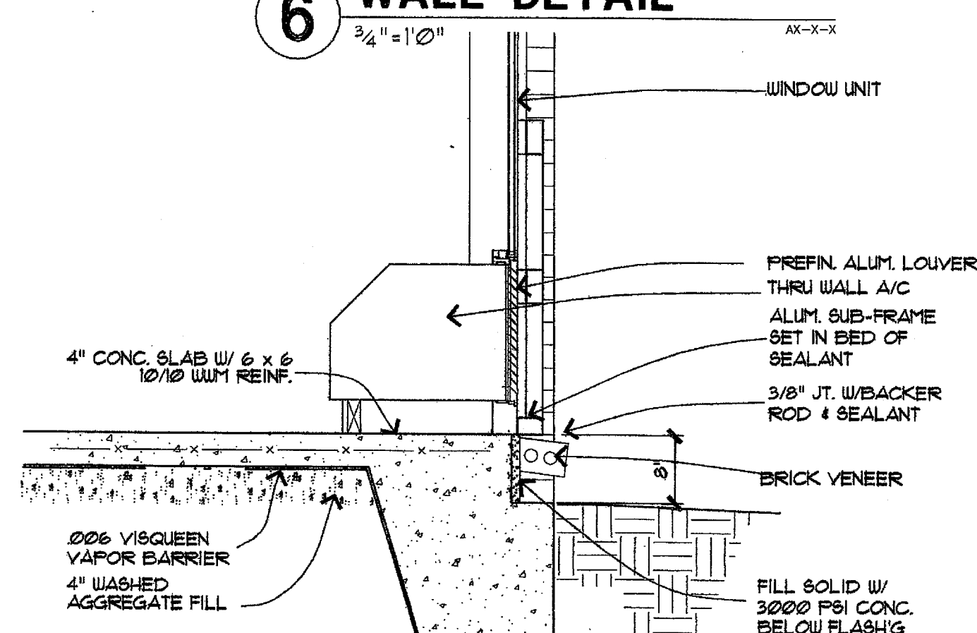
6 WALL DETAIL 3/4" = 1'-0"
