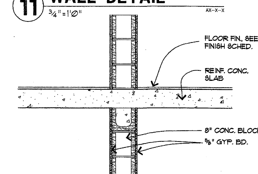
11 WALL DETAIL 3/4" = 1'-0"
