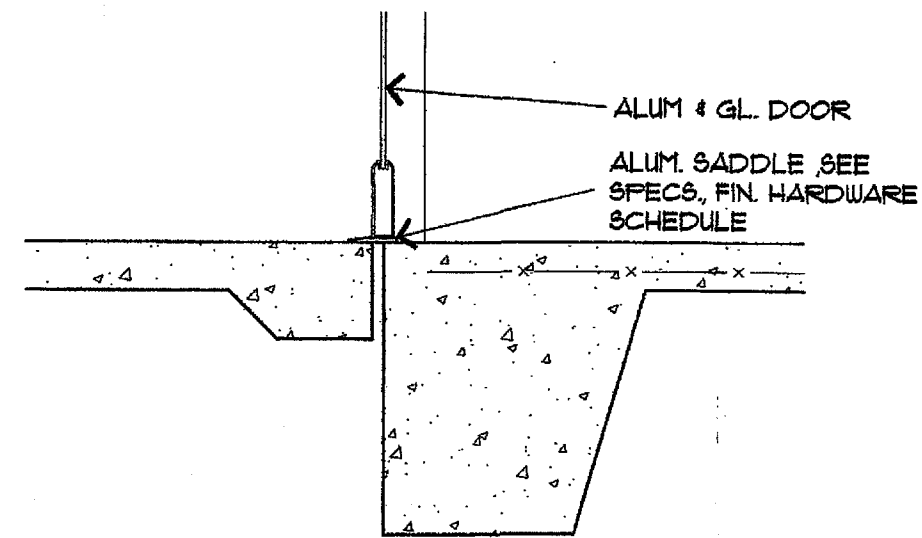
13 FOUNDATION DETAIL 3/4" = 1'-0"
