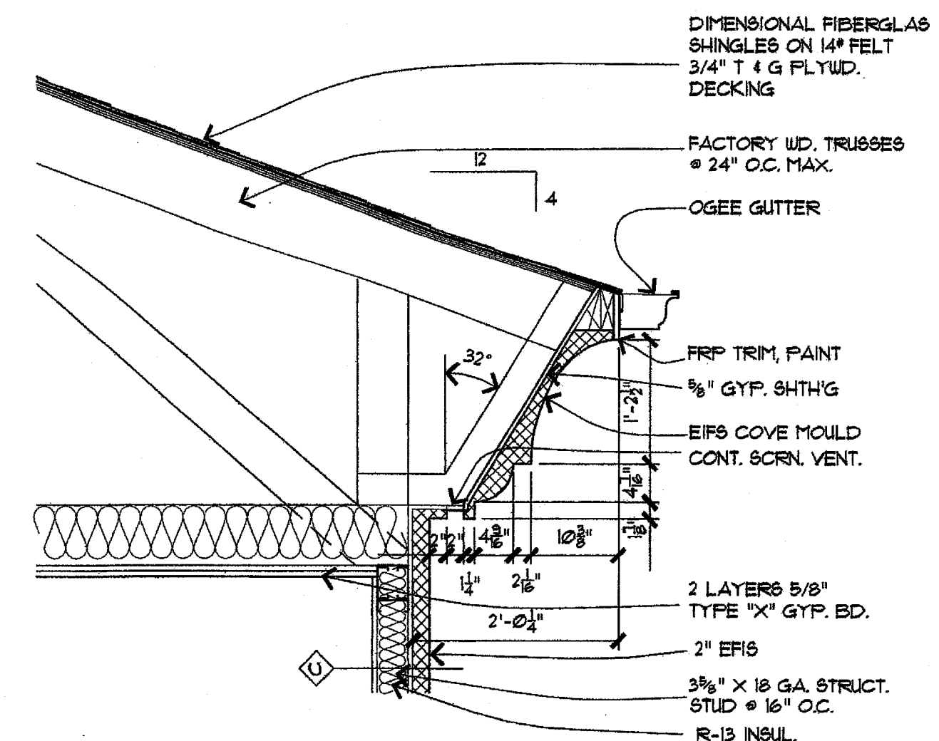
4 CORNICE DETAIL 3/4" = 1'-0"
