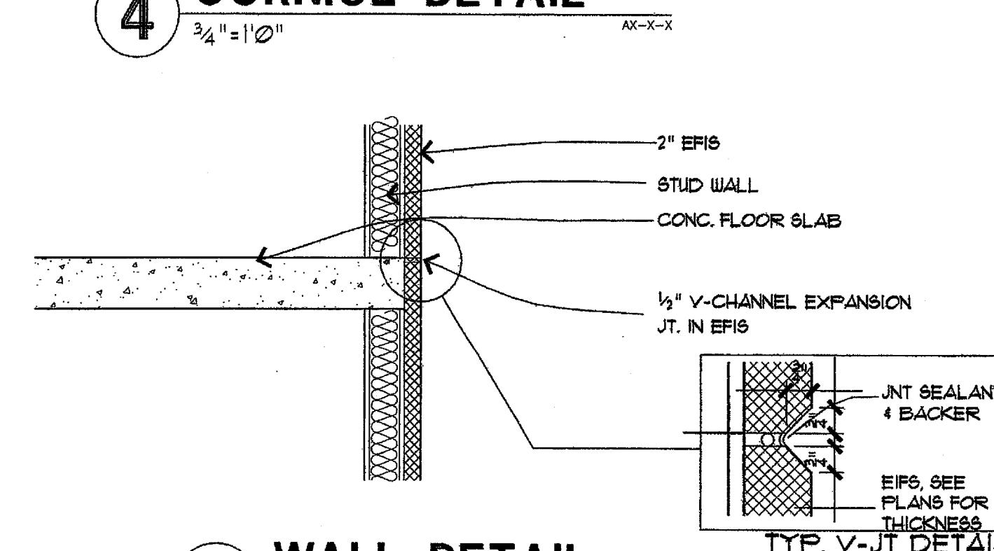
3 WALL DETAIL 3/4" = 1'-0"
