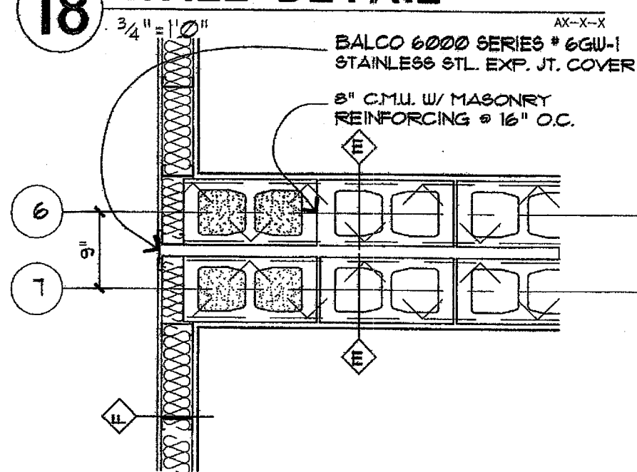
17 WALL DETAIL 3/4" = 1'-0"
