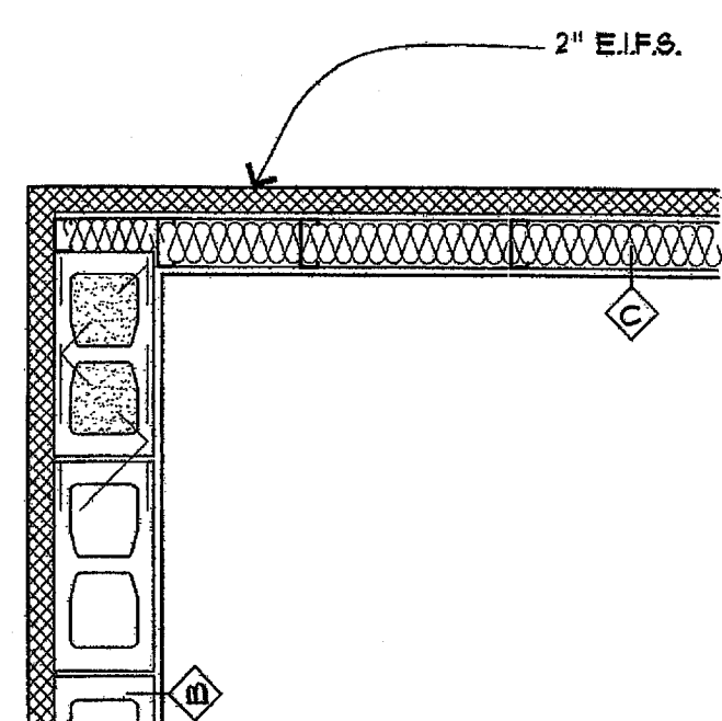
14 WALL DETAIL 3/4" = 1'-0"
