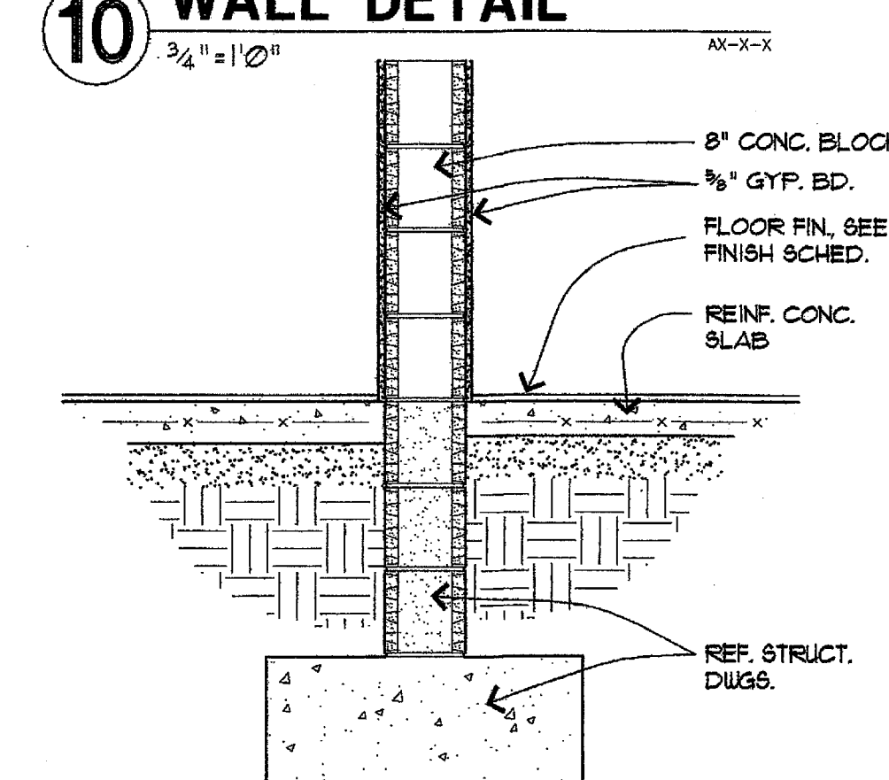
10 WALL DETAIL 3/4" = 1'-0"
