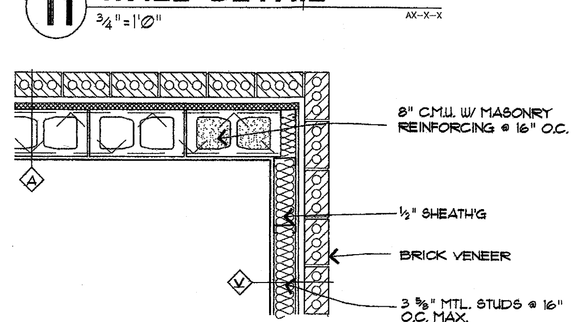
11 WALL DETAIL 3/4" = 1'-0"
