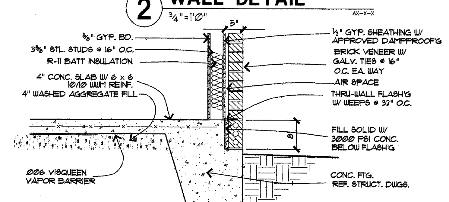
2 WALL DETAIL 3/4" = 1'-0"
