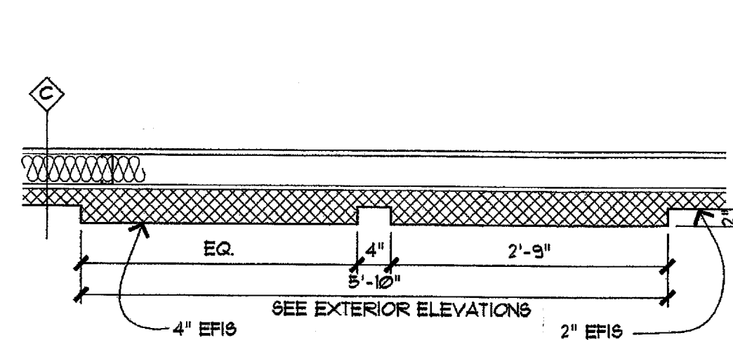
8 PILASTER DETAIL 3/4" = 1'-0"
