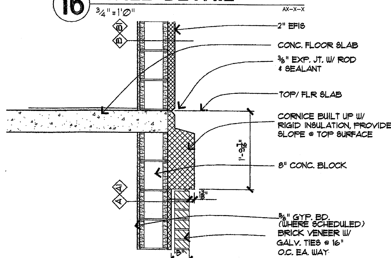
15 WALL DETAIL 3/4" = 1'-0"
