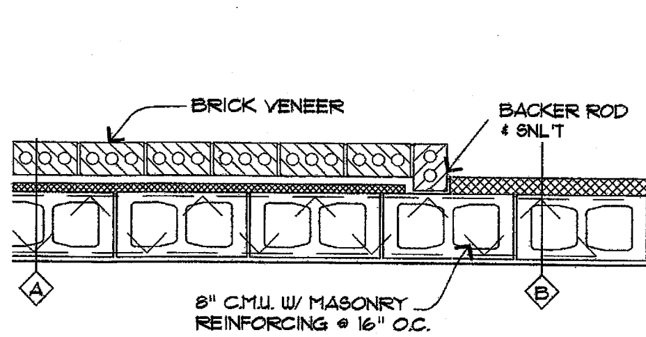
18 WALL DETAIL 3/4" = 1'-0"
