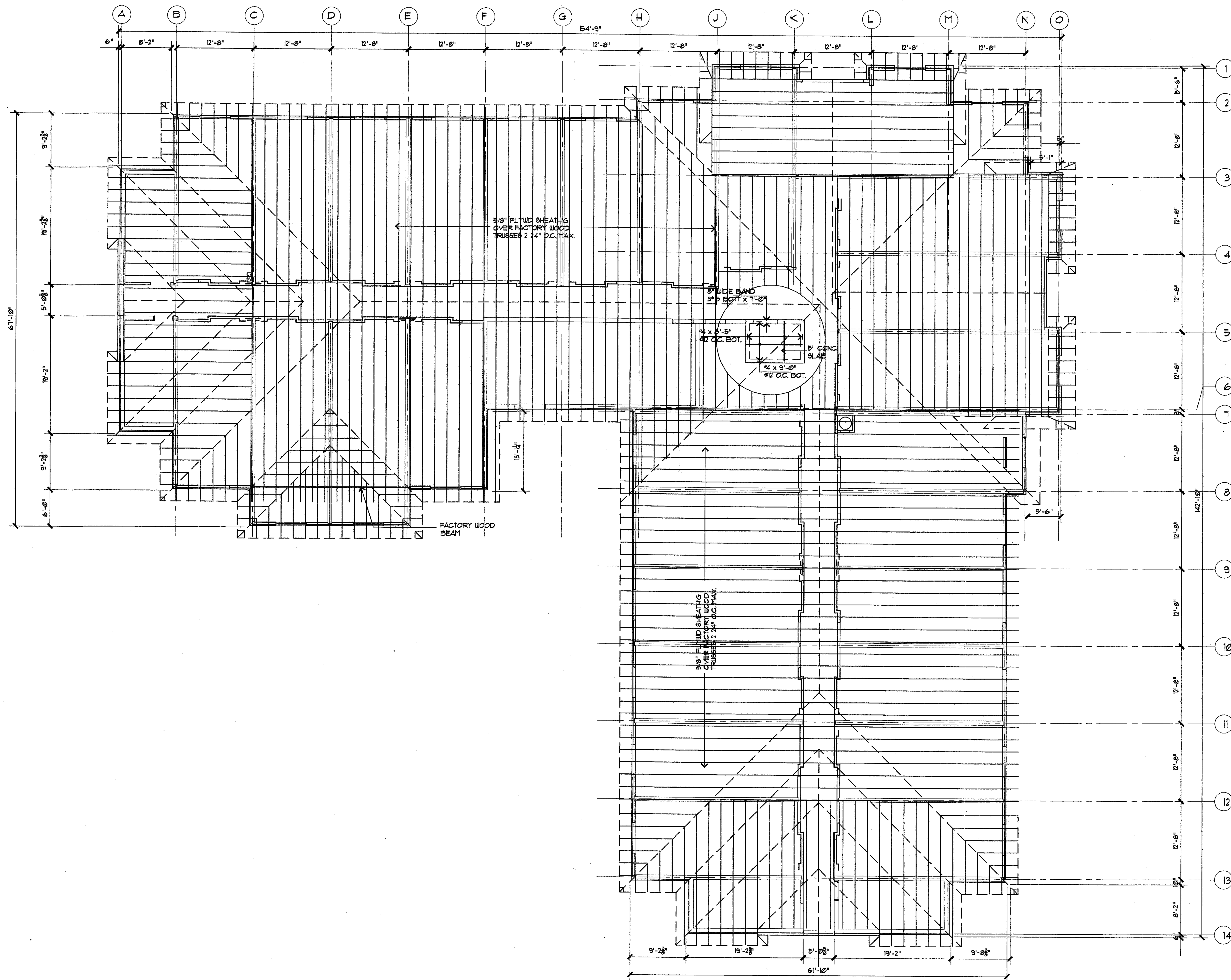
1 ROOF FRAMING PLAN
