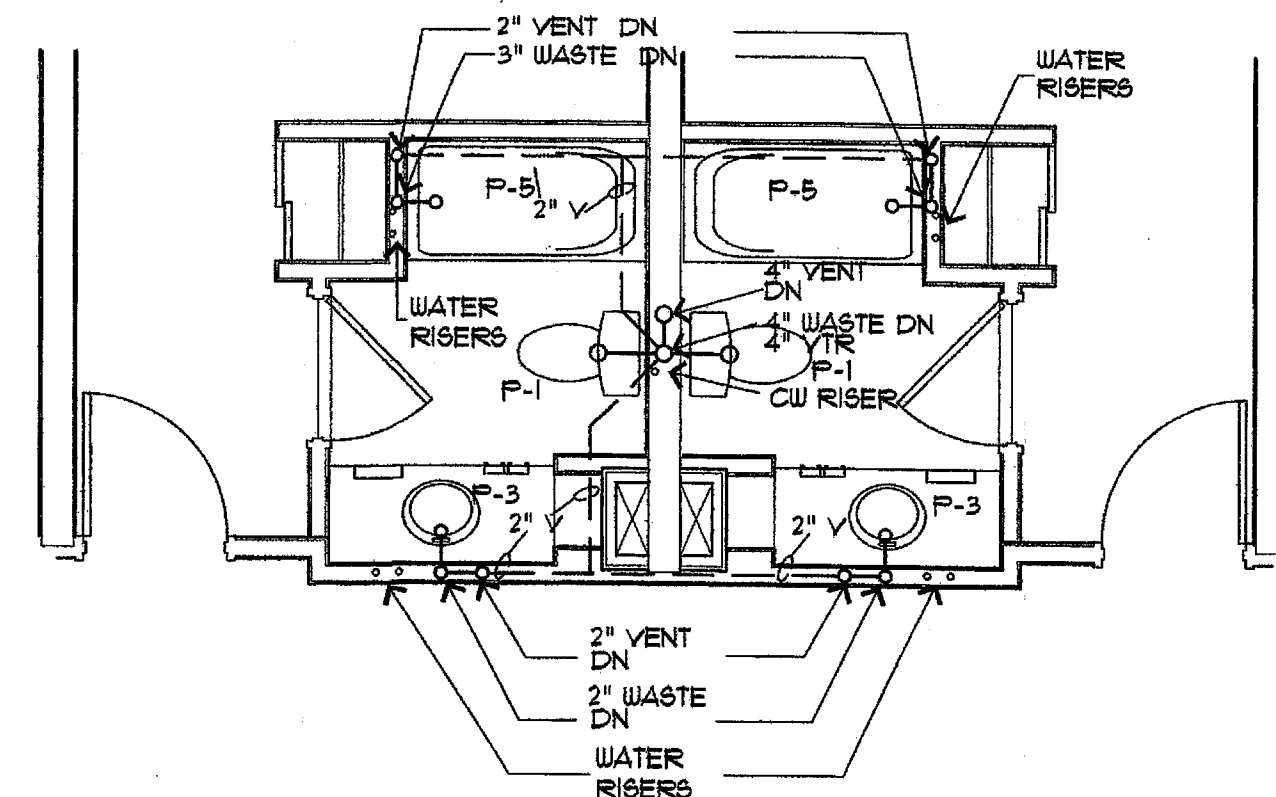
10 3rd FLR. BACK TO BACK RMS. 1/4" = 1'-0" AX-X-X
