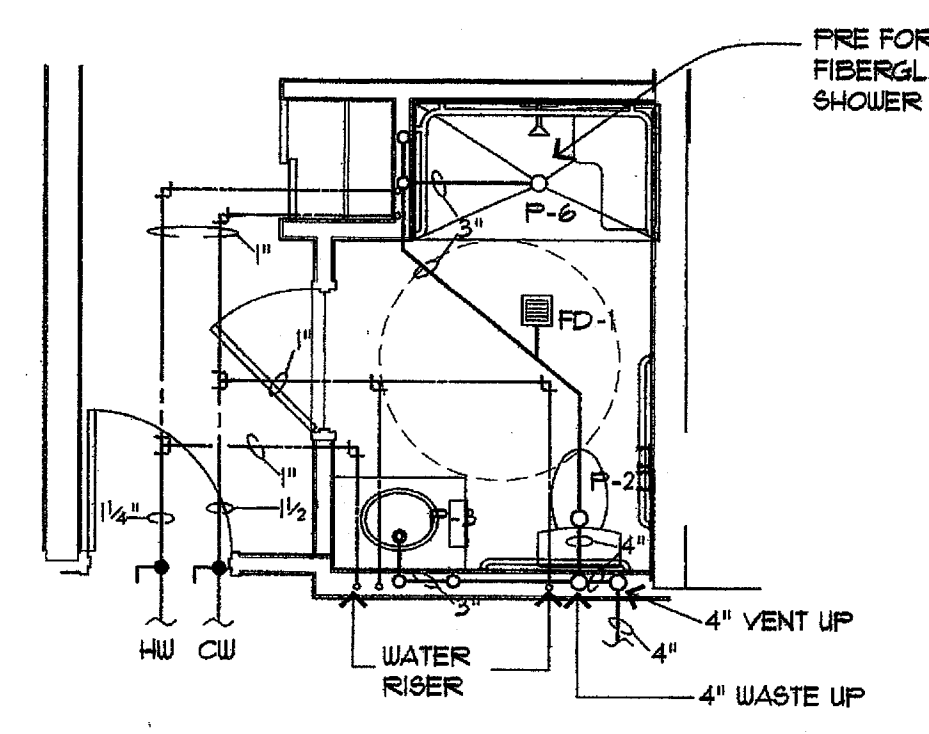
3 GR. FLR. ACCESS. RM 1/4" = 1'-0" AX-X-X
