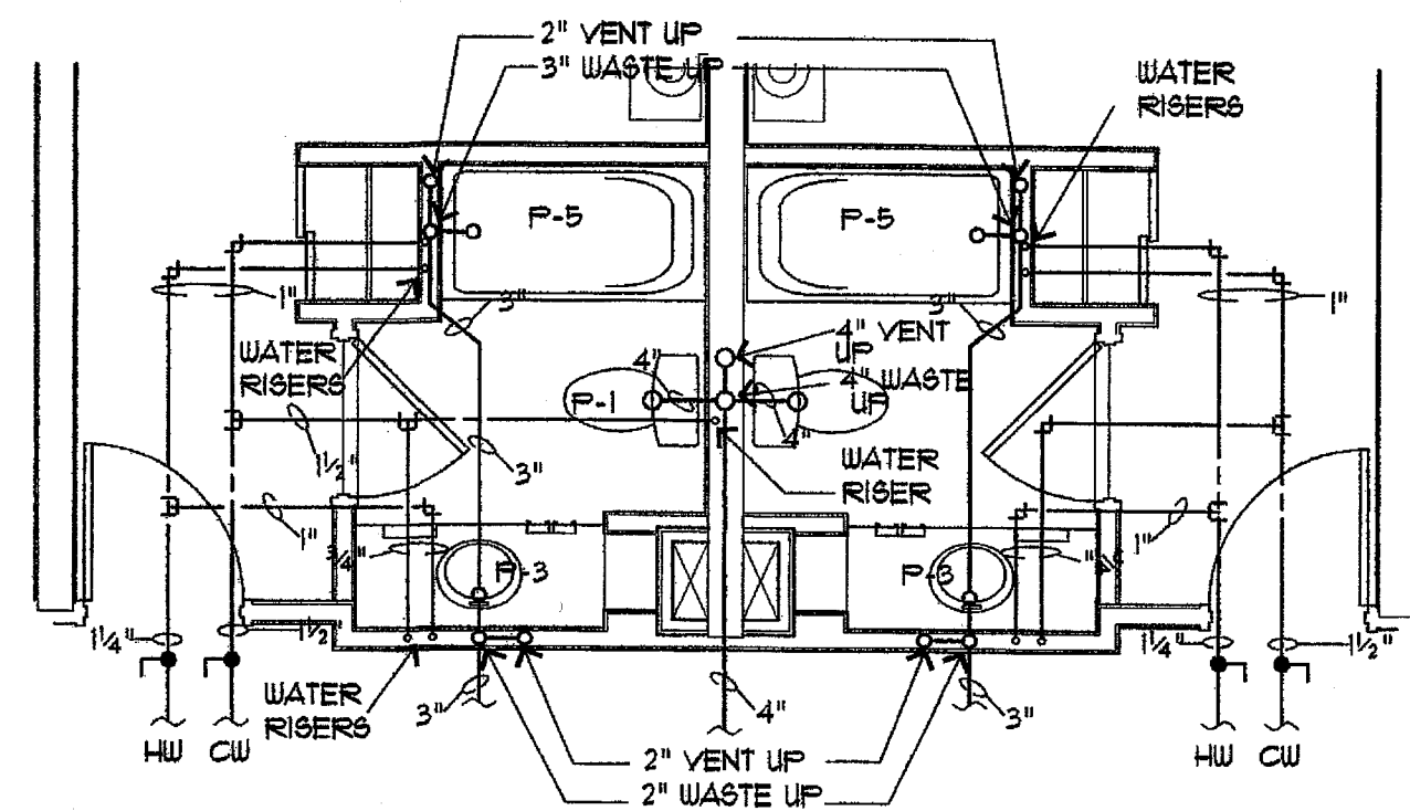
2 GR. FLR. BACK TO BACK RMS. 1/4" = 1'-0" AX-X-X
