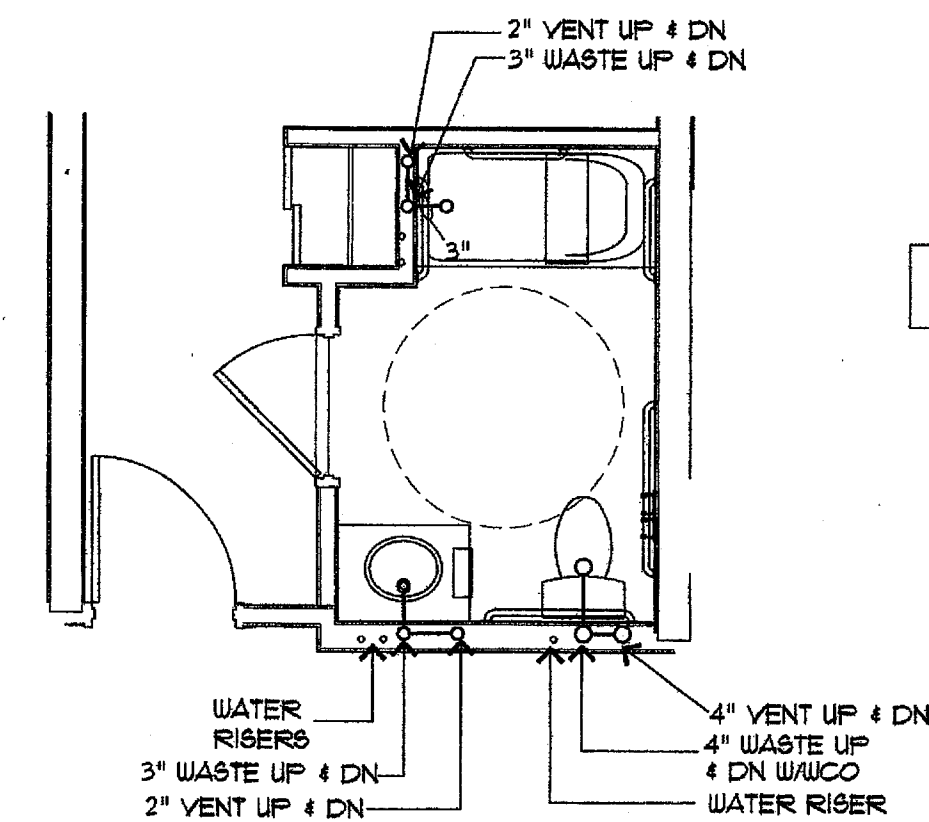
7 TYP. FLR. ACCESS. RM 1/4" = 1'-0" AX-X-X
