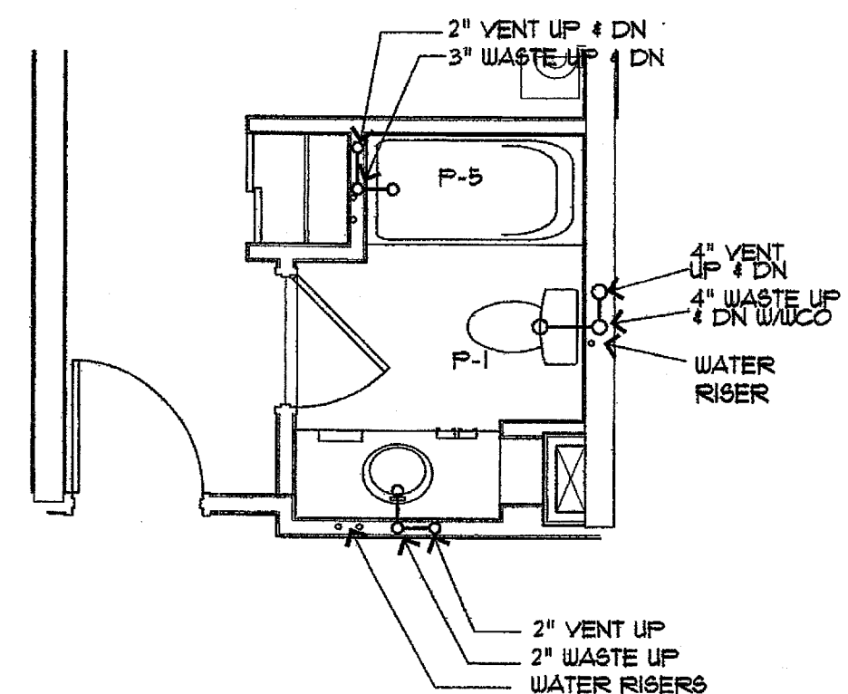
5 TYP. FLR. SINGLE RM 1/4" = 1'-0" AX-X-X
