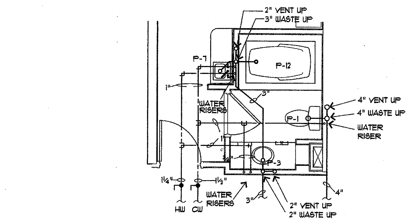
4 GR. FLR. WHIRLPOOL SUITE 1/4" = 1'-0" AX-X-X
