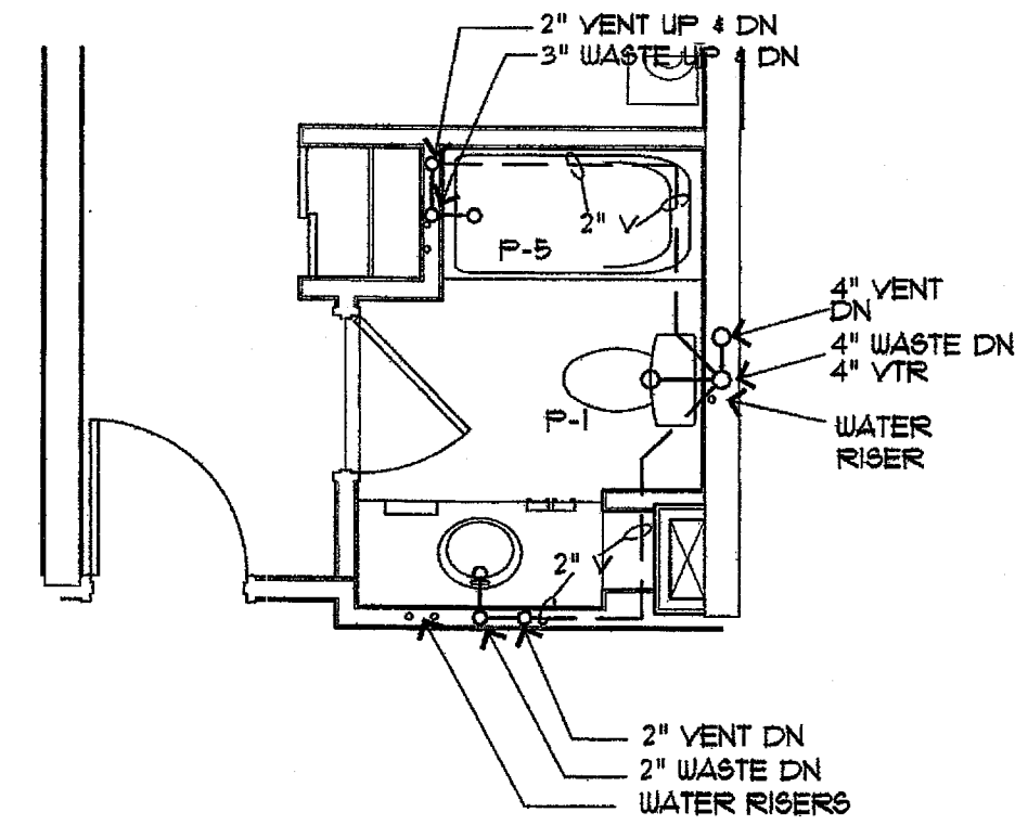
9 3rd FLR. SINGLE RM 1/4" = 1'-0" AX-X-X
