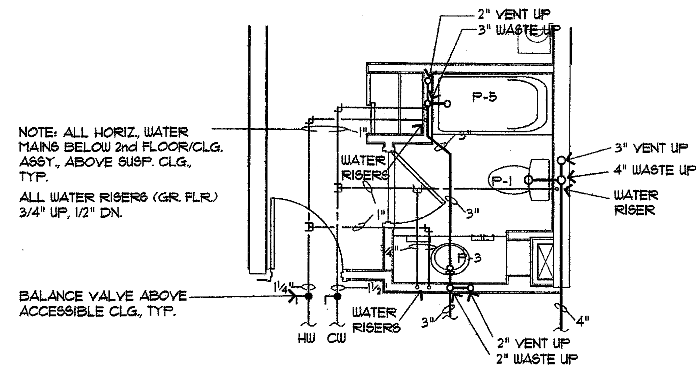
1 GR. FLR. SINGLE RM 1/4" = 1'-0" AX-X-X
