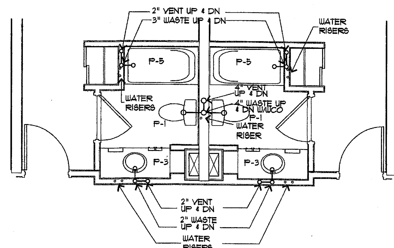
6 TYP. FLR. BACK TO BACK RMS. 1/4" = 1'-0" AX-X-X
