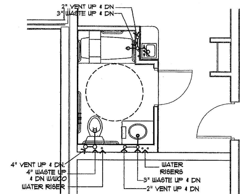
12 ACCESS. SUITE 1/4" = 1'-0" AX-X-X
