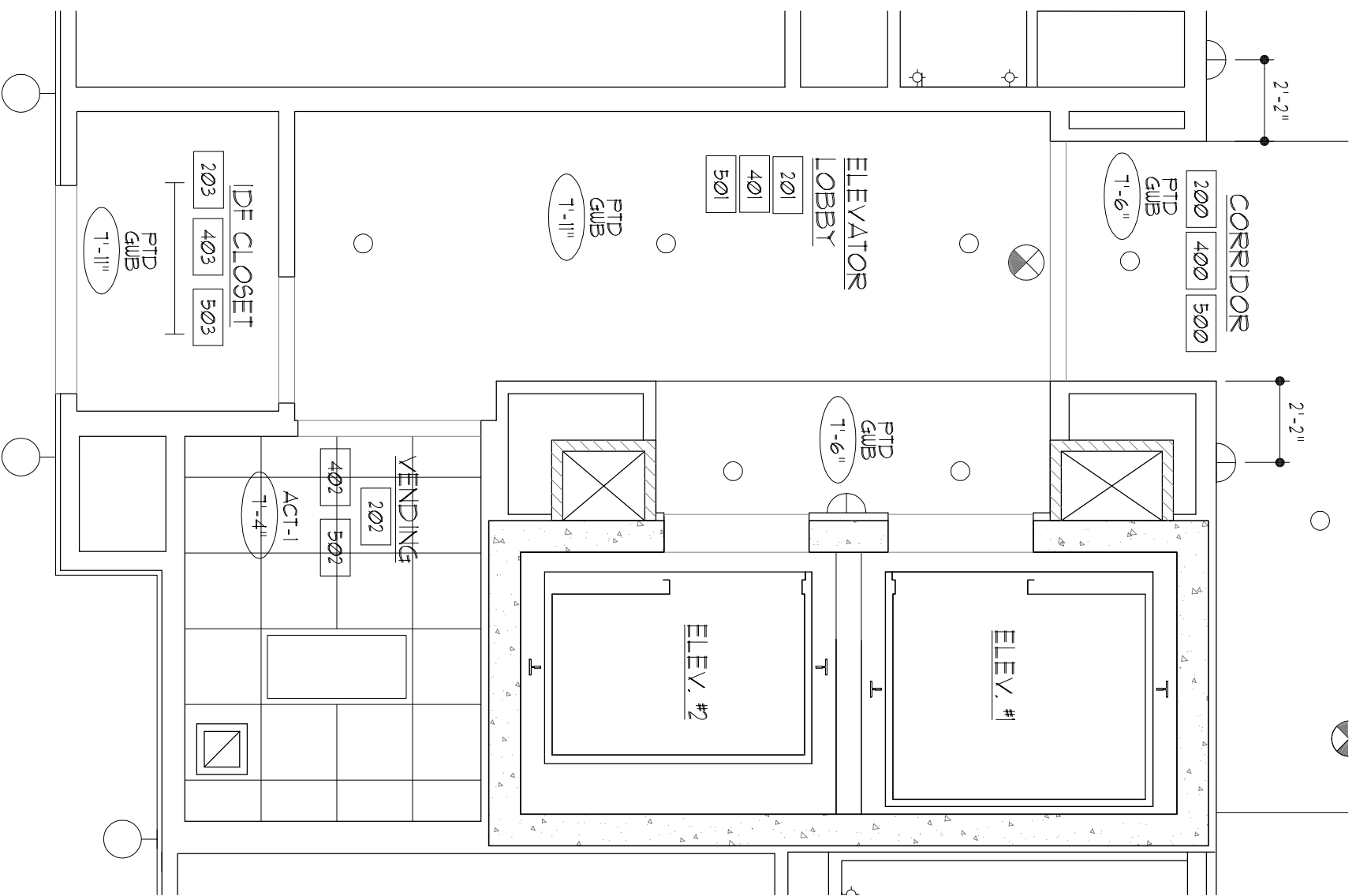
1 ELEVATOR LOBBY @ 2ND, 4TH, AND 5TH FLOORS A4.10 SCALE: 1/4" = 1'-0"
