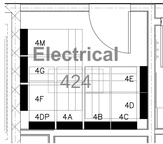
2 E204 ENLARGED ELECTRICAL ROOM SCALE: 1/4" = 1'-0"
