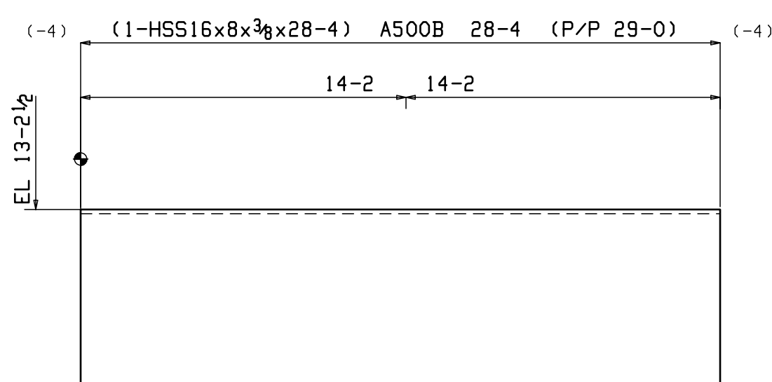
ONE BEAM 4B8
