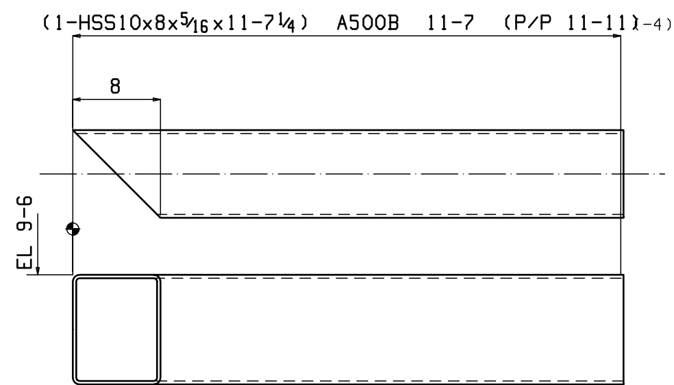
ONE BEAM 12B2
