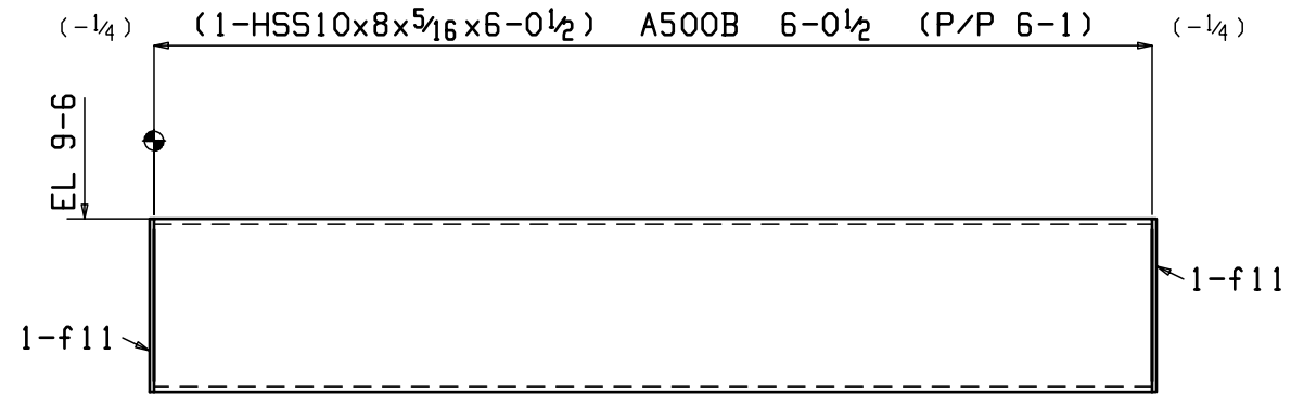
ONE BEAM 10B3
