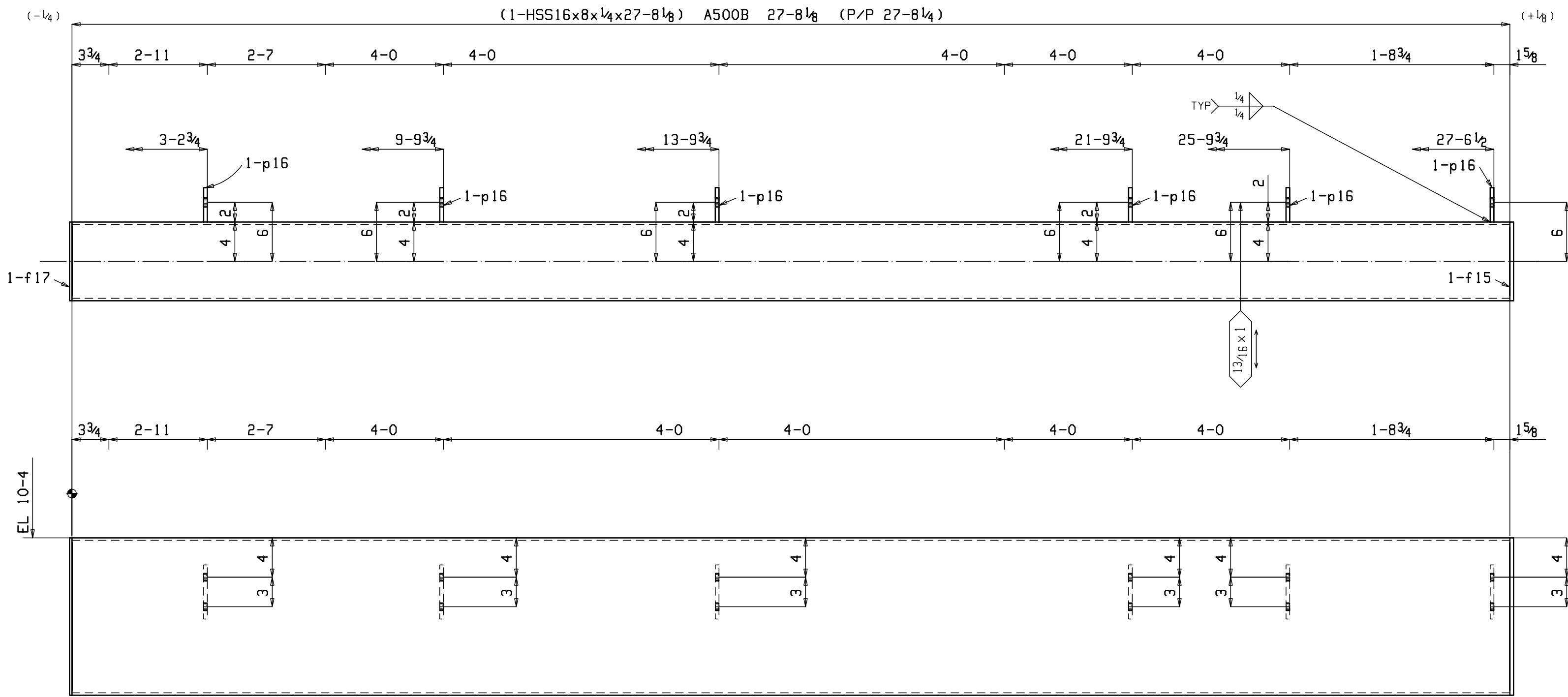
ONE BEAM 3B5
