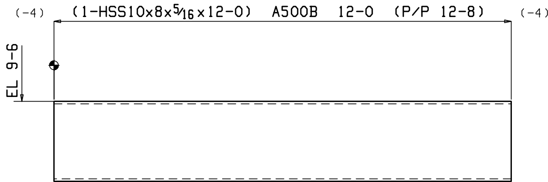
4 BEAMS 10B1
