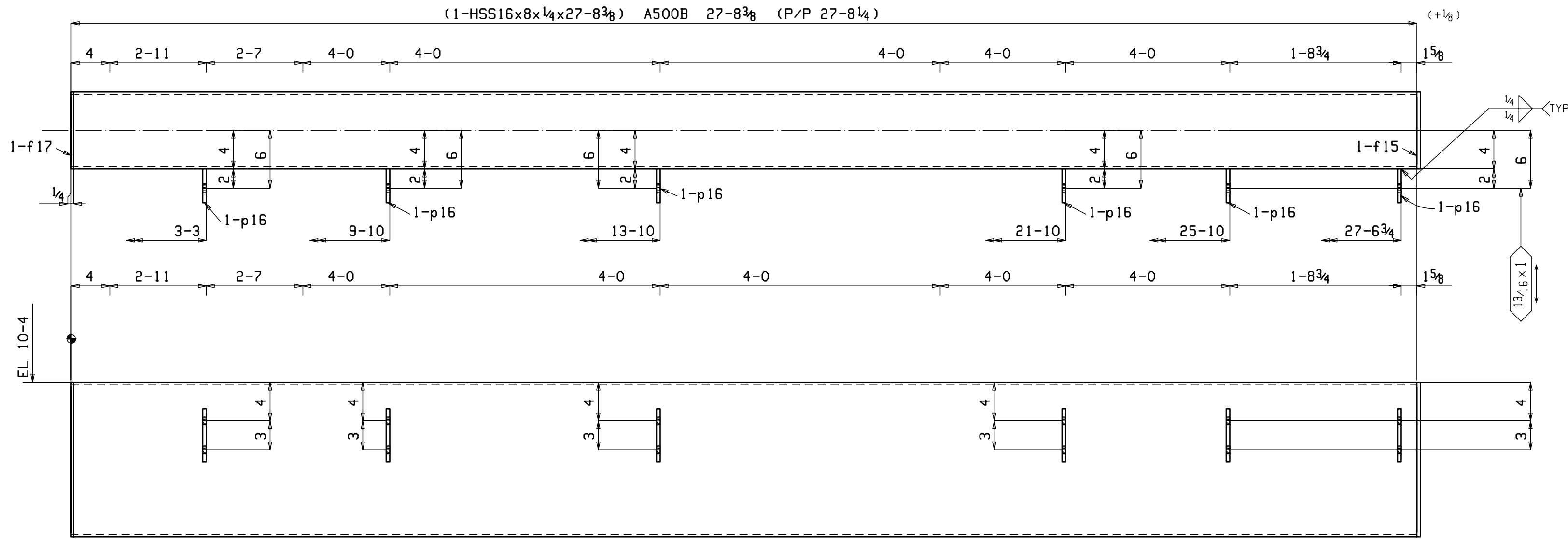
ONE BEAM 3B1
