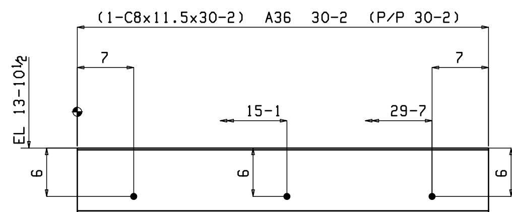
4 BEAMS 11B3
