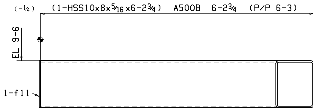
ONE BEAM 3B6
