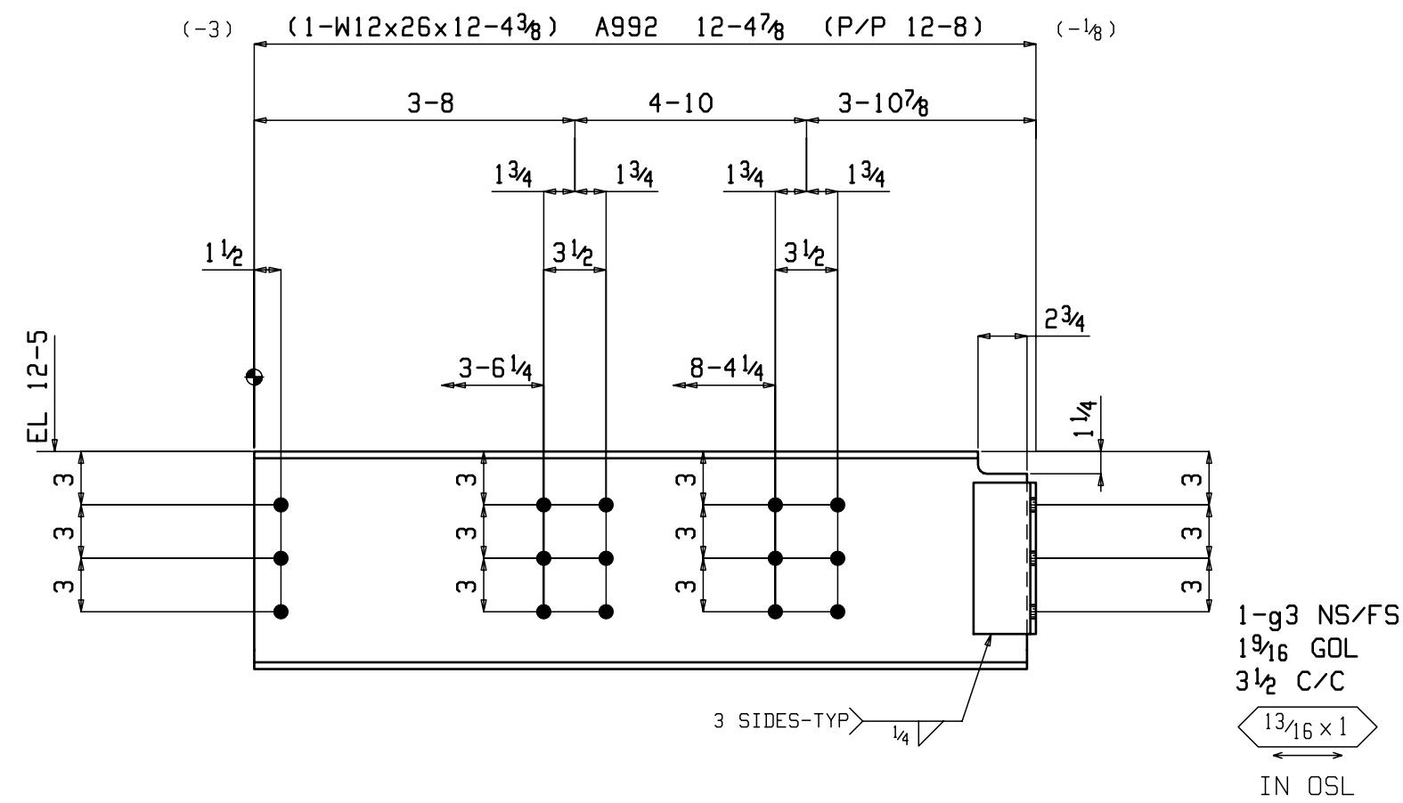
ONE BEAM 8B4
