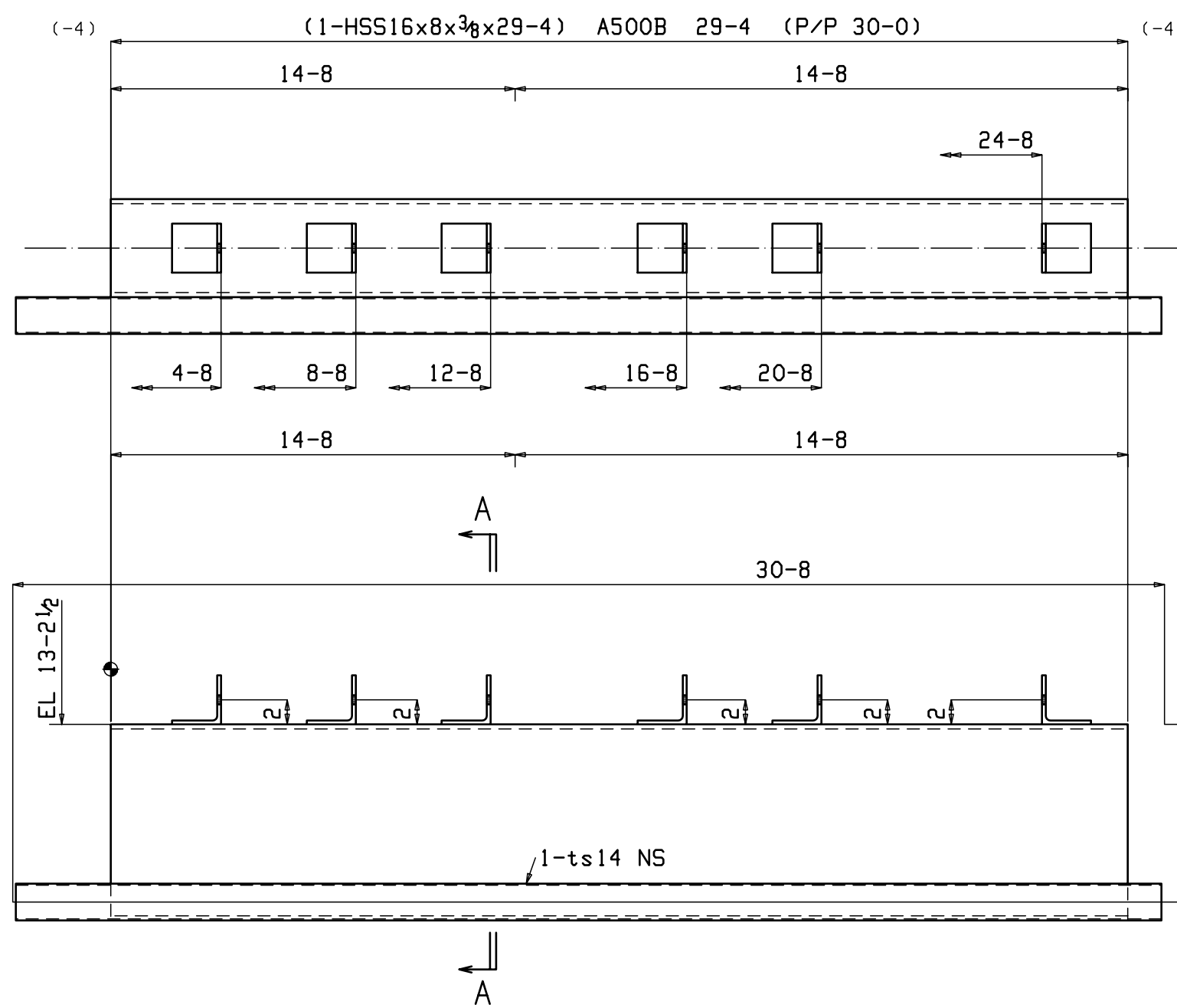
ONE BEAM 12B7
