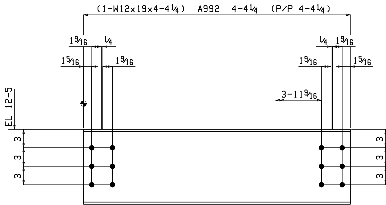
ONE BEAM 3B2
