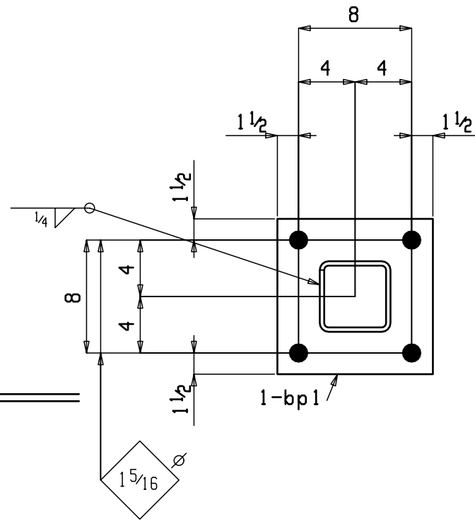
ONE COLUMN 21C2
