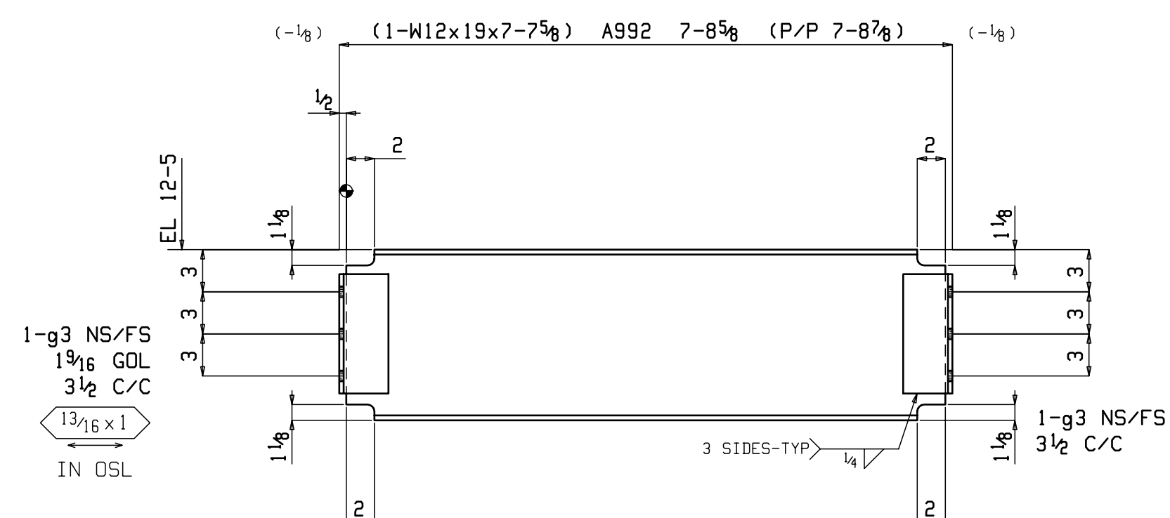
3 BEAMS 4B7
