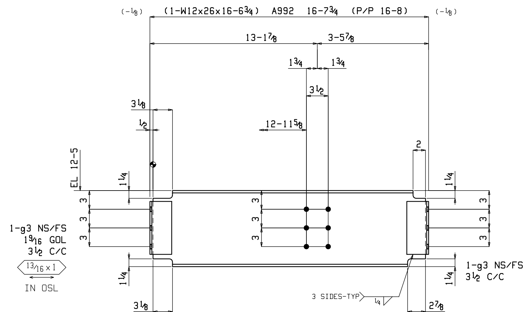
ONE BEAM 8B9
