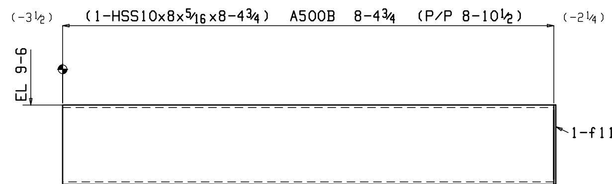
2 BEAMS 11B4
