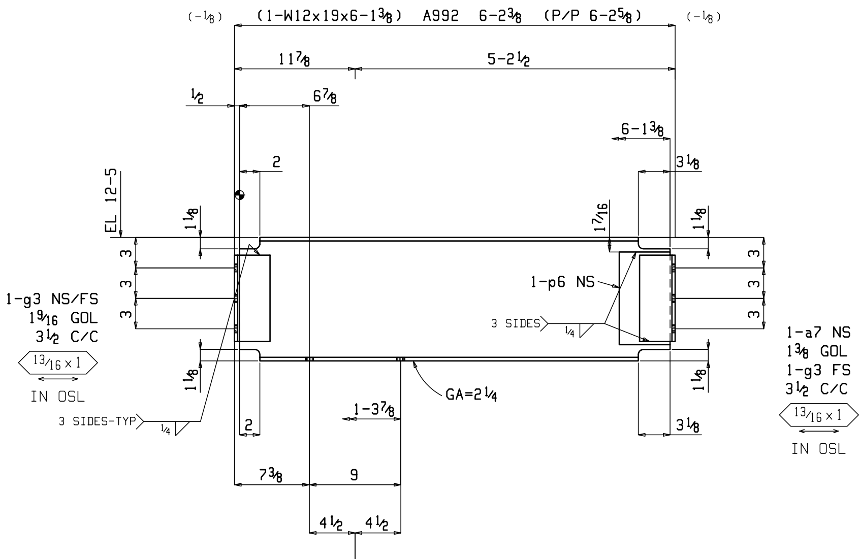
ONE BEAM 10B8
