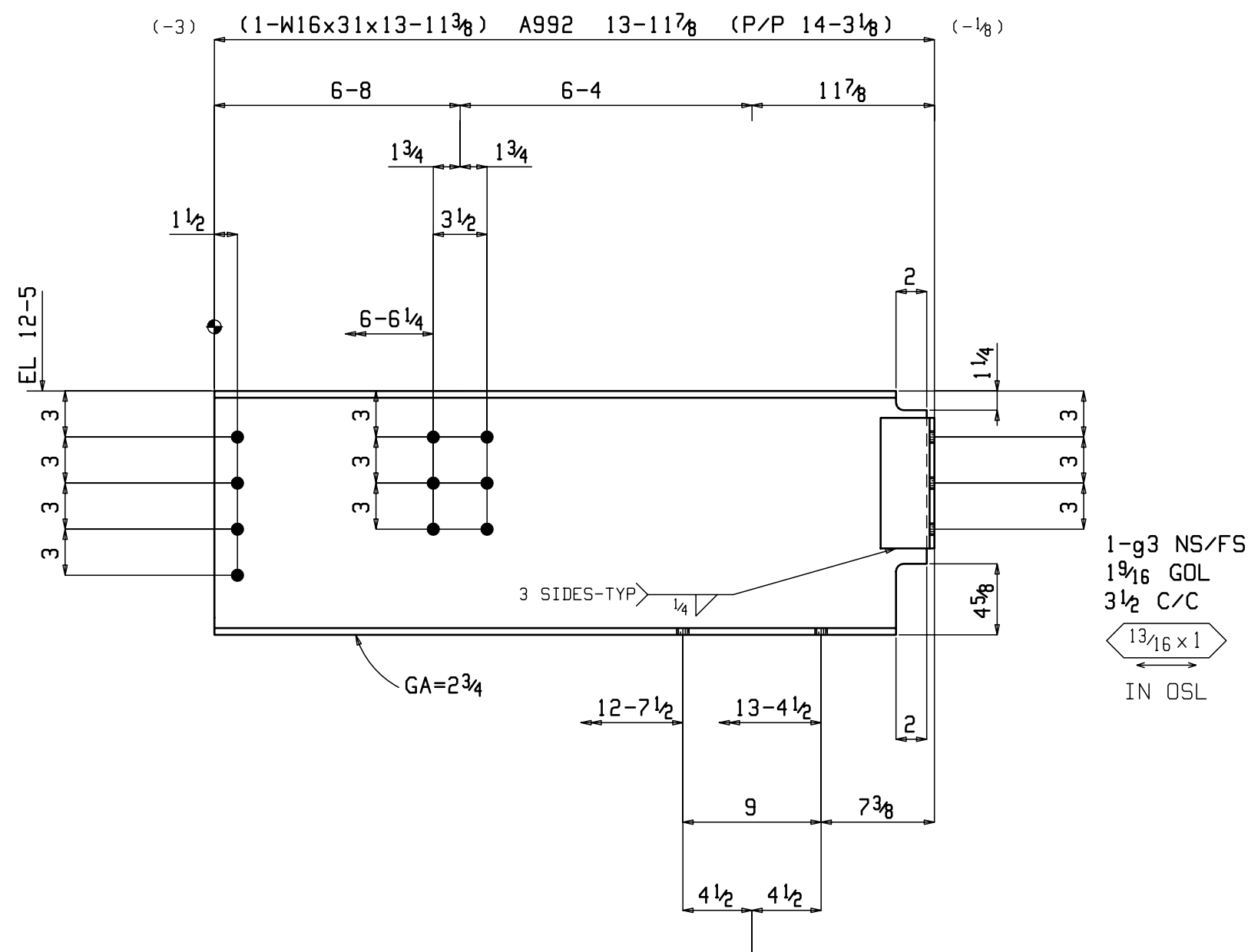
ONE BEAM 8B1
