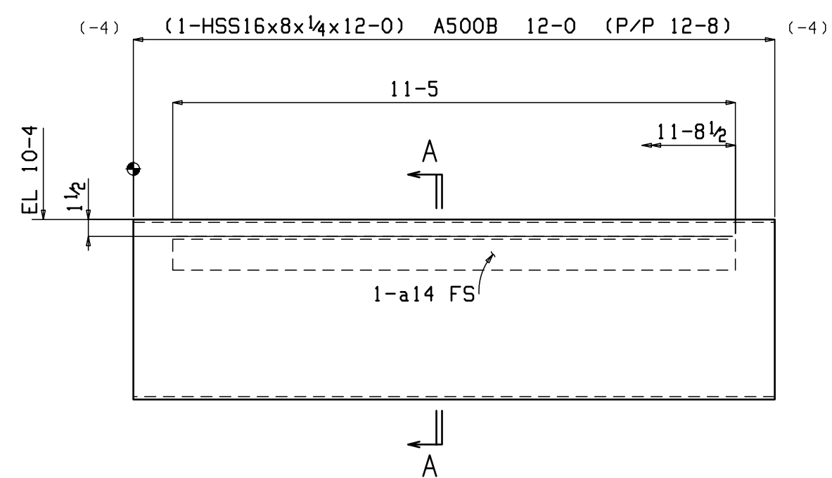
ONE BEAM 11B6
