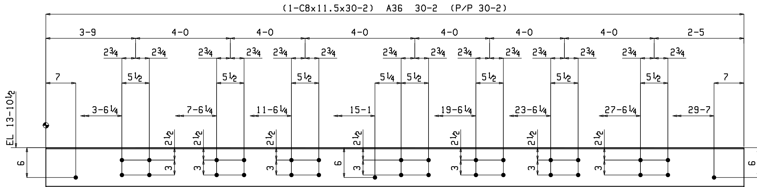
ONE BEAM 10B5
