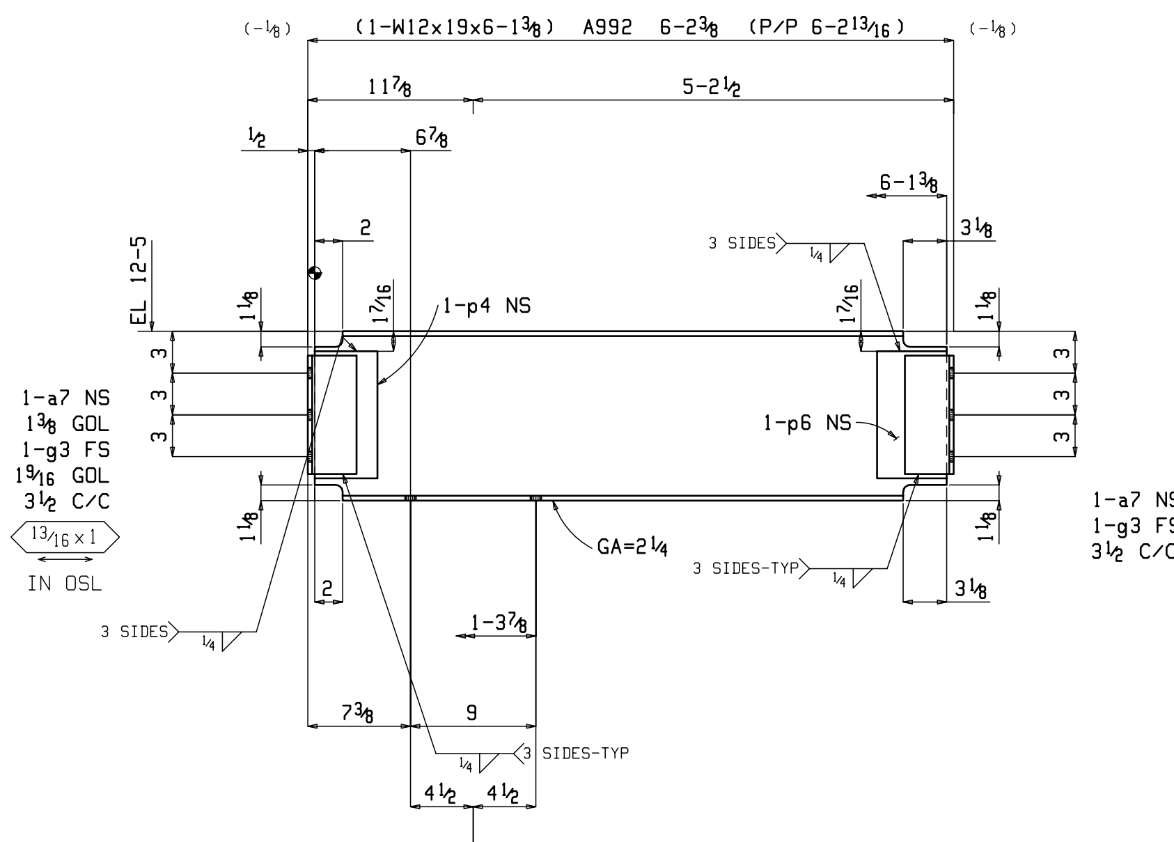
ONE BEAM 12B3
