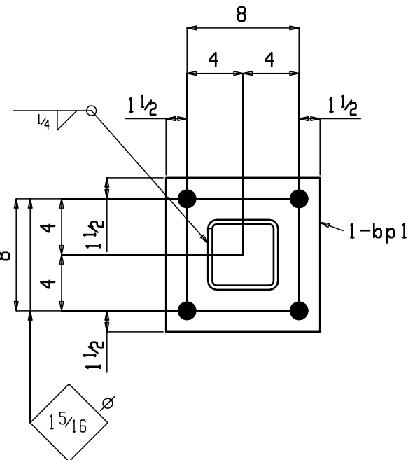
ONE COLUMN 18C1
