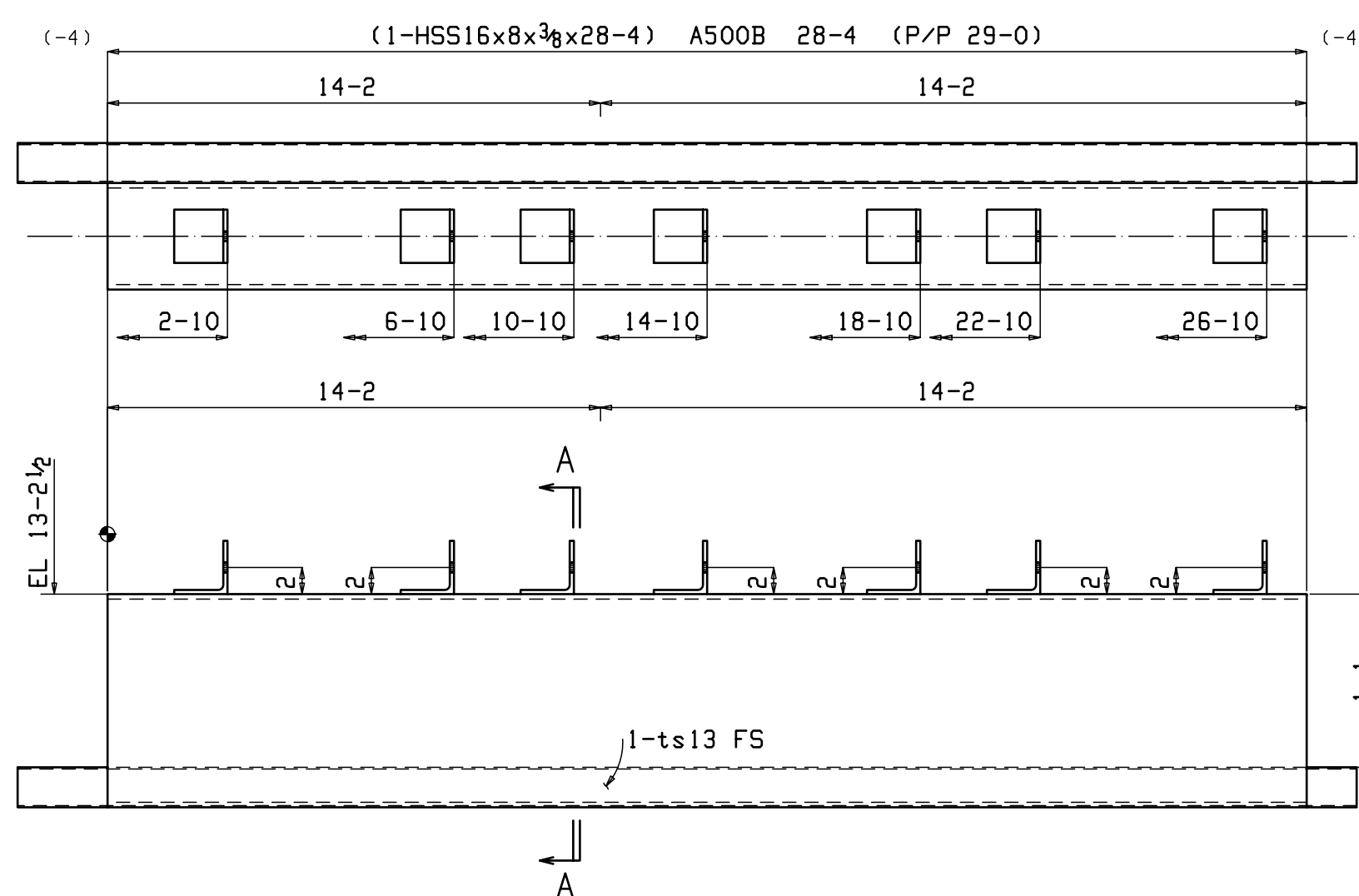
ONE BEAM 4B6
