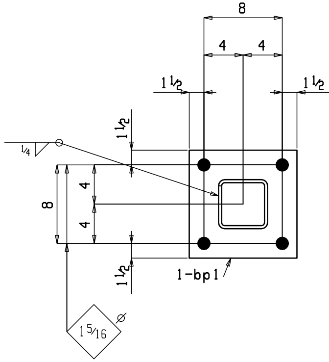
ONE COLUMN 21C1
