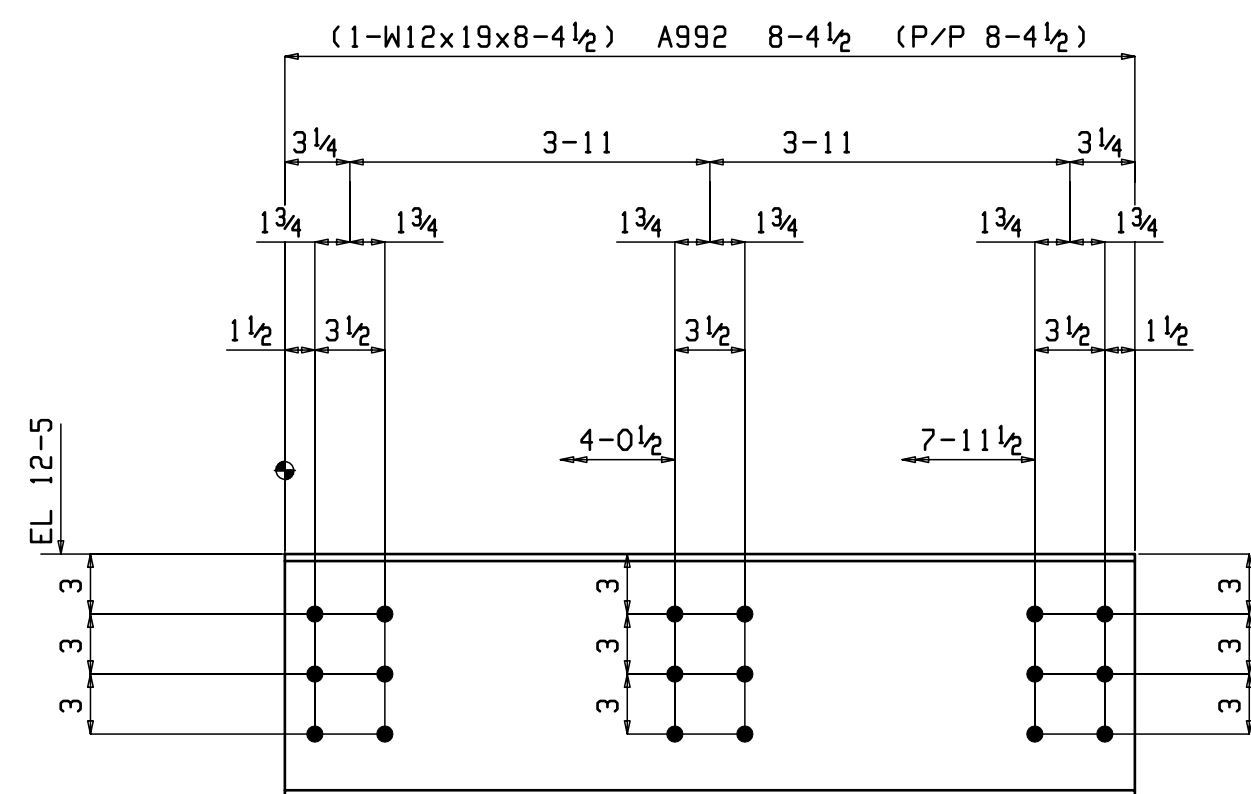
ONE BEAM 8B7
