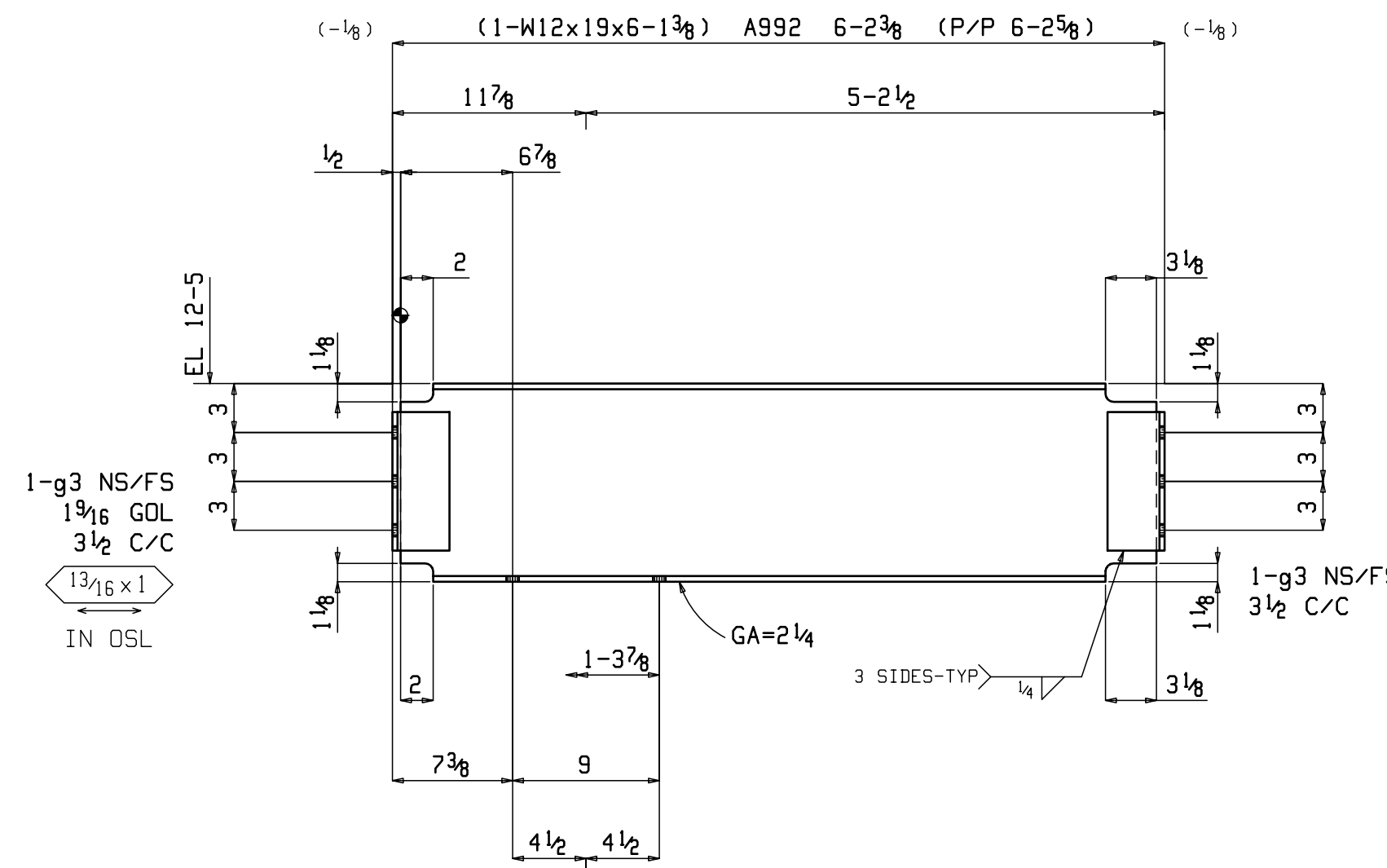
ONE BEAM 11B5
