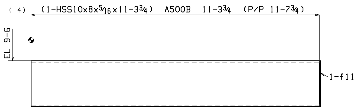
ONE BEAM 12B1
