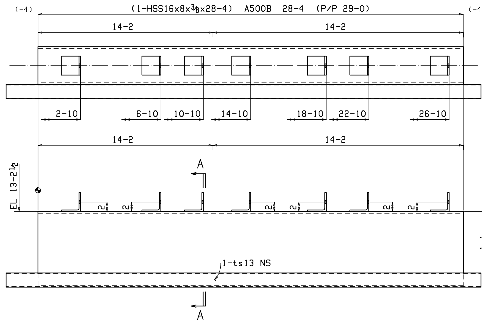
ONE BEAM 11B2
