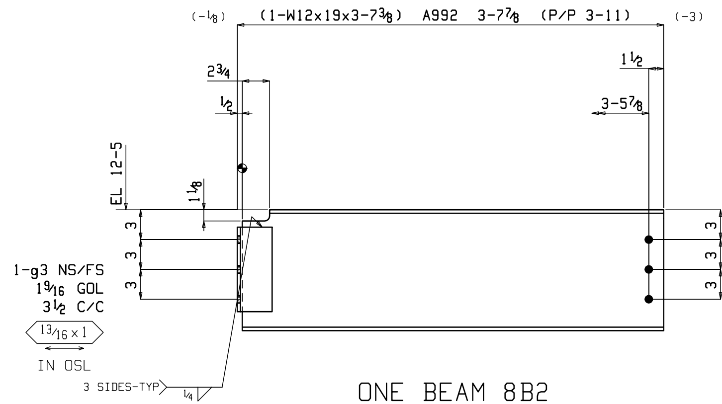
ONE BEAM 8B2
