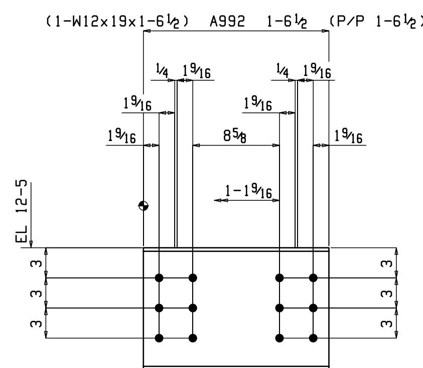
ONE BEAM 4B2
