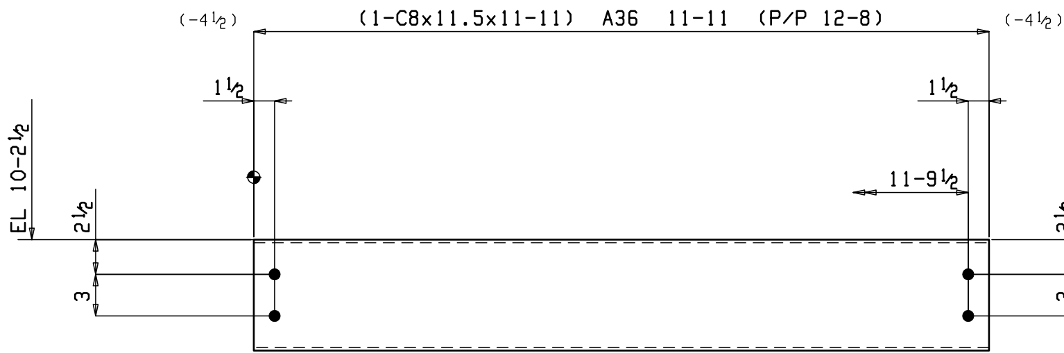
5 BEAMS 3B3
