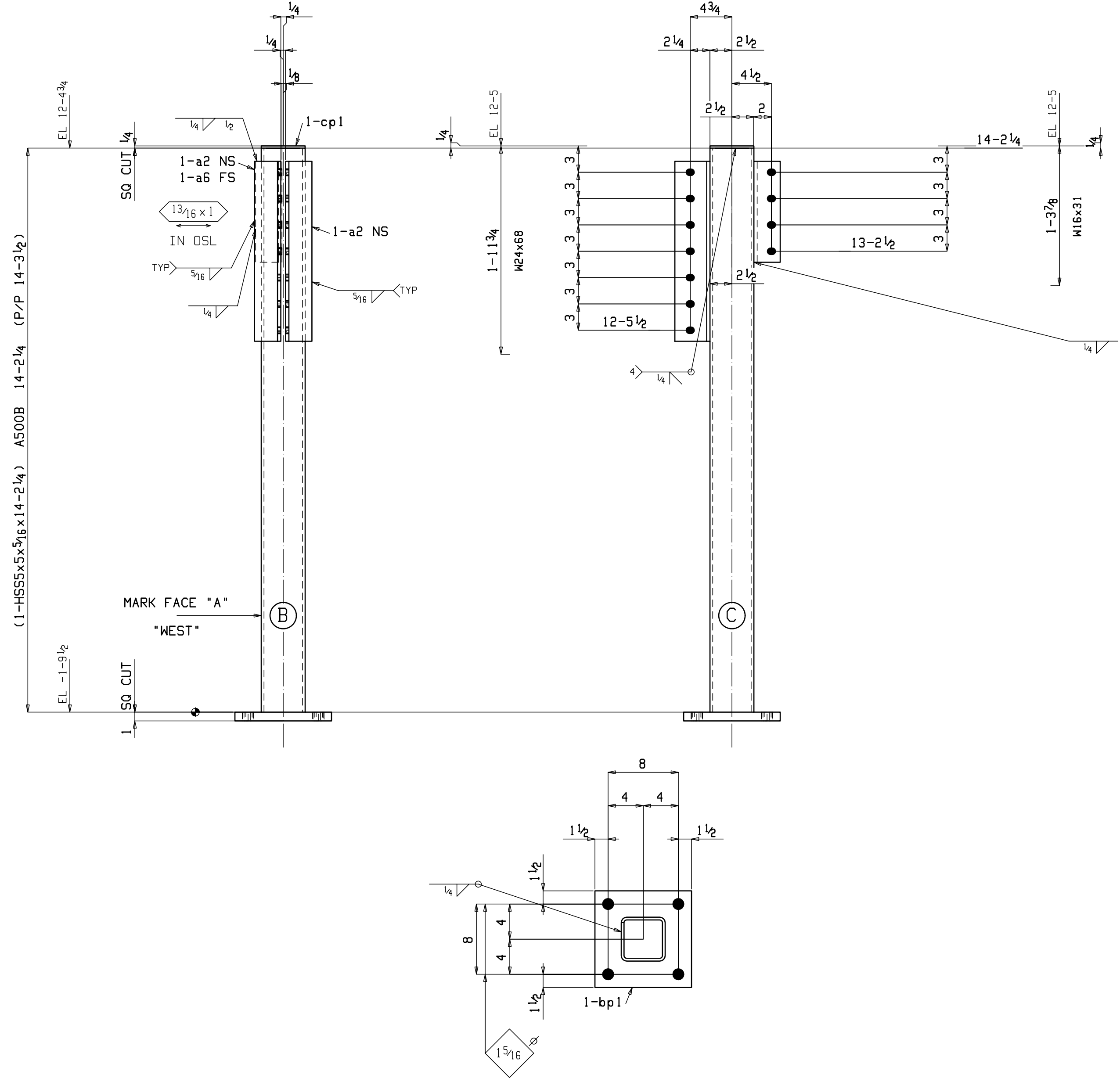
ONE COLUMN 22C1
