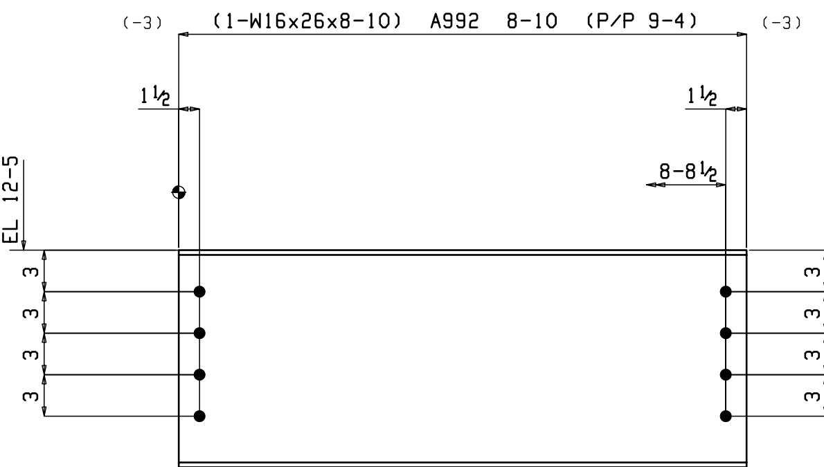
ONE BEAM 10B4
