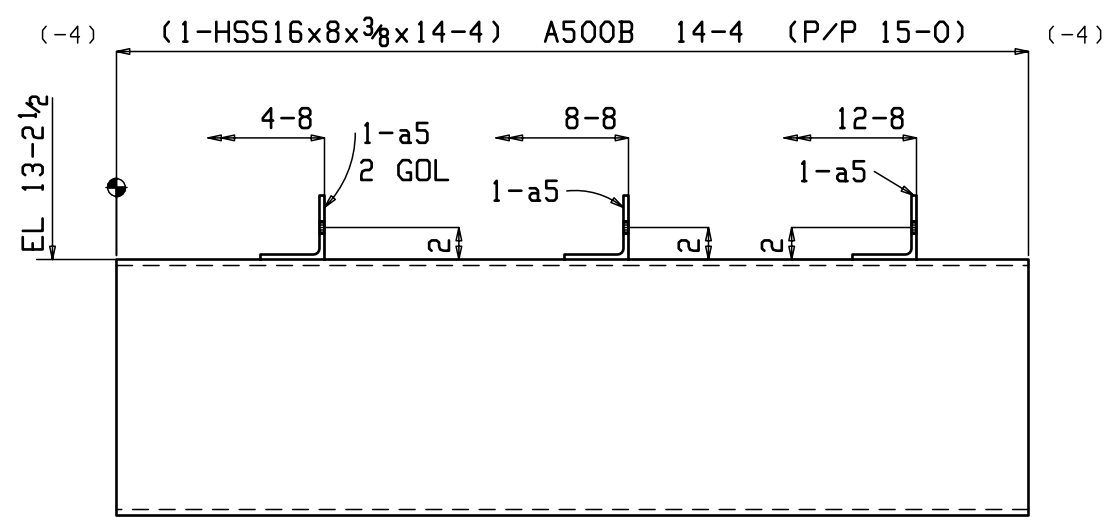
ONE BEAM 12B6
