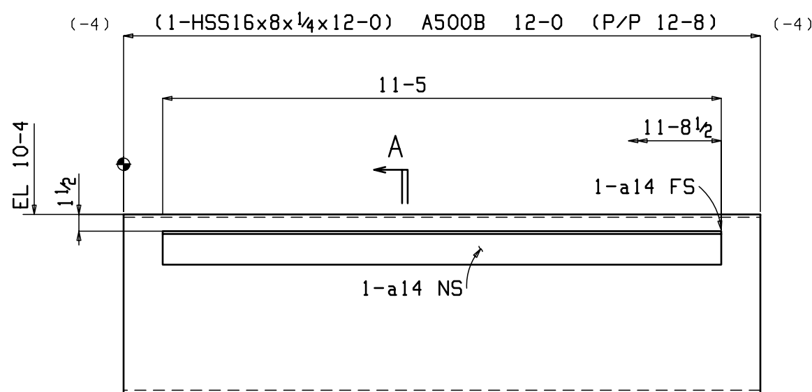
2 BEAMS 12B4
