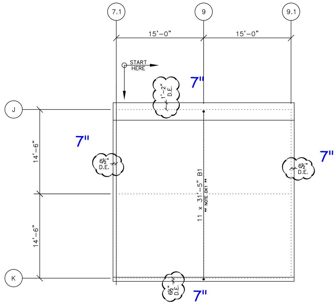
HIGH CANOPY DECKING PLAN SCALE : 1/8"=1'-0" REF. S-202 DATE 7-17-15 SEQUENCE 1, CANOPY - TOA 7, SUMMARY 1, CANOPY
