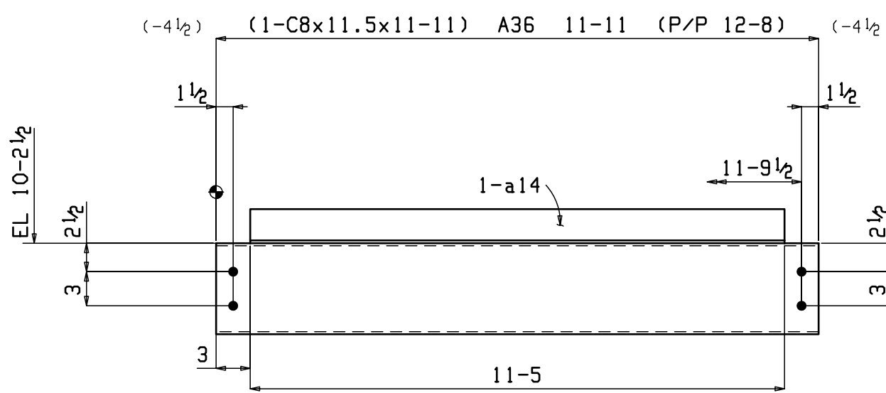
ONE BEAM 12B5
