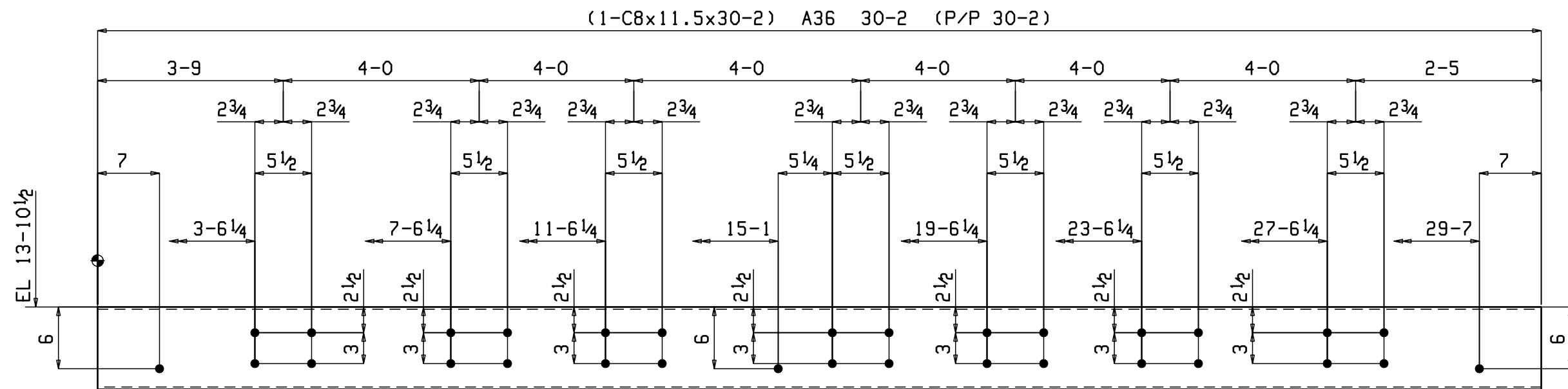
ONE BEAM 10B6
