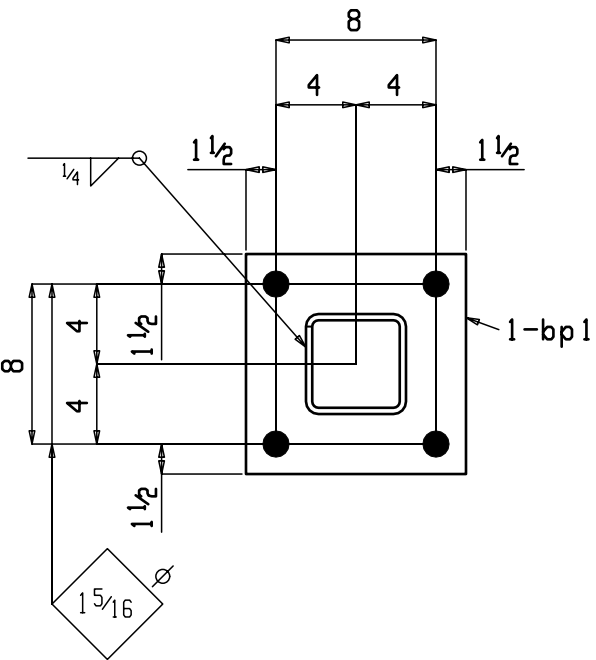
ONE COLUMN 18C2
