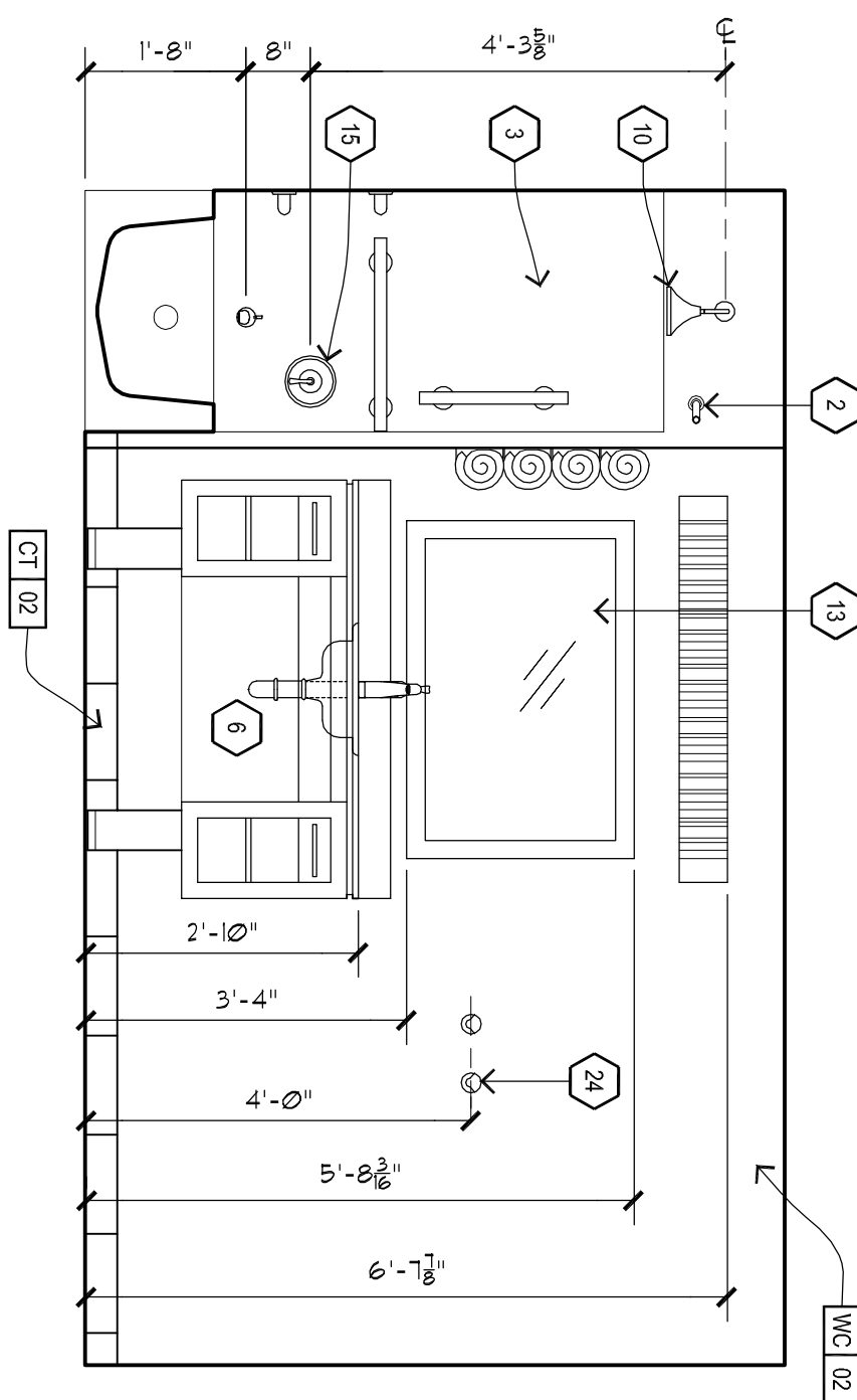
4 INT. ELEV. - ACC. 1 BR. - W/ACC TUB 1/2" = 1'-0"
