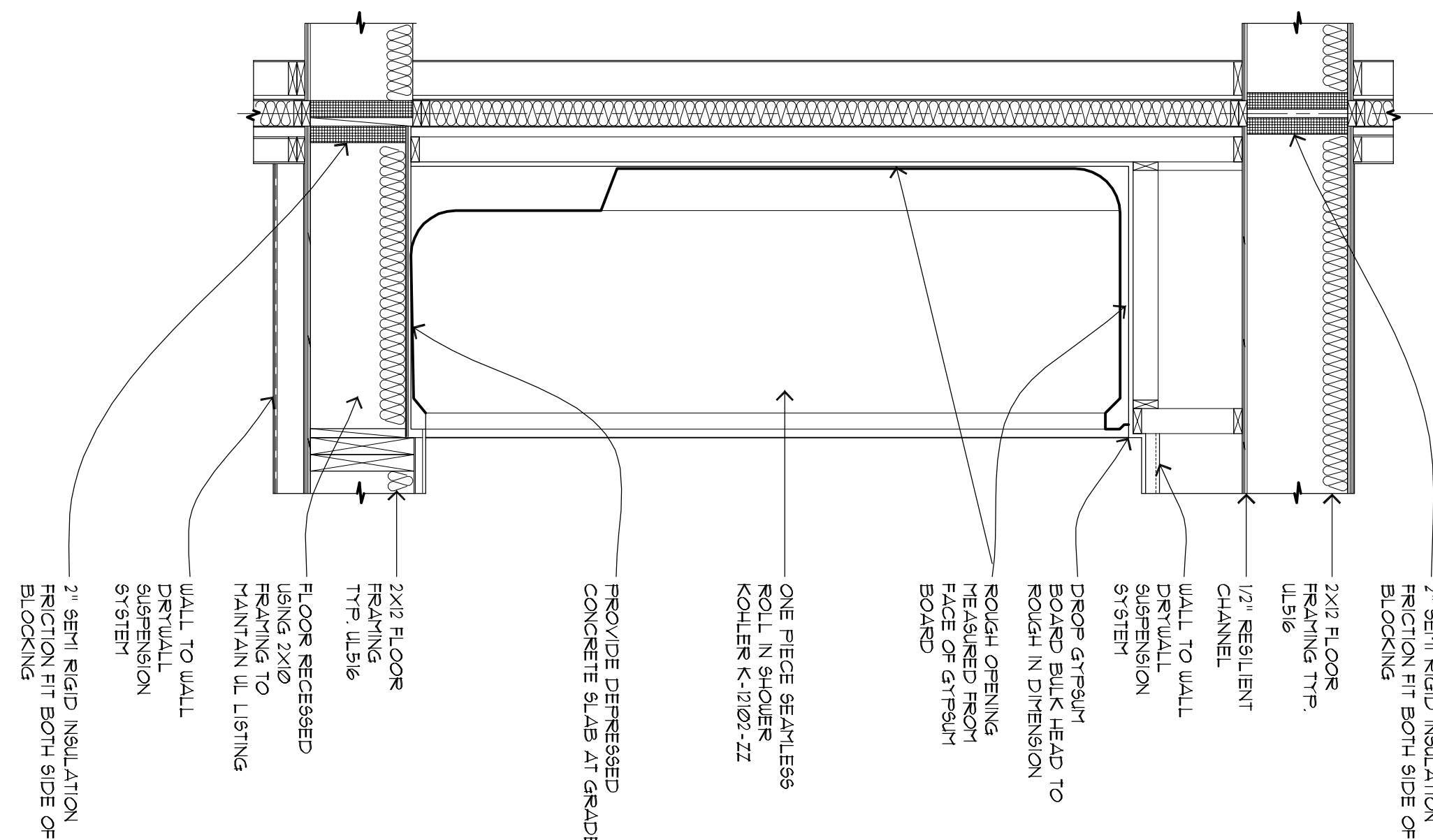
9 DETAIL - ROLL IN SHOWER 3/4" = 1'-0"
