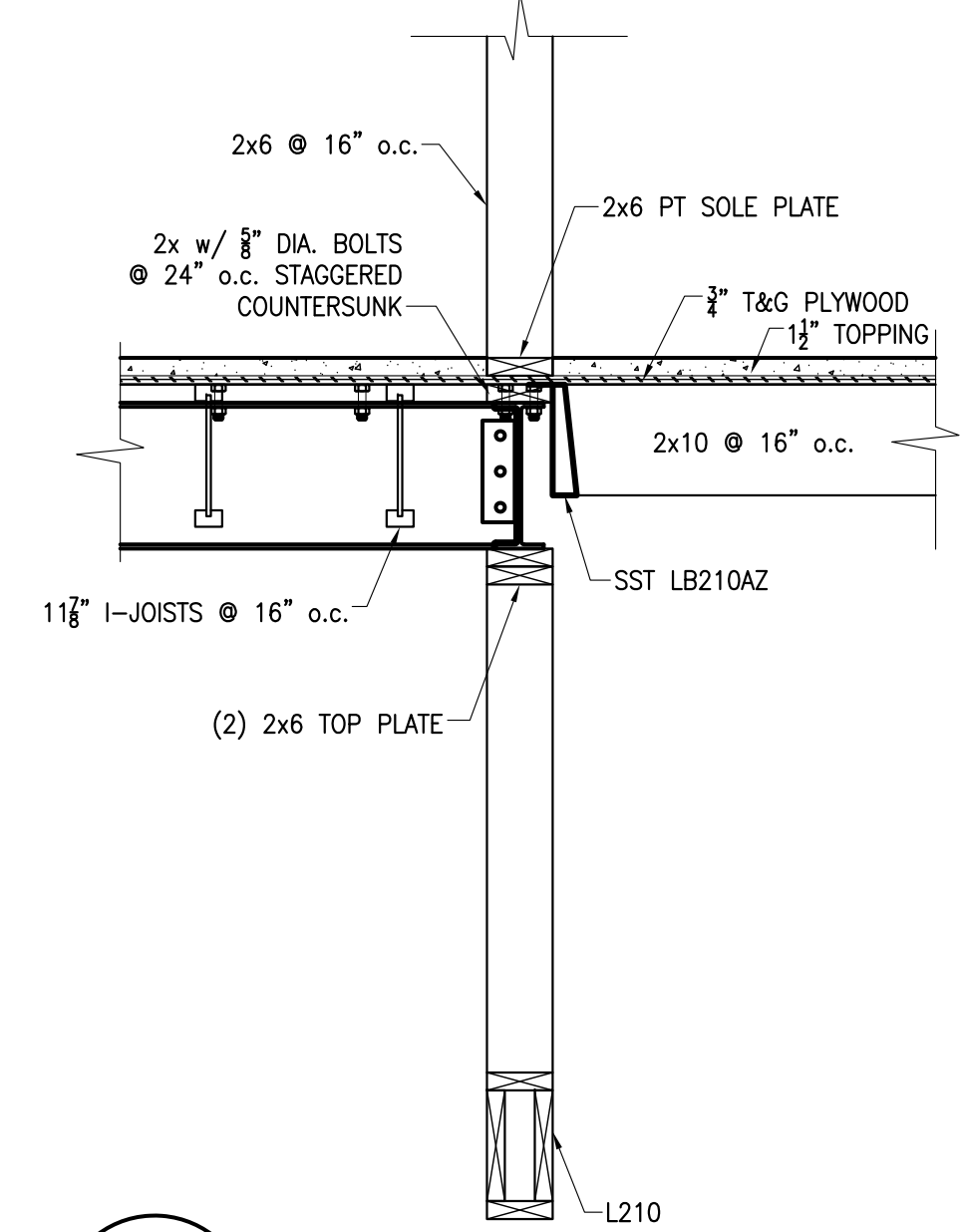
10 SECTION S501 3/4" = 1'-0"
