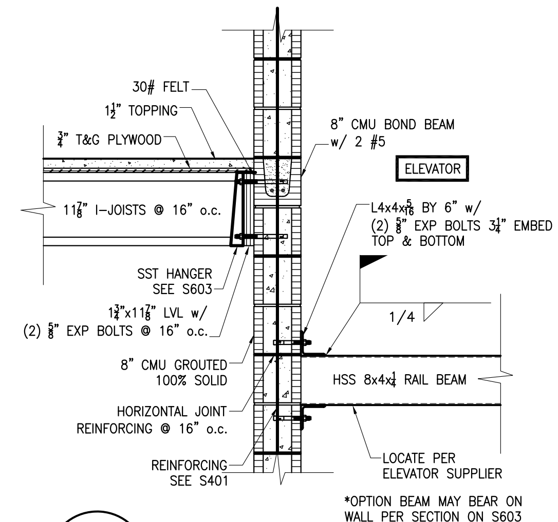
15 SECTION S501 3/4" = 1'-0"
