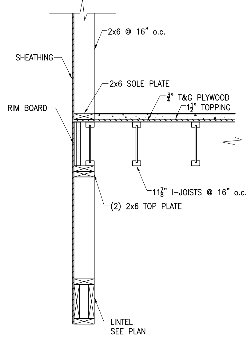
2 SECTION S501 3/4" = 1'-0"
