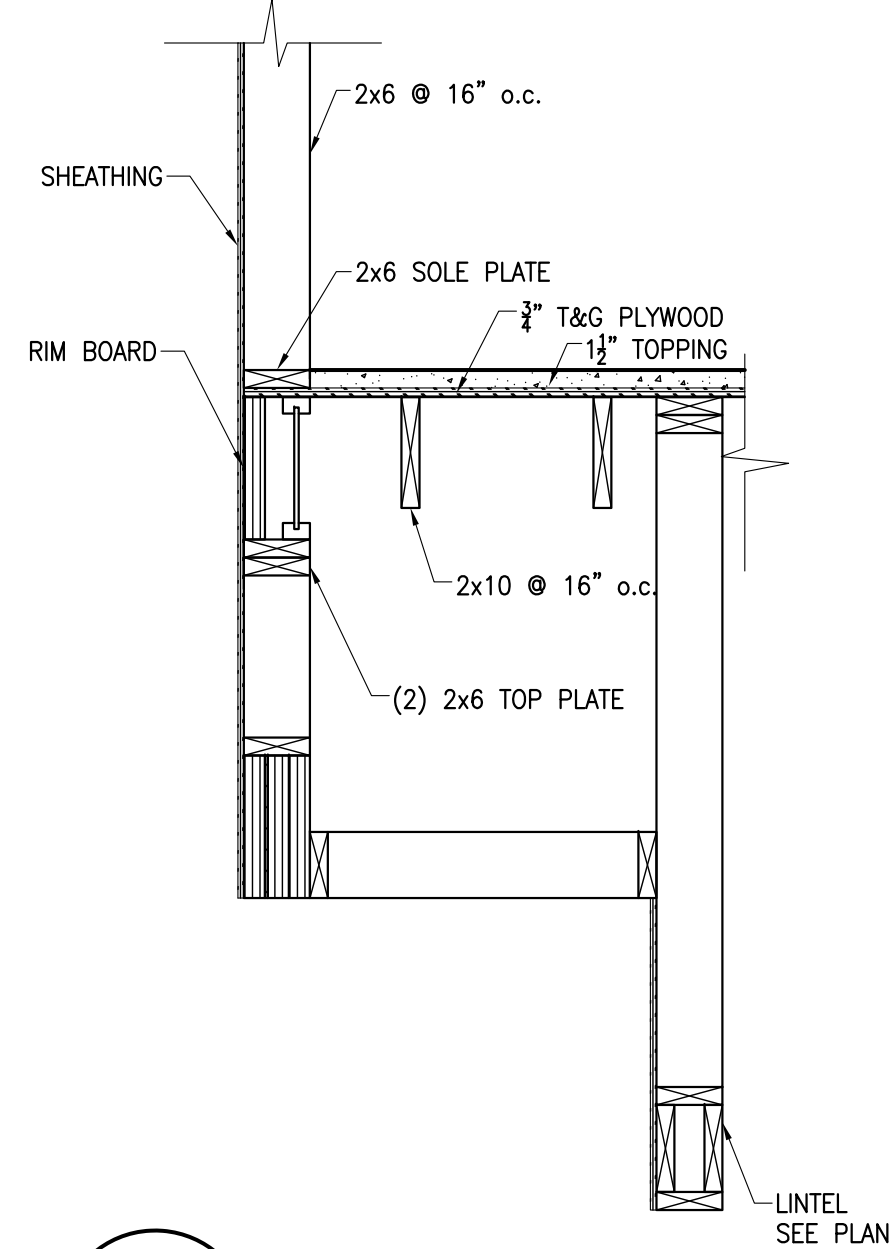
5 SECTION S501 3/4" = 1'-0"
