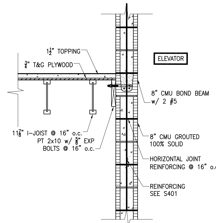
12 SECTION S501 3/4" = 1'-0"
