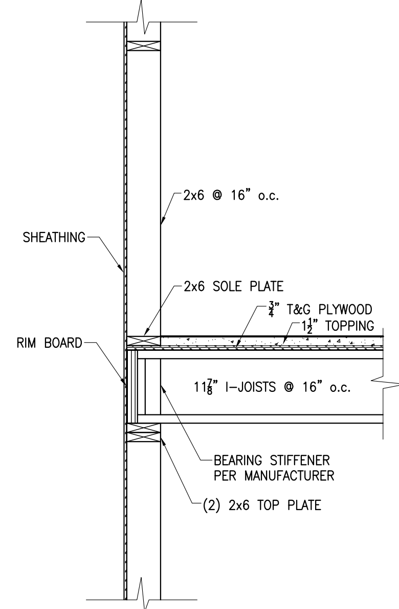
4 SECTION S501 3/4" = 1'-0"
