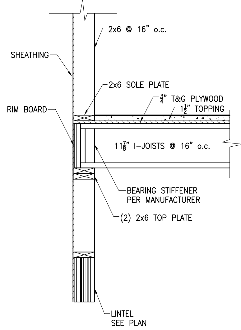
3 SECTION S501 3/4" = 1'-0"
