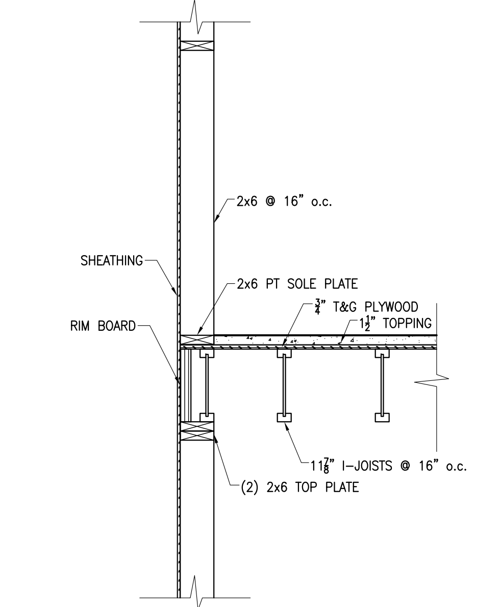
1 SECTION S501 3/4" = 1'-0"
