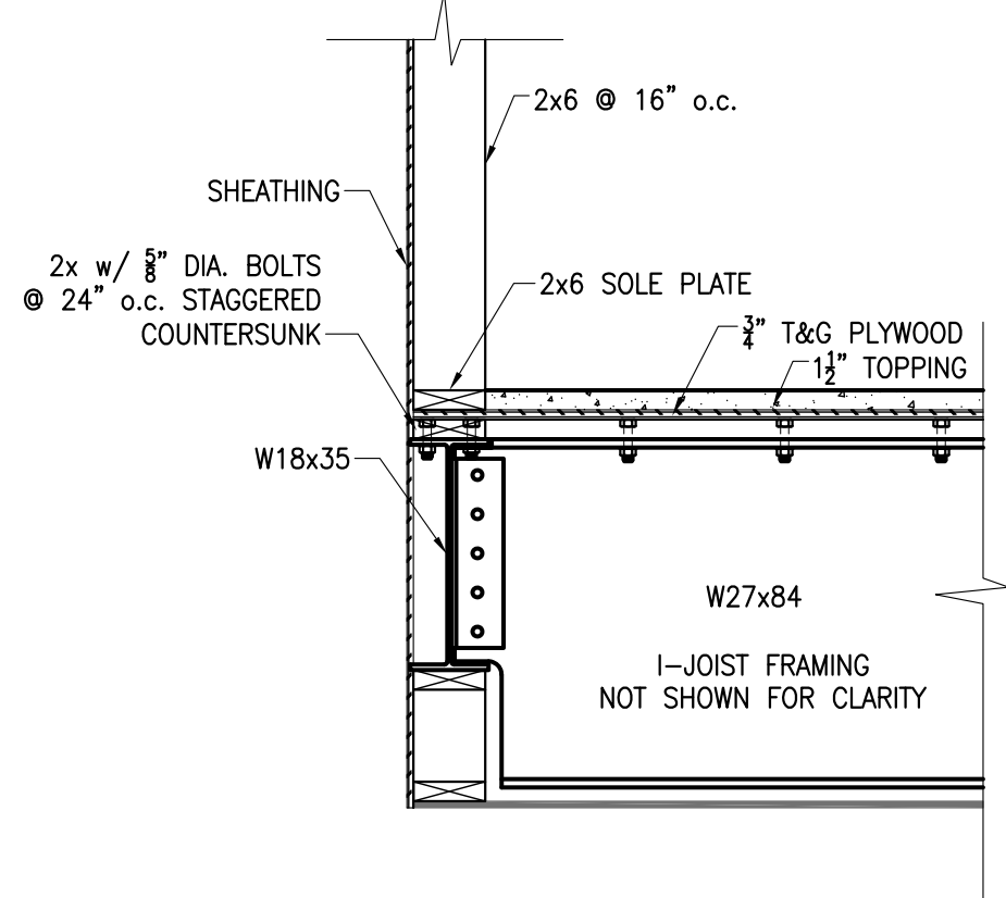
1 SECTION S501 3/4" = 1'-0"
