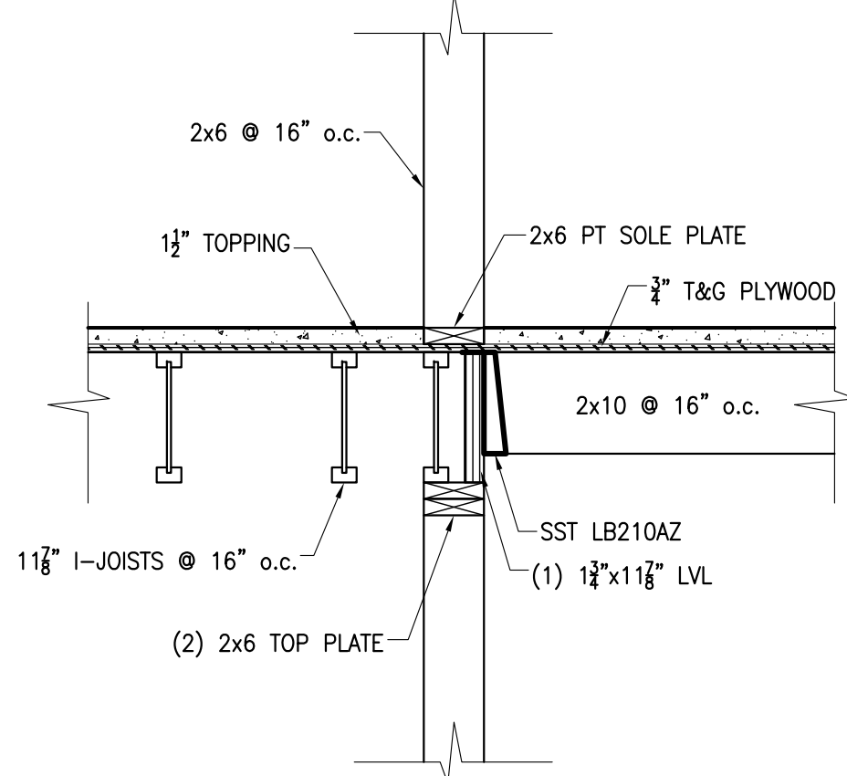
2 SECTION S501 3/4" = 1'-0"
