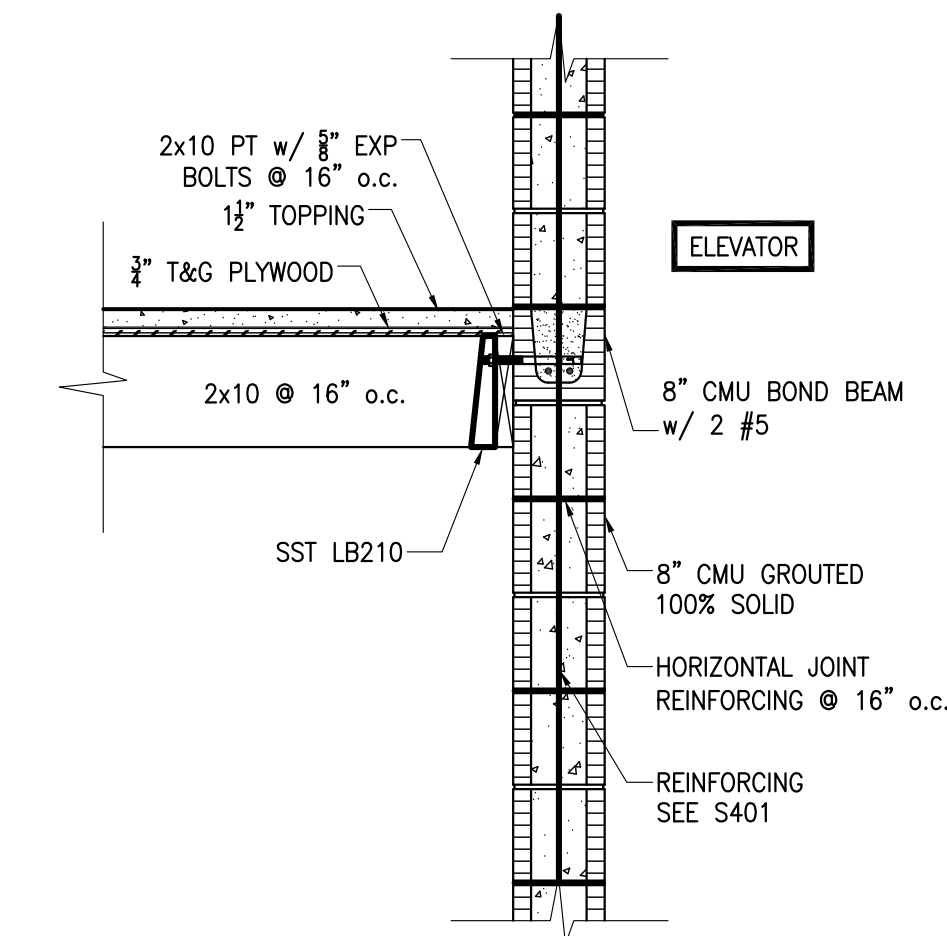
14 SECTION S501 3/4" = 1'-0"
