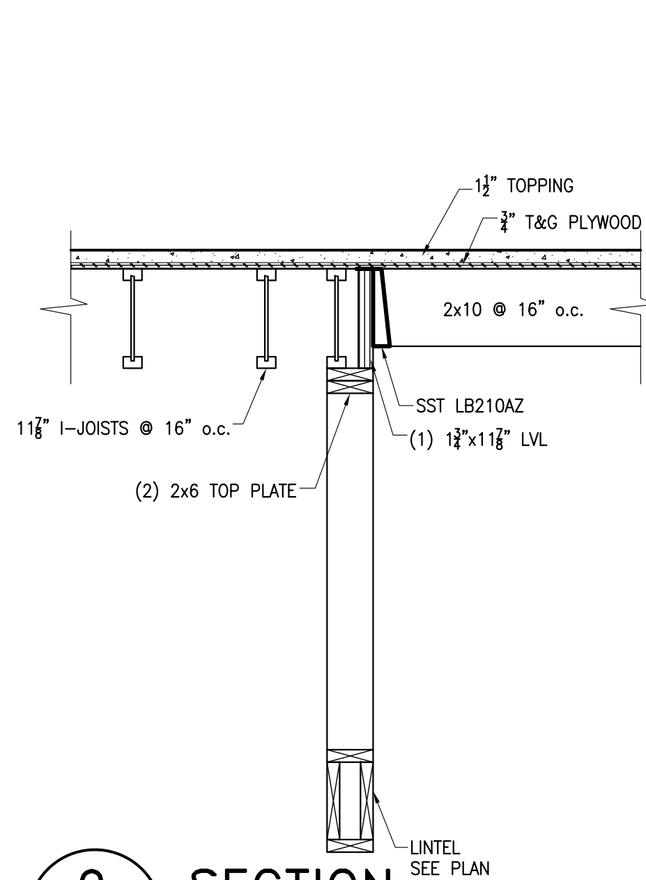
9 SECTION S501 3/4" = 1'-0"
