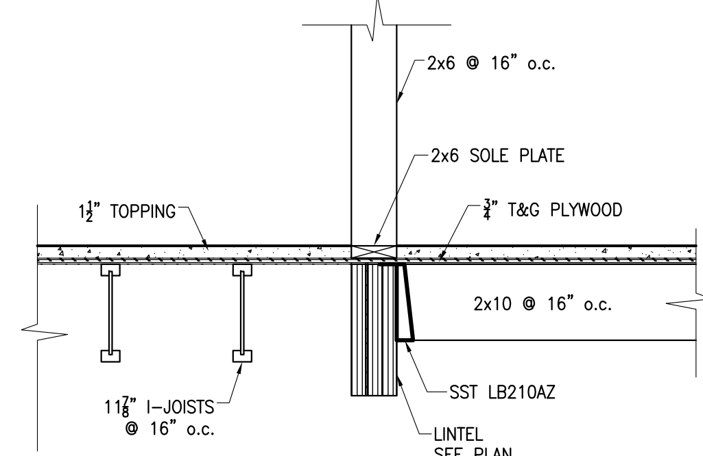
3 SECTION S501 3/4" = 1'-0"
