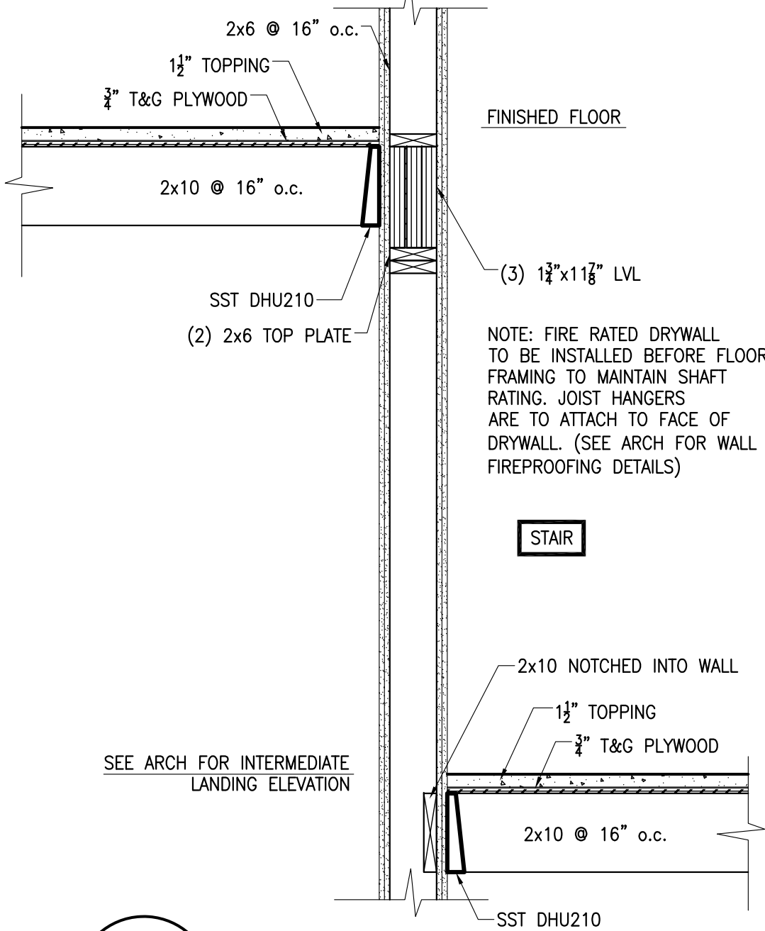
11 SECTION S501 3/4" = 1'-0"
