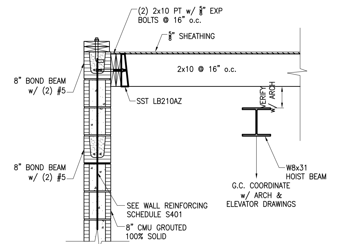
30 SECTION S502 3/4" = 1'-0"
