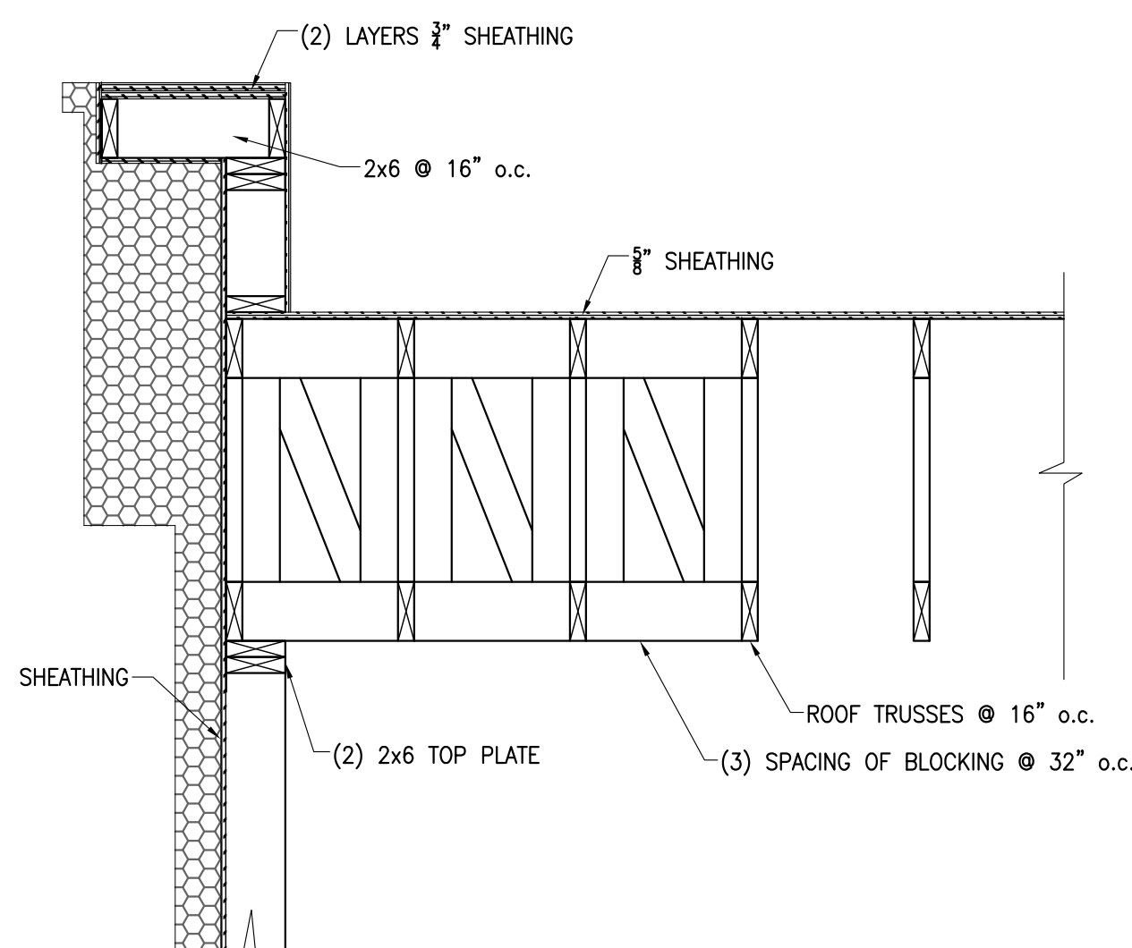
27 SECTION S502 3/4" = 1'-0"
