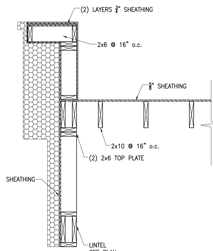
28 SECTION S502 3/4" = 1'-0"
