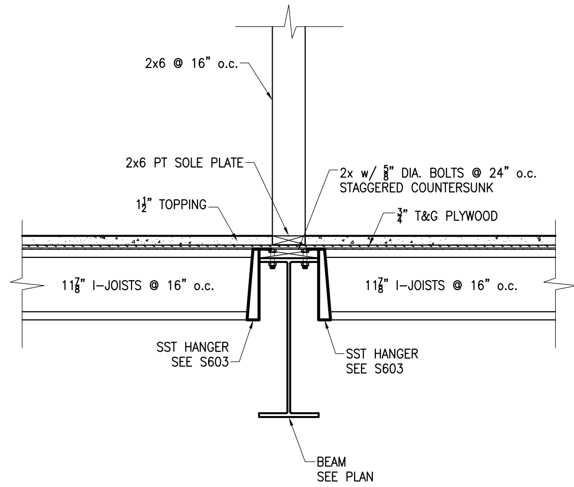
17 SECTION S502 3/4" = 1'-0"
