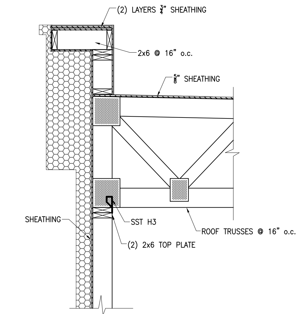
24 SECTION S502 3/4" = 1'-0"
