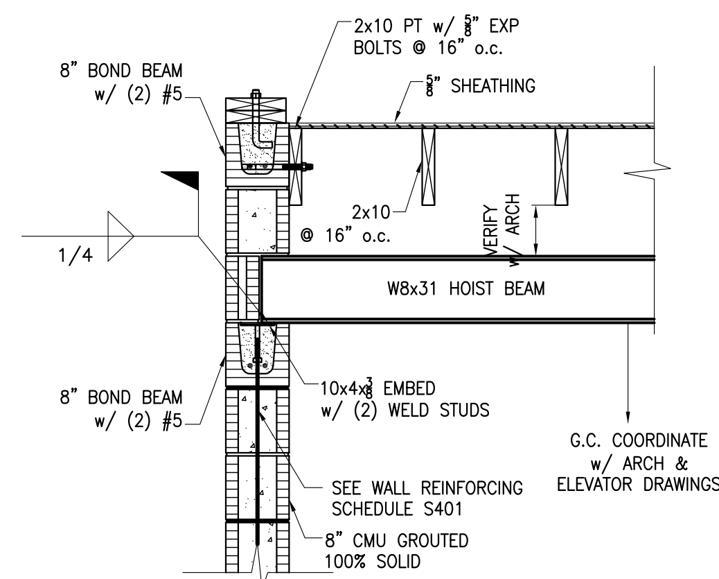
29 SECTION S502 3/4" = 1'-0"
