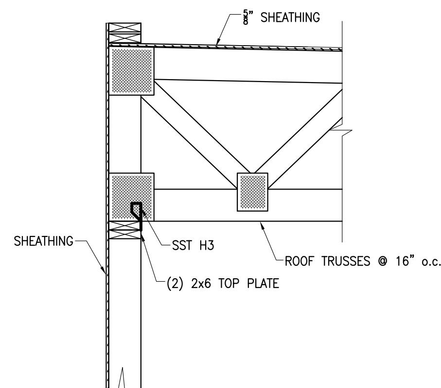
26 SECTION S502 3/4" = 1'-0"
