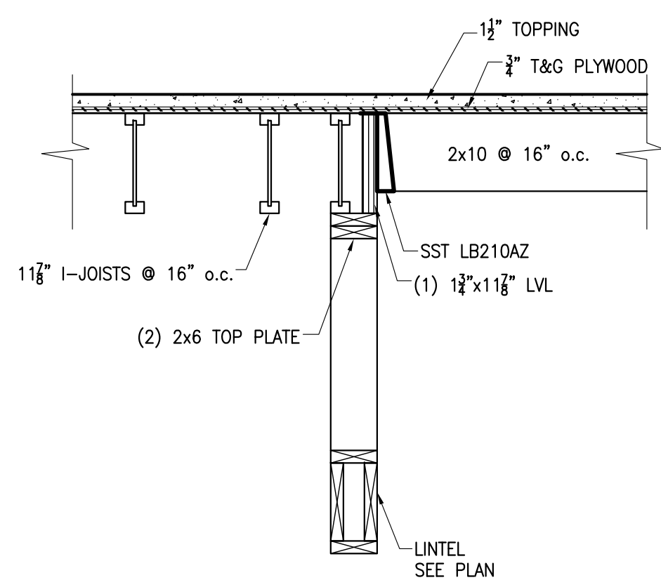
22 SECTION S502 3/4" = 1'-0"
