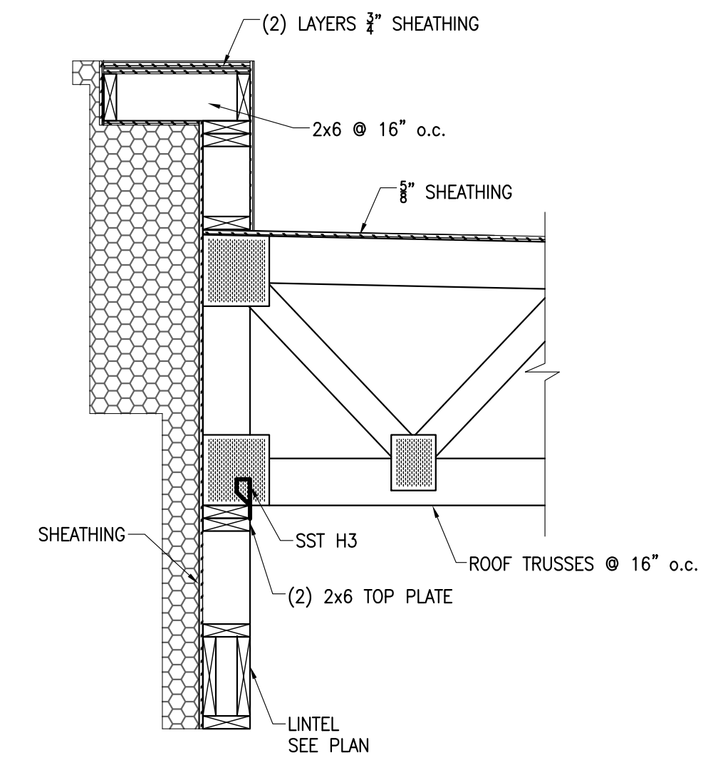
25 SECTION S502 3/4" = 1'-0"
