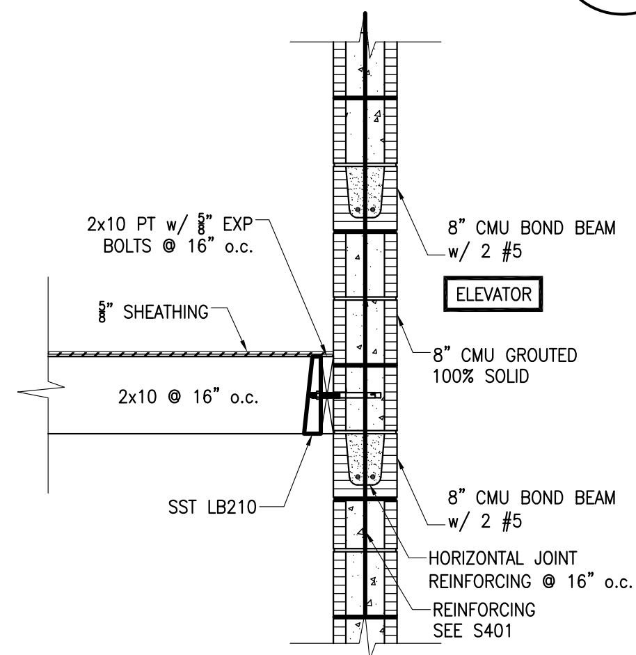
63 SECTION S506 3/4" = 1'-0"
