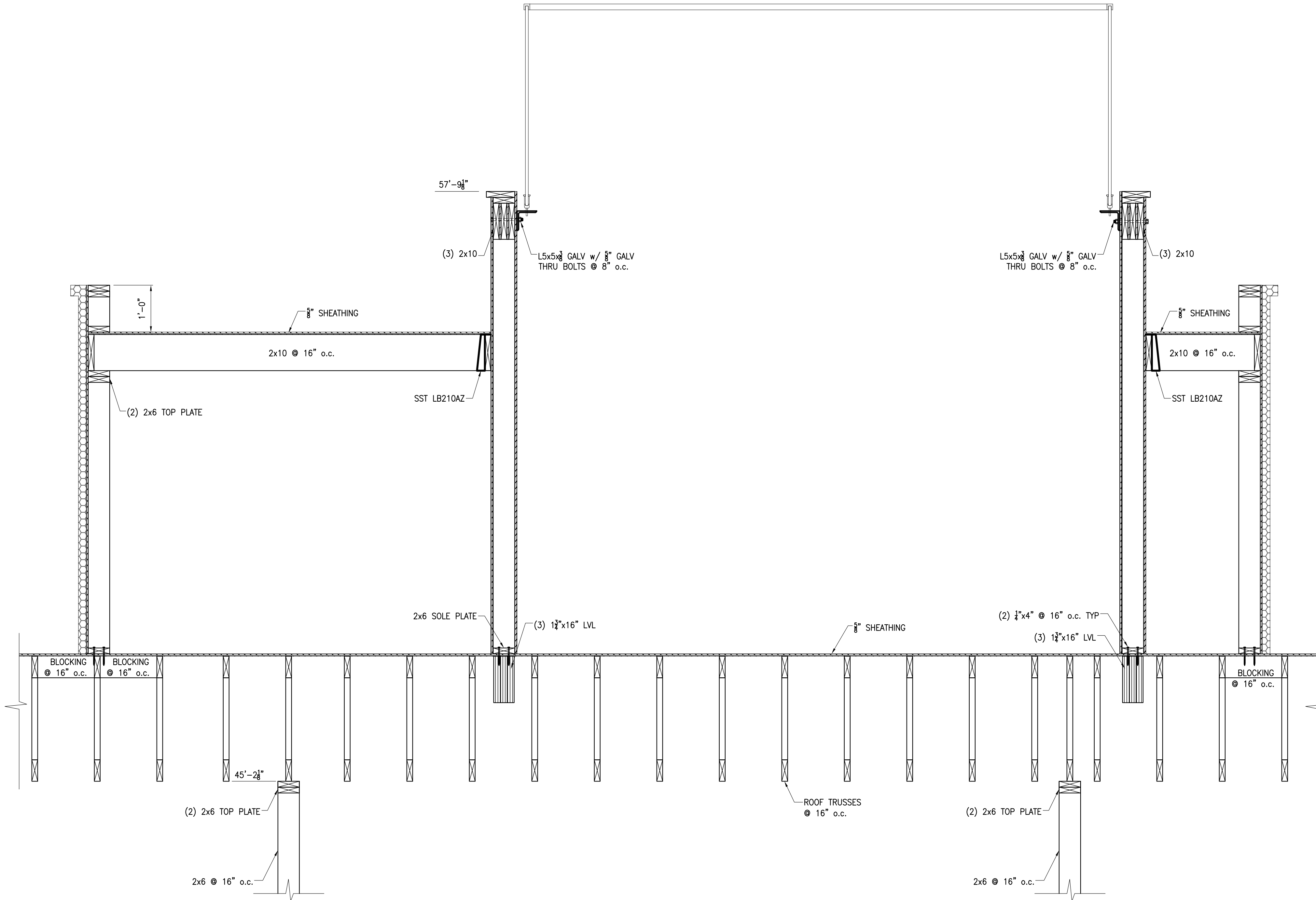
59 SECTION S506 3/4" = 1'-0"
