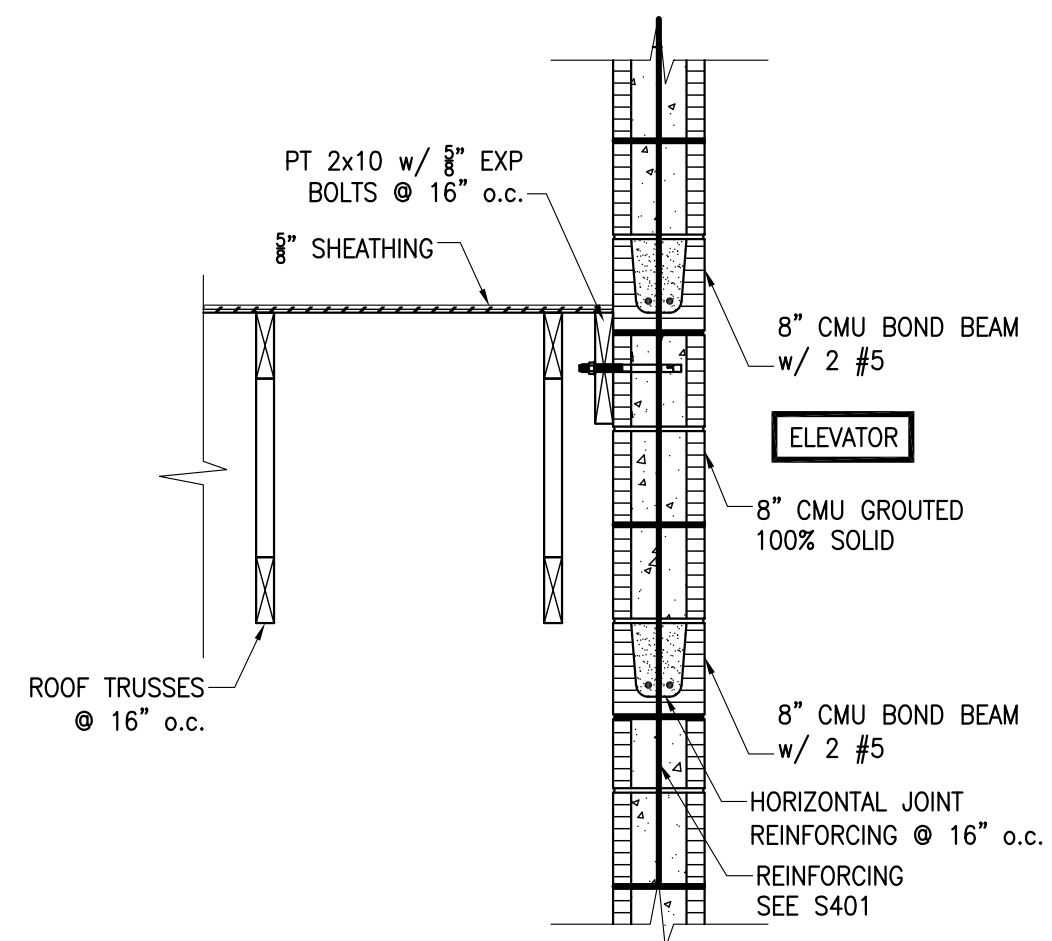
64 SECTION S506 3/4" = 1'-0"
