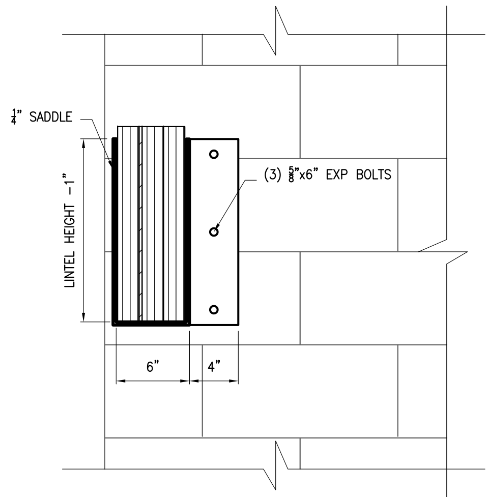
62 SECTION S506 1 1/2" = 1'-0"
