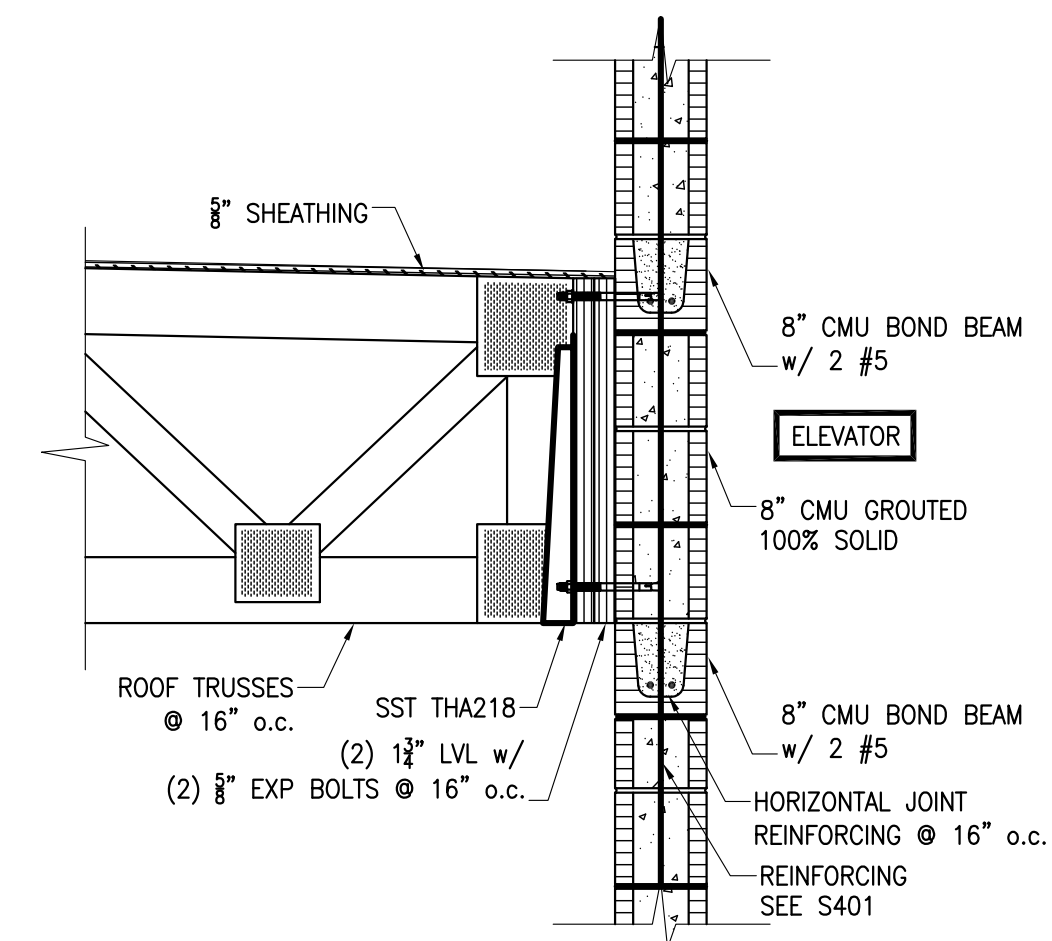
65 SECTION S506 3/4" = 1'-0"
