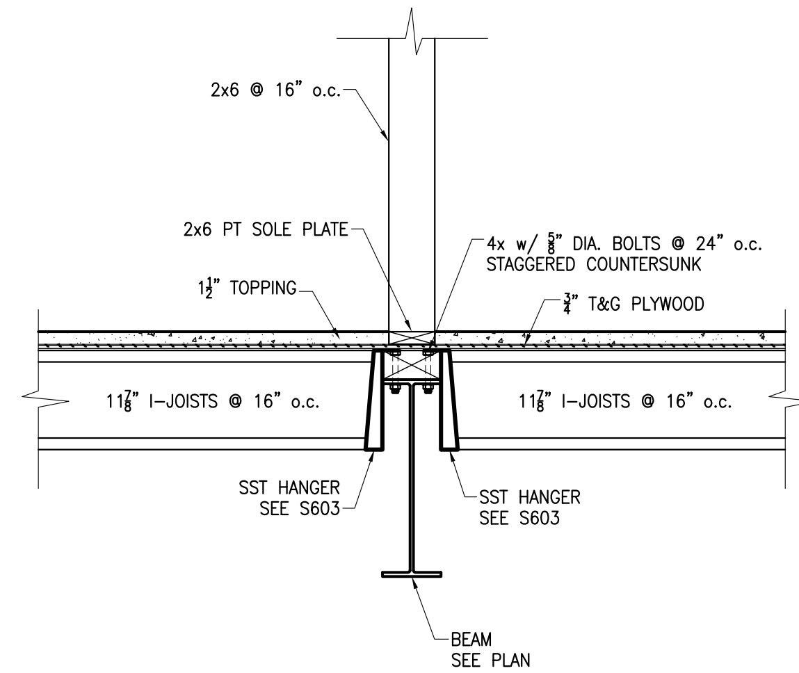
61 SECTION S506 3/4" = 1'-0"
