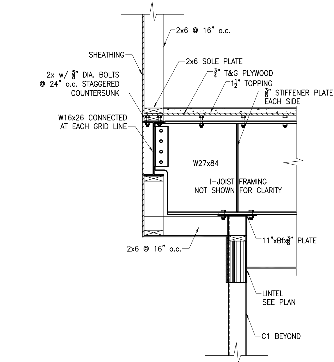
60 SECTION S506 3/4" = 1'-0"
