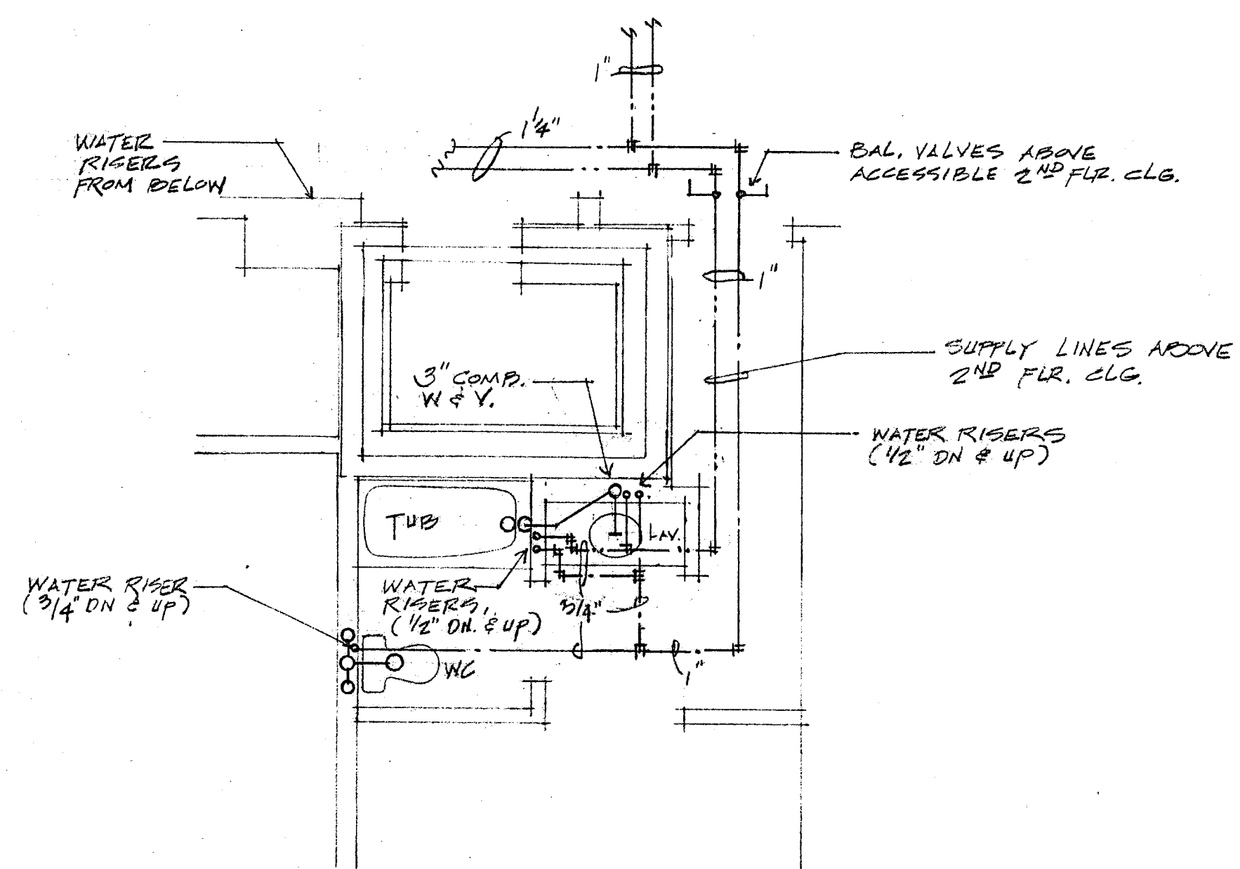
⑤ K2 BATHRM. PIPING
